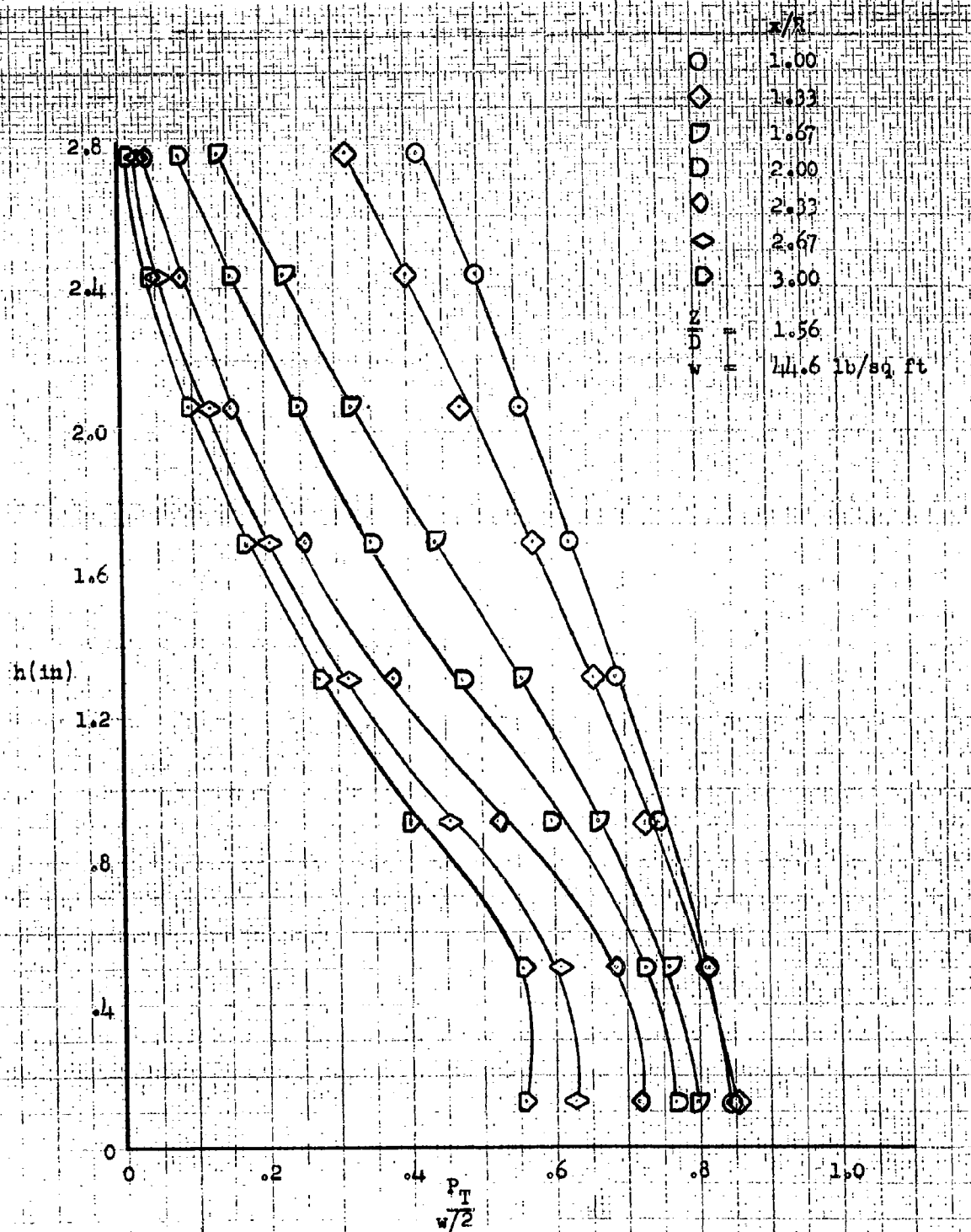
Figure 14 Side by Side Ducts Total Pressure Profiles \phi = 45^\circ
