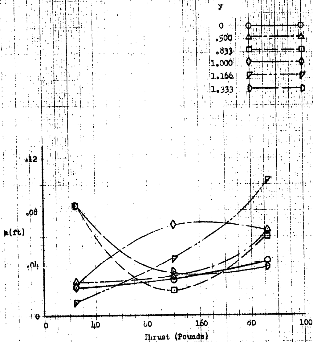
Figure 82 Wave Amplitude
