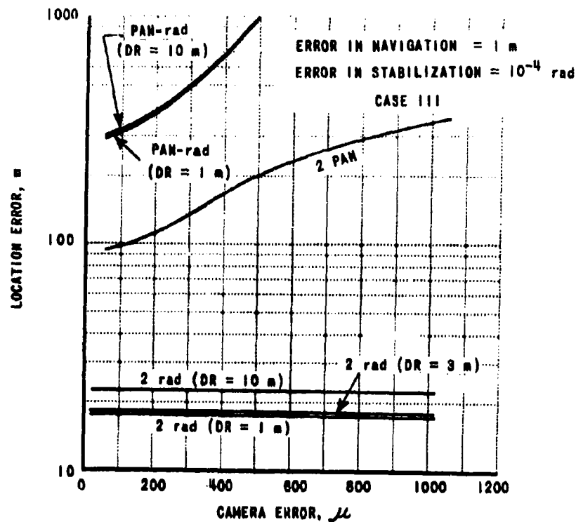
Figure 5.30 TARGET LOCATION ERROR
