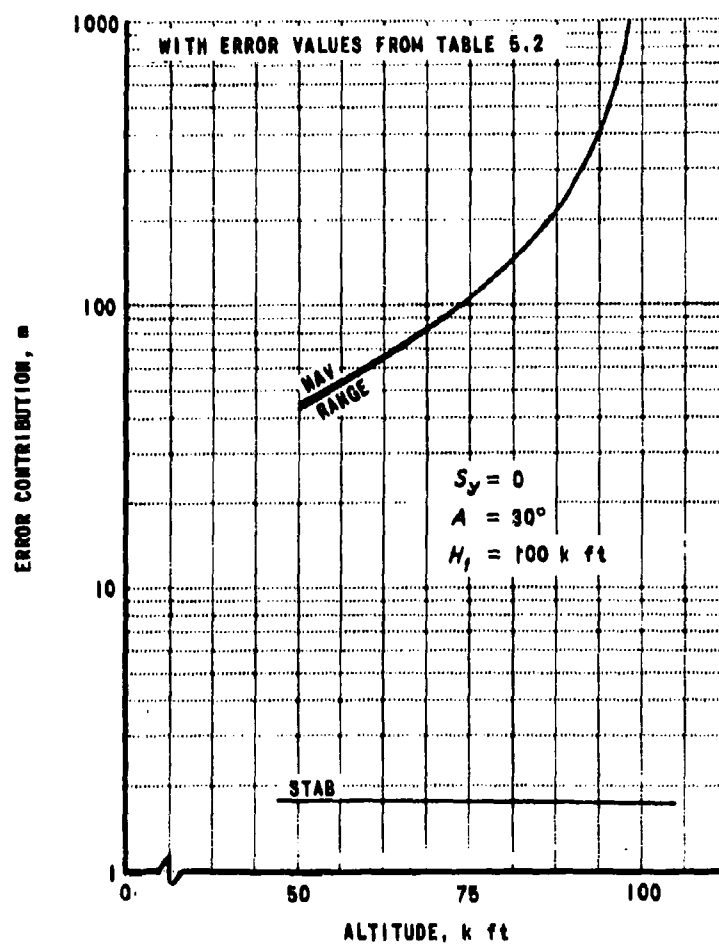
Figure 5.19 TWO-RAD SYSTEM - VARIATION WITH ALTITUDE OF SENSOR TWO
