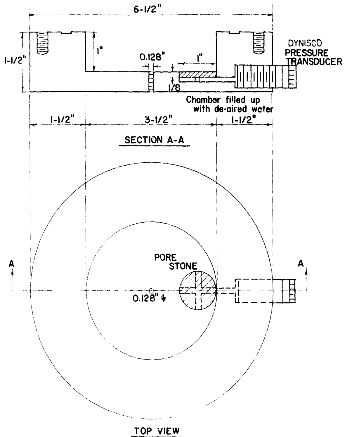
FIGURE 5.4 PORE PRESSURE MEASUREMENT SCHEME FOR DYNAMIC TESTS
