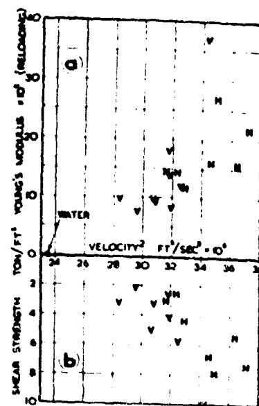
Correlation between the square of the wave velocity and (a) Young's modulus and (b) shear strength
