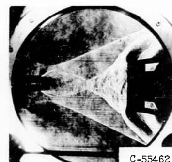
(9) D_1/D_2, 1.25 ; L/D_2, 2.164 ; p_b/p_0, 0.41 .
