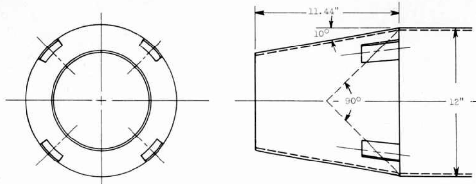
(a) Diameter ratio, D_1/D_2 , 1.5.
