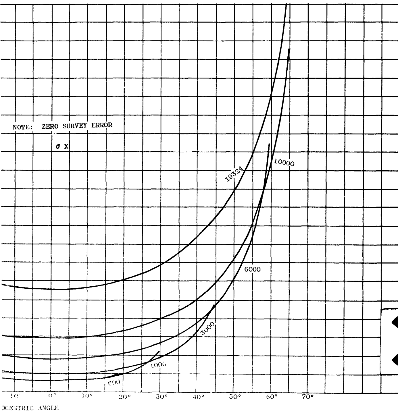
Figure 31. Standard Deviation in X Coordinate of Satellite Position vs. Geocentric Orbit Angle (Zero Survey Error)
