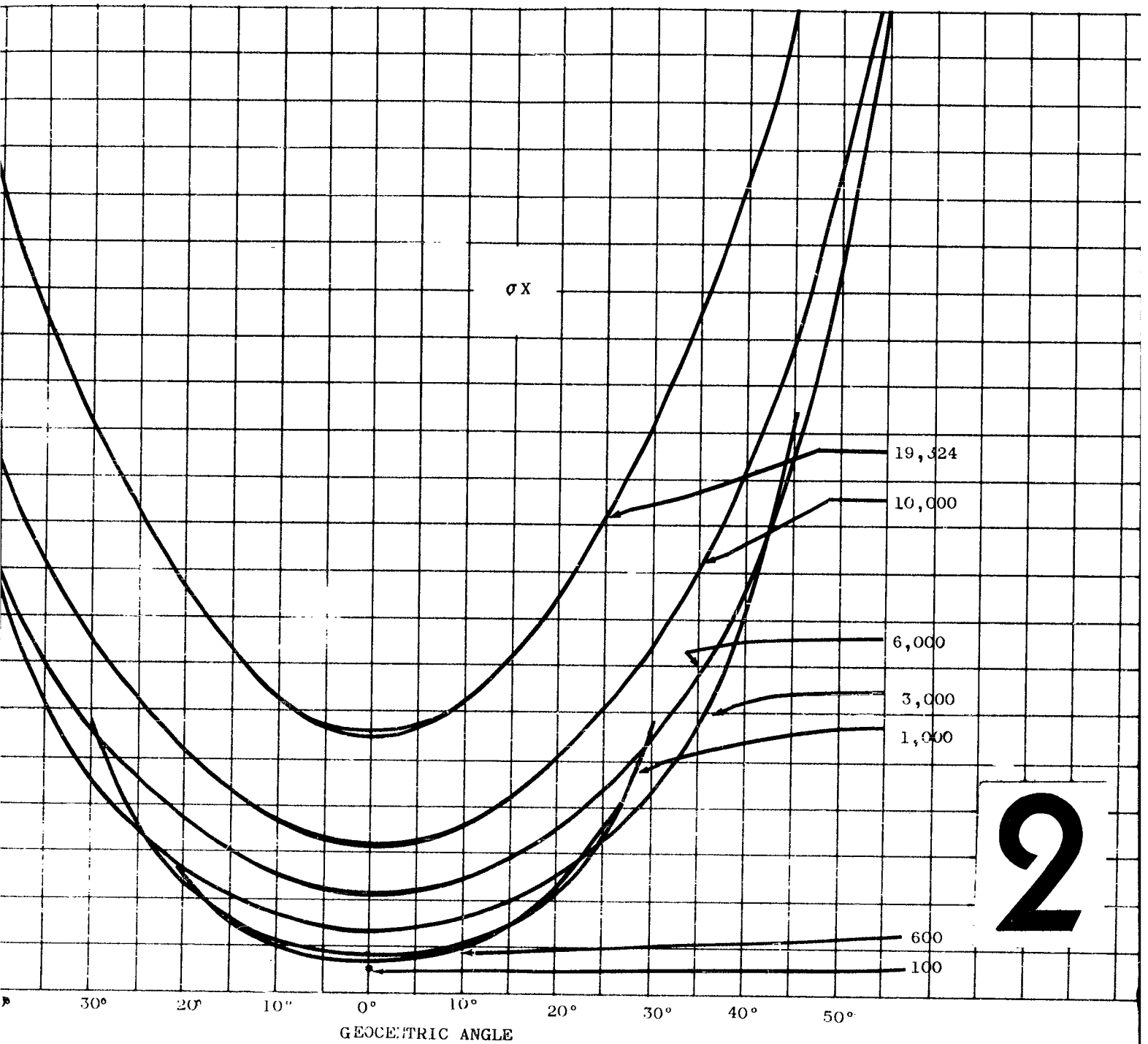
Figure 25. Standard Deviation in X Coordinate of Geocentric Orbit Angle
