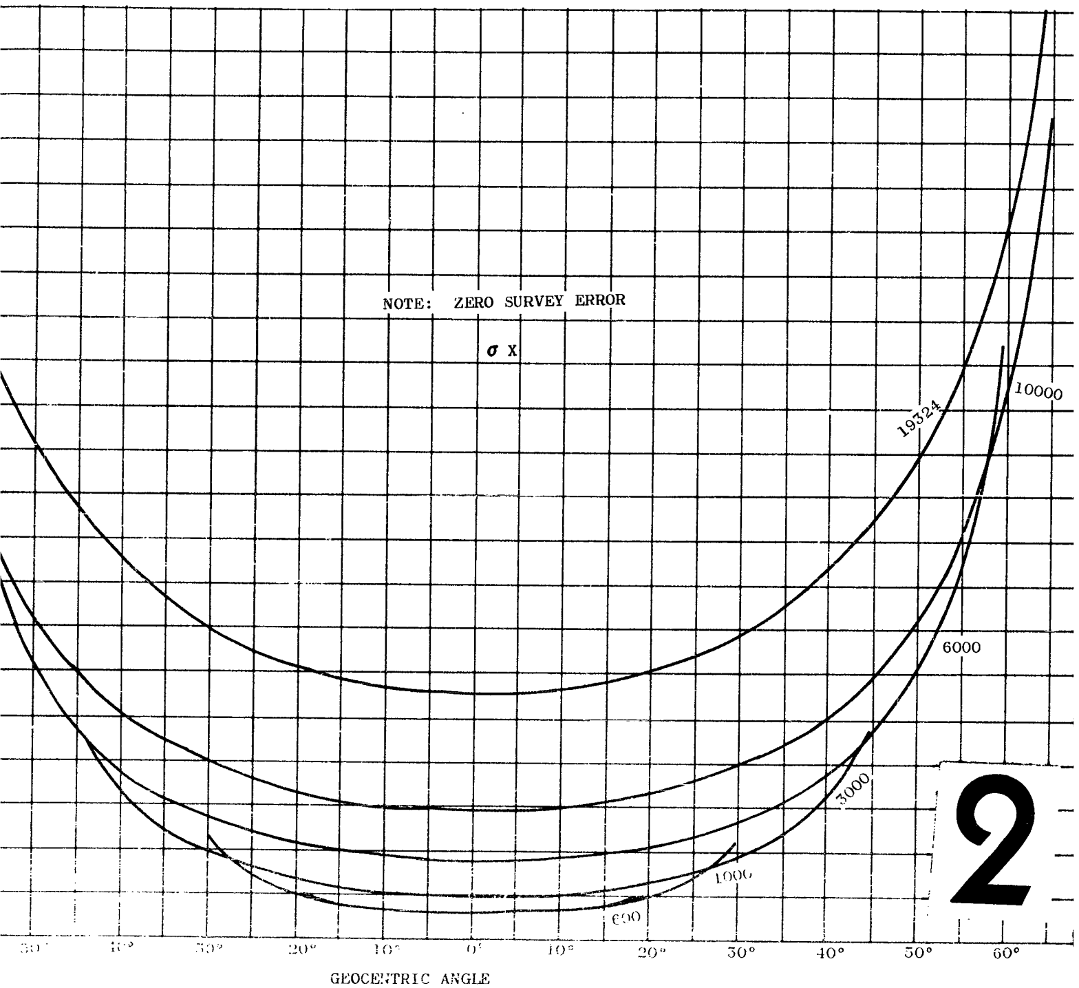
Figure 31. Standard Deviation in X Coordinate of S_z Geocentric Orbit Angle (Zero Survey
