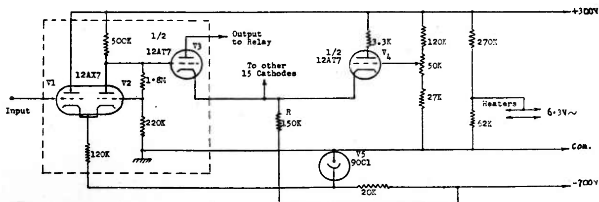
Fig. 16 (b) Maximum detector circuit. Detailed circuit diagram of one of 16 identical sections.
