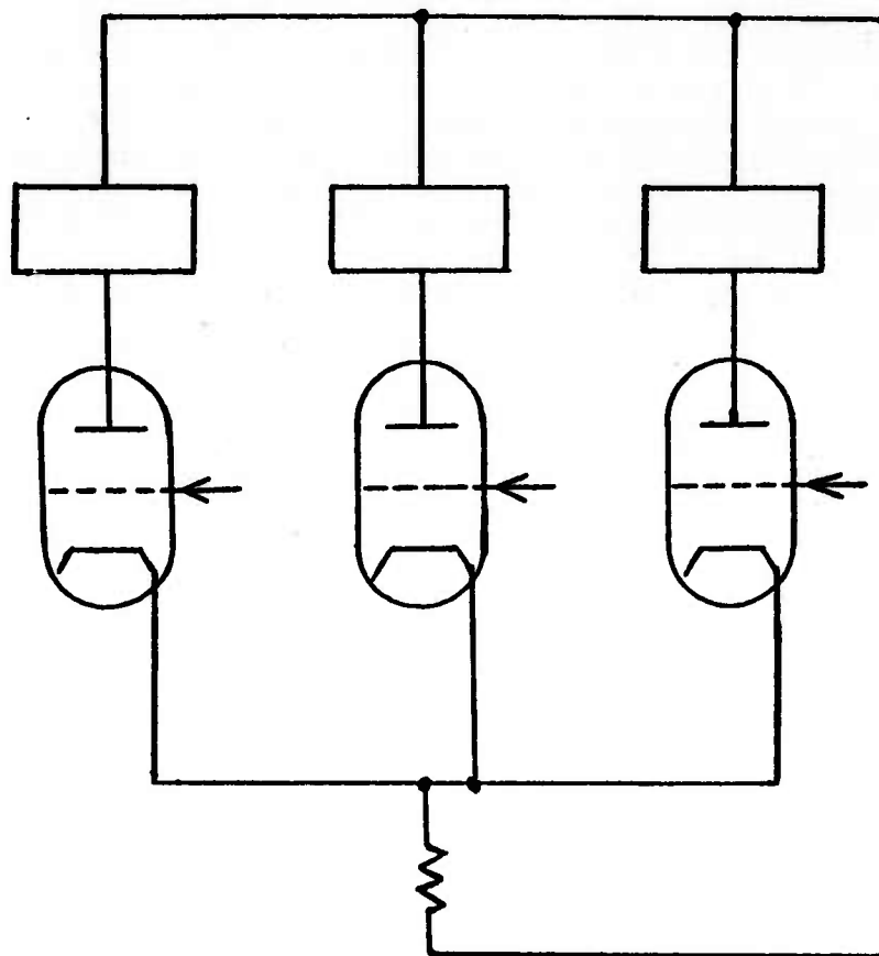
Fig. 16 (a). Maximum detector circuit. Simplified diagram.
