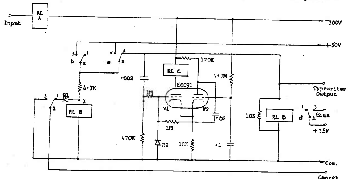
Fig. 22. Circuit diagram of a typical phoneme memory unit.
