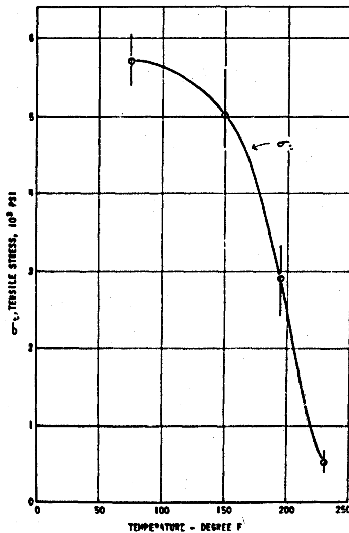
Fig. 10 - Maximum Tensile Stress vs. Temperature
