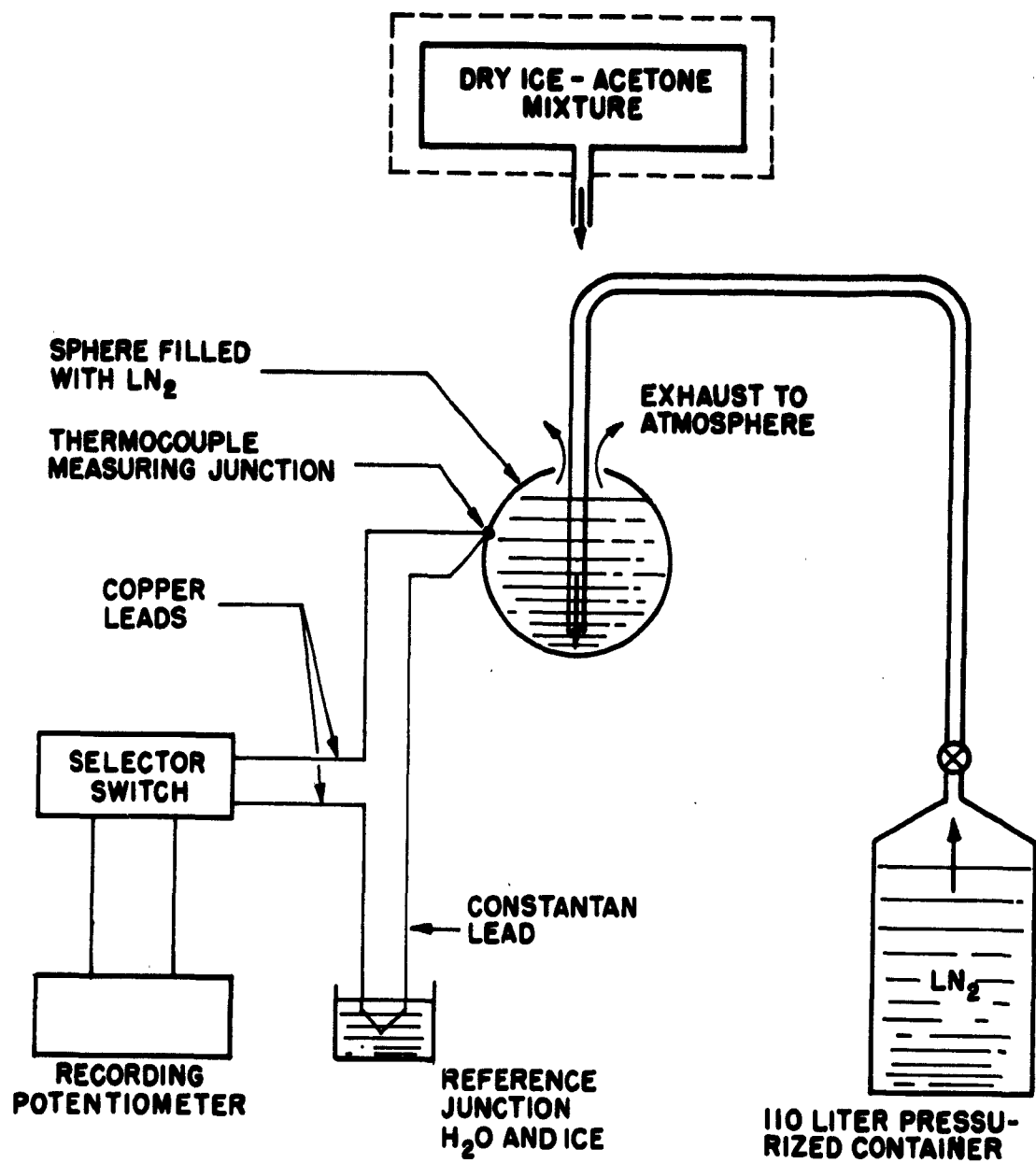
Figure 15. Schematic Diagram of Cooling Procedure and Thermocouple Circuit.
