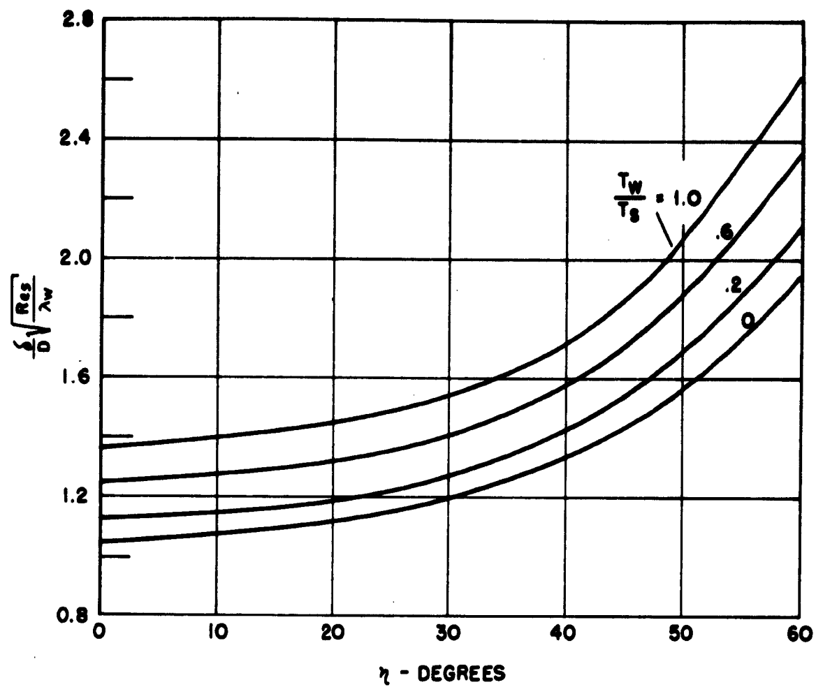
Figure 30. Variation of \delta with \eta and T_w/T_s on a Hemisphere in Hypersonic Flow.
