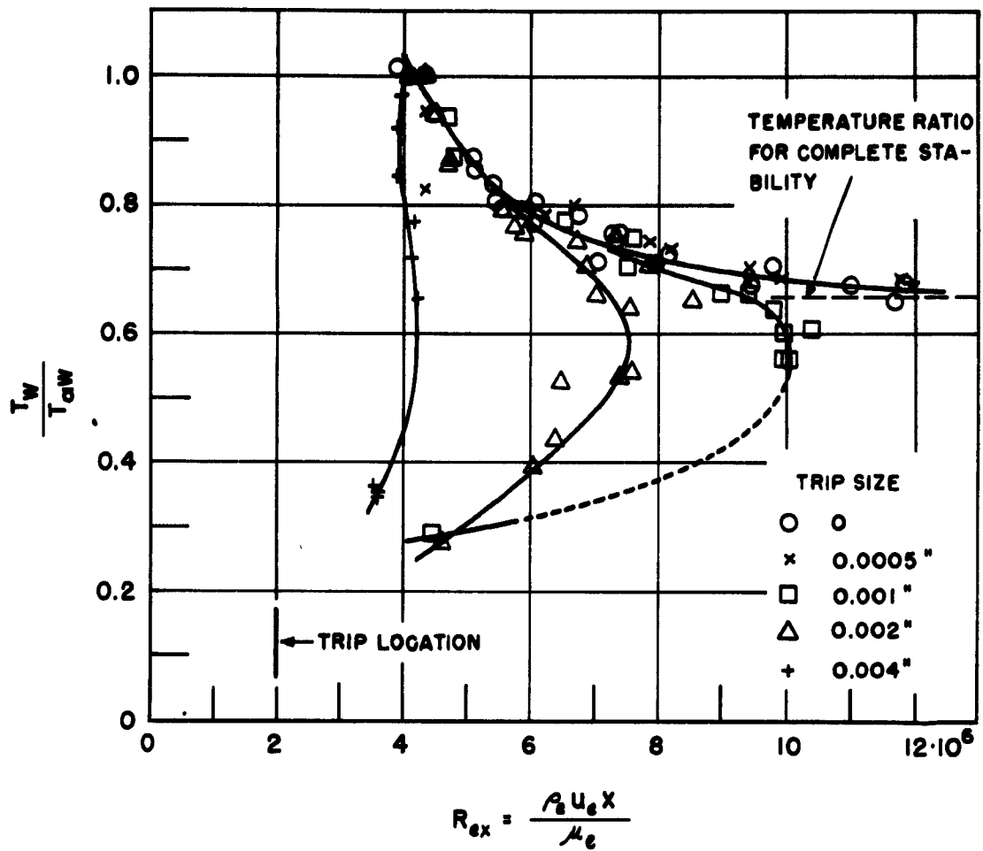
Figure 3. Effect of Cooling and Roughness on Transition on a Sharp 10^\circ Apex Angle cone at M_e = 2.70 (Data of van Driest and Boison(10)).
