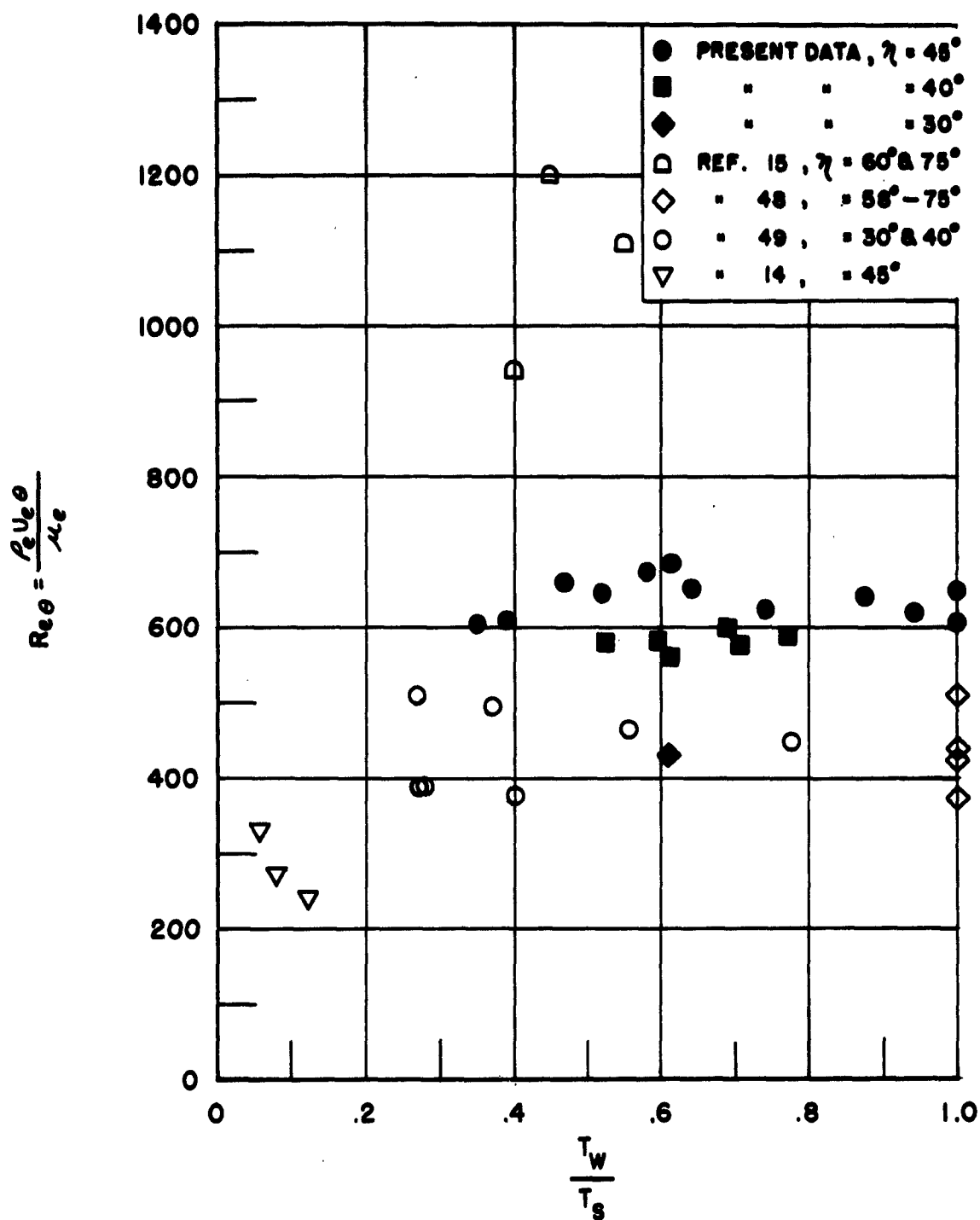
Figure 28. Local Transition Reynolds numbers Based on Boundary-Layer Momentum Thickness, Re_\theta , vs. T_w/T_s .
