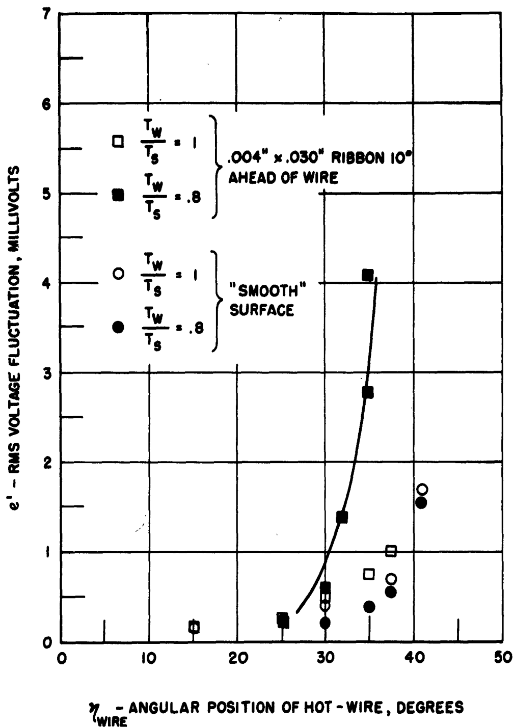
Figure 23. Hot Wire Fluctuation Distributions for T_W/T_S = 1.0 and 0.8 , (two-dimensional ribbons 10^\circ ahead of wire) (a) .004'' \times .030'' ribbon, and "smooth" surface.
