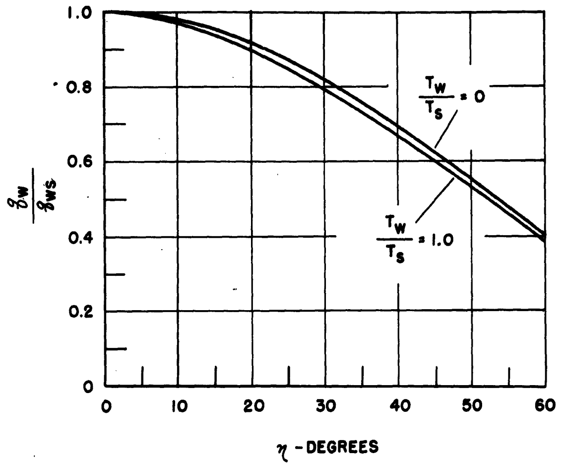
Figure 34. Variation of q_w with \eta and T_w/T_s on a Hemisphere in Hypersonic Flow.
