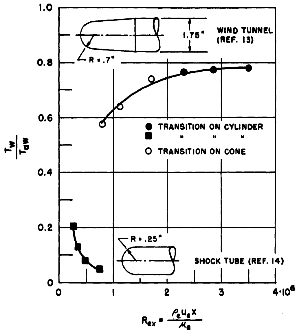
Figure 5. Effects of Cooling on Transition on Blunt Bodies (Data of Diaconis et al(13) and Stetson(14)).
