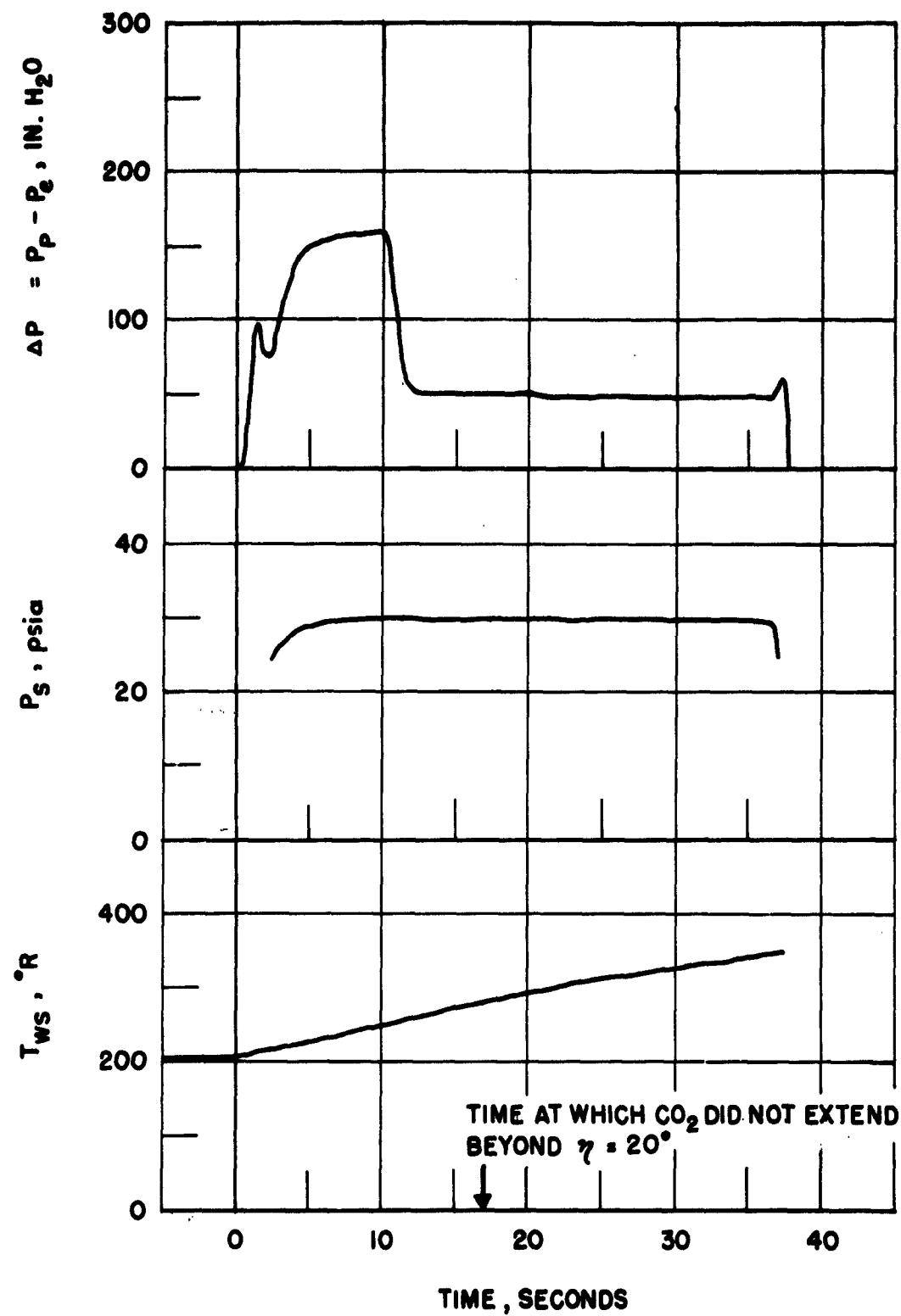
Figure 26. Correlation of Transition with \text{CO}_2 Film.
