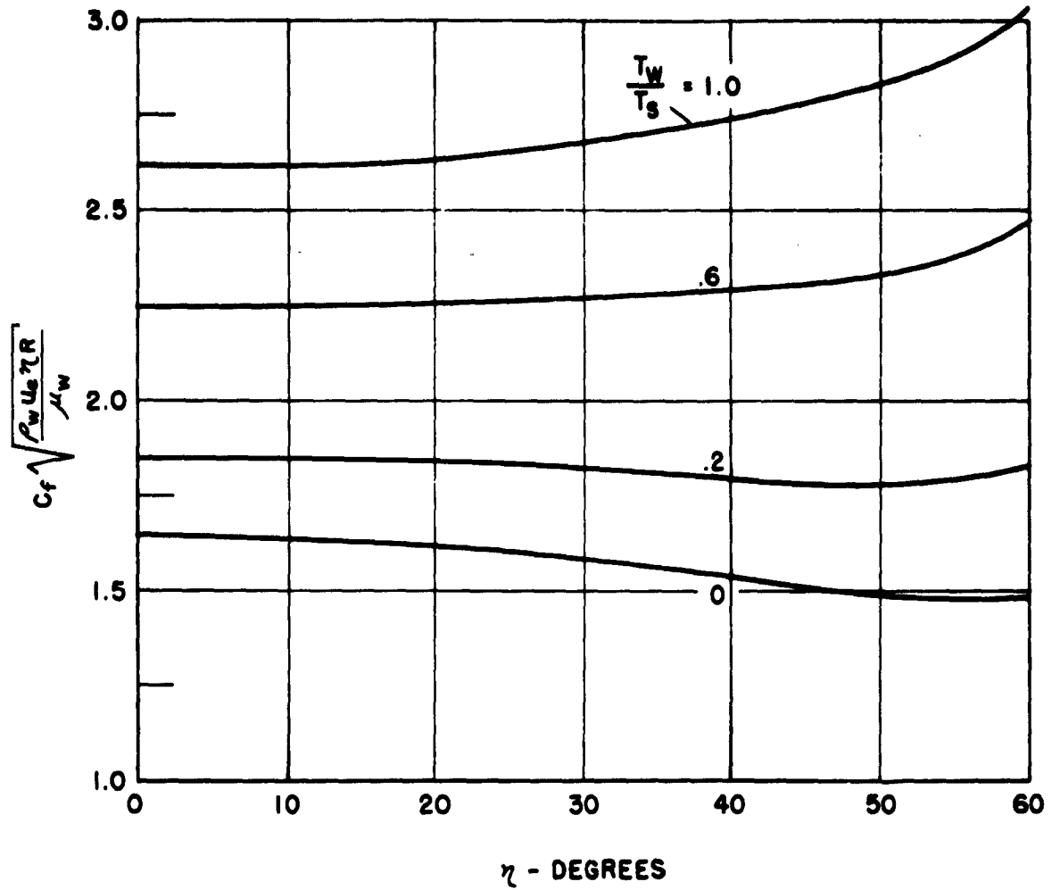
Figure 33. Variation of C_f \sqrt{\frac{\rho_w u_e \eta R}{\mu_w}} with \eta and T_w/T_s on a Hemisphere in Hypersonic Flow.
