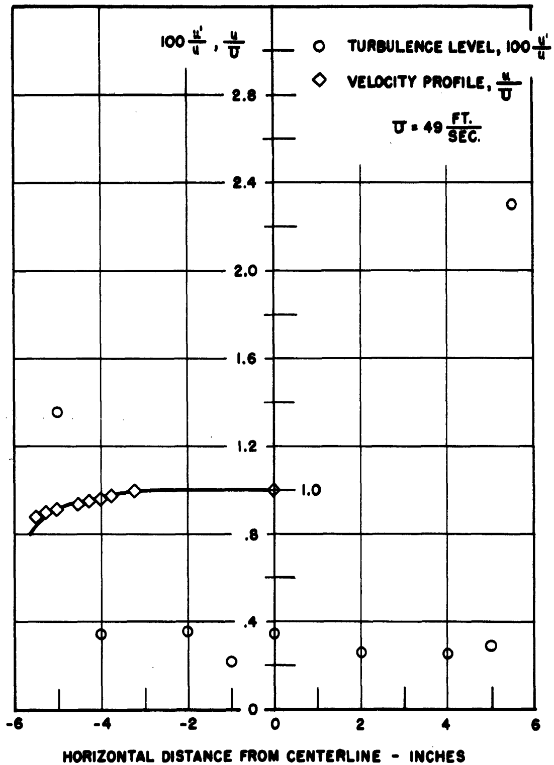
Figure 19. Turbulence Level and Velocity Distribution in the Settling Chamber.
