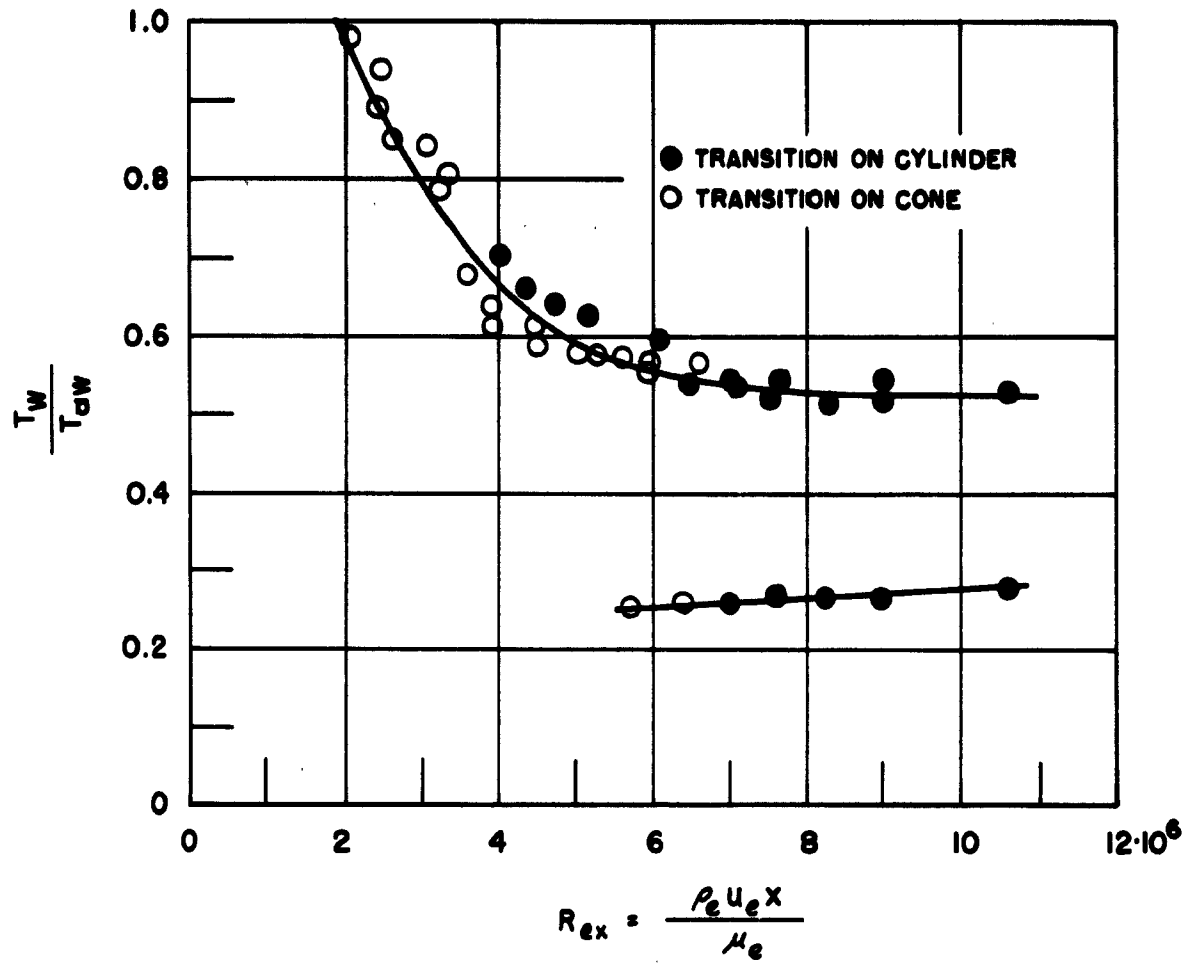
Figure 4. Effect of Cooling on Transition on a Sharp 9.5° Apex Angle Cone at M_{\infty} = 3.12 (Data of Jack et al(12))
