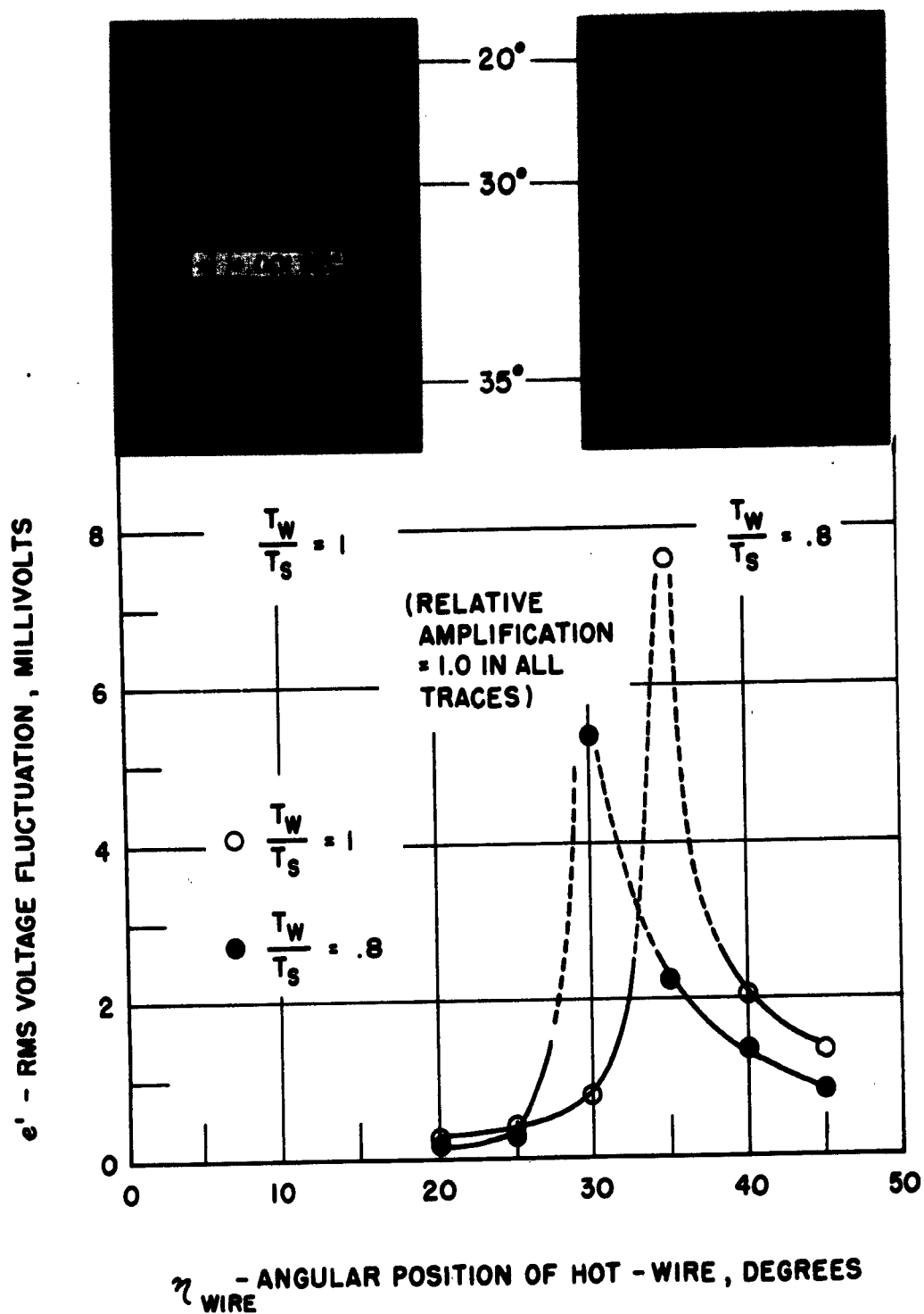
Figure 22. Hot Wire Fluctuation Distributions for T_W/T_S = 1.0 and 0.8 , (.004" x .025" Diameter Disk, 15° Ahead of Wire)
