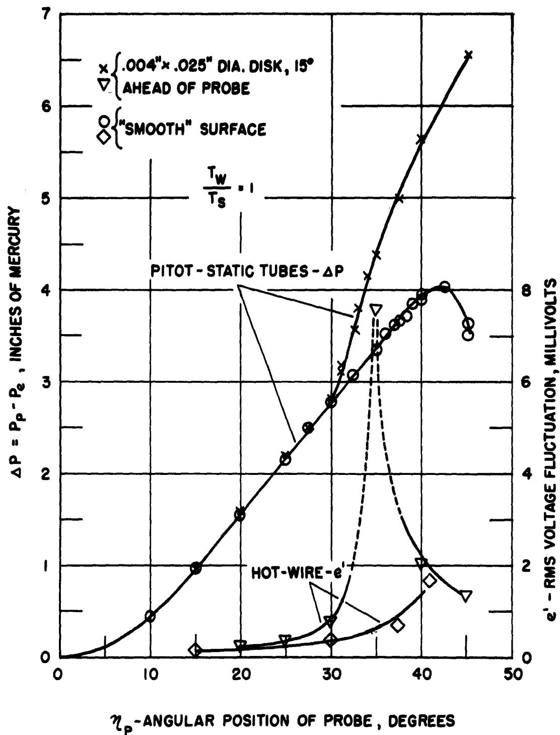
Figure 21. Hot-wire and Pitot Tube Measurements of Transition Caused by a .004" x .025" Diameter Disk.
