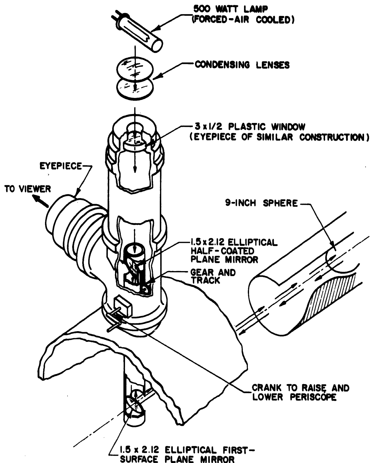
Figure 11. General Construction of Traveling Periscope.
