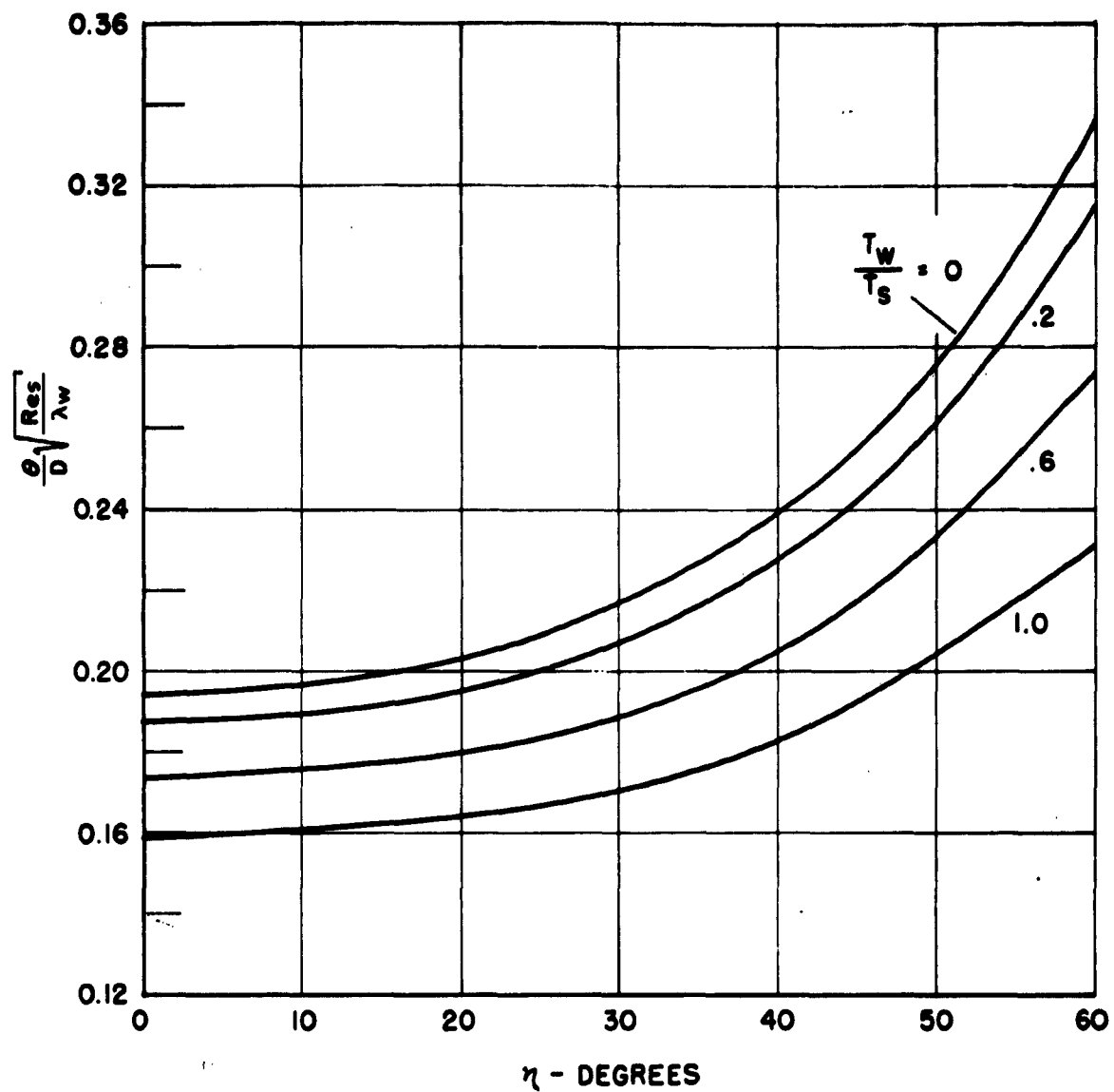
Figure 32. Variation of \theta with \eta and T_w/T_s on a Hemisphere in Hypersonic Flow.
