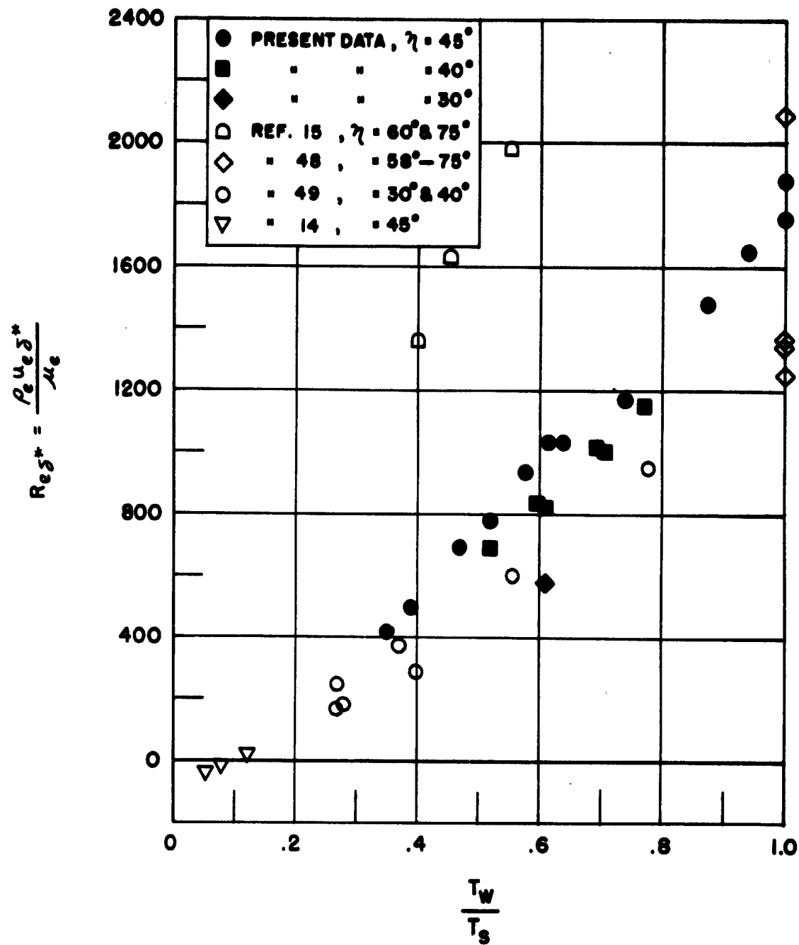
Figure 29. Local Transition Reynolds Number Based on Boundary-Layer Displacement Thickness, Re_{\delta^*} , vs. T_w/T_s .
