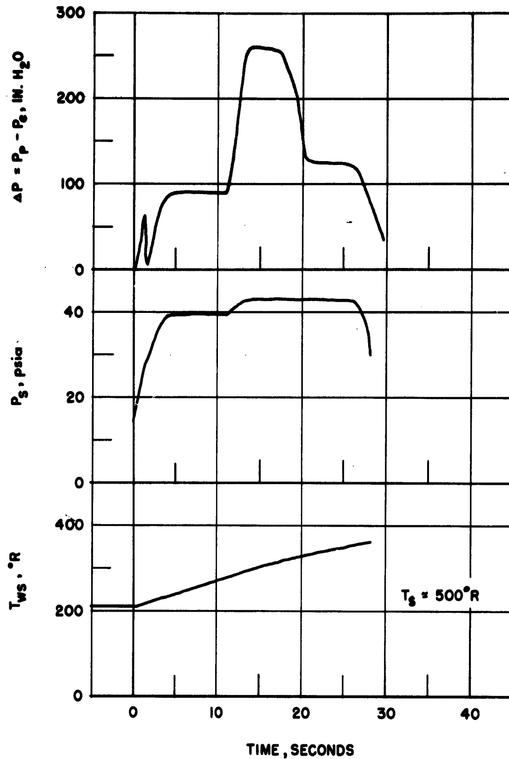
Figure 25. Records of P_p - P_s , P_s , and T_w During a Typical Transition Experiment.
