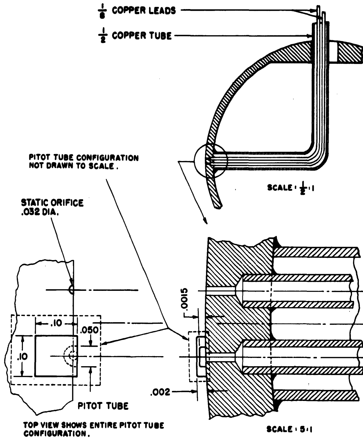
Figure 14. Size and Construction of Pitot and Static Pressure Probes.
