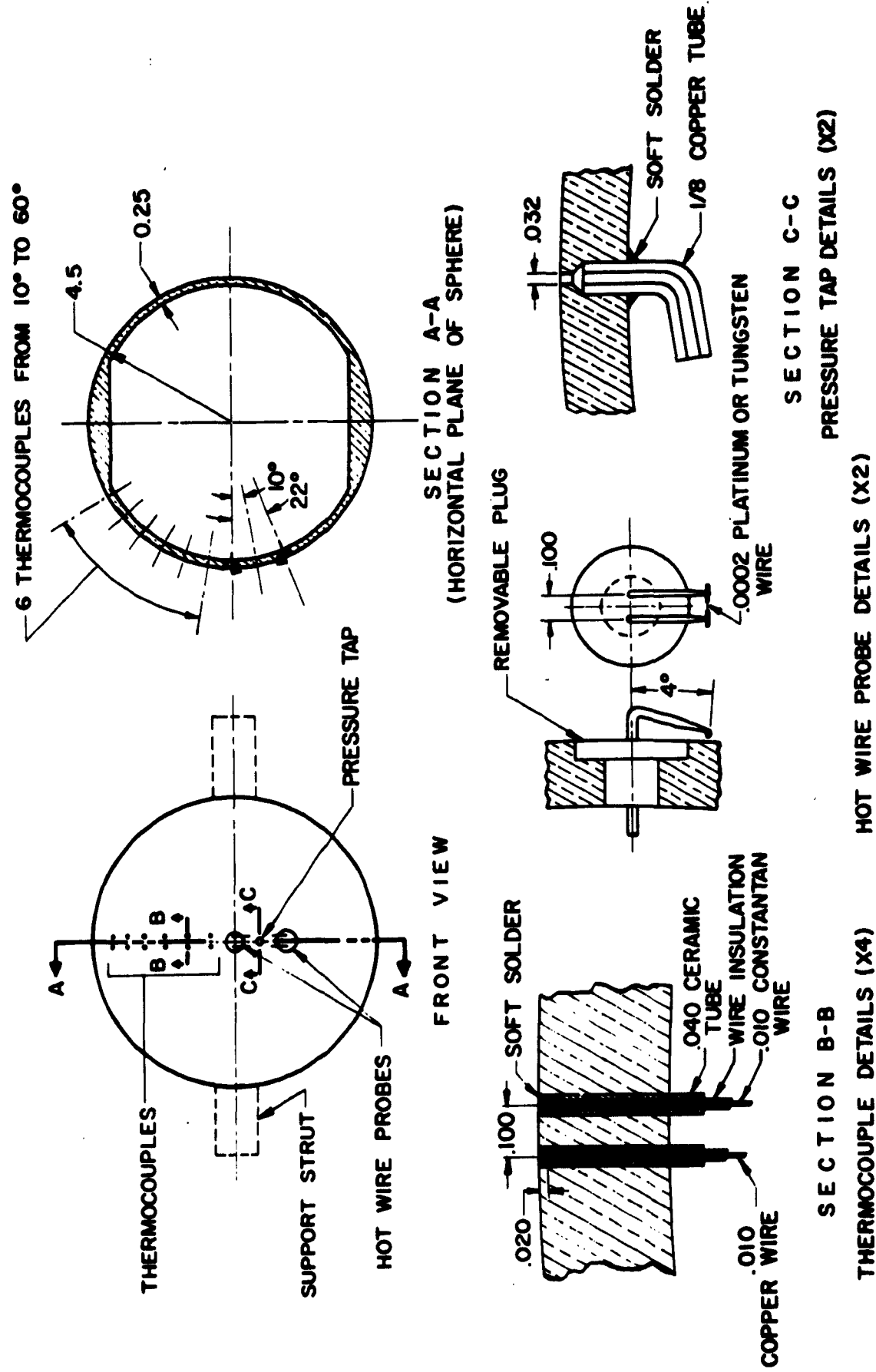
Figure 12. Details of Sphere Instrumentation. All Dimensions in inches.
