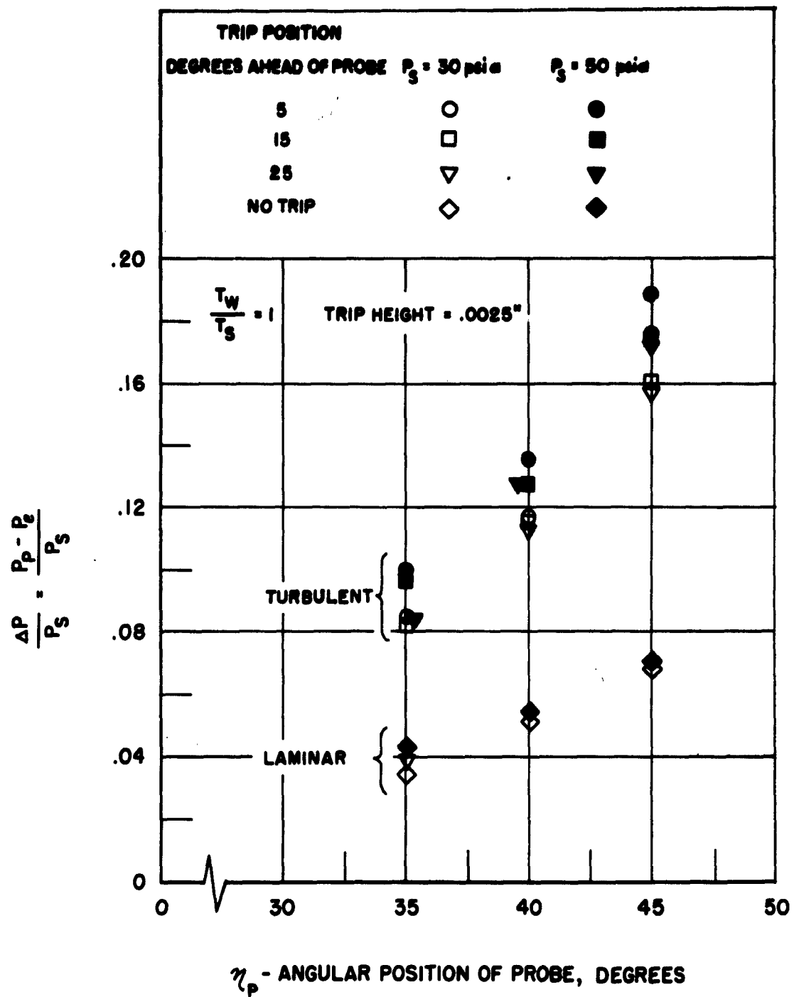
Figure 24. Calibration of Pitot Probe.
