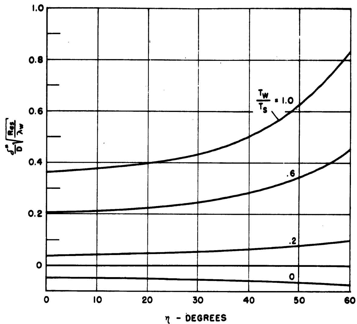
Figure 31. Variation of \delta^* with \eta and T_w/T_s on a Hemisphere in Hypersonic Flow.
