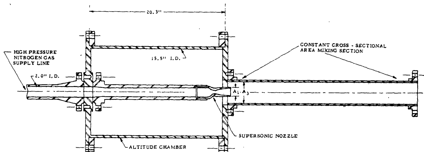
CONSTANT CROSS - SECTIONAL AREA SUPERSONIC DIFFUSER
