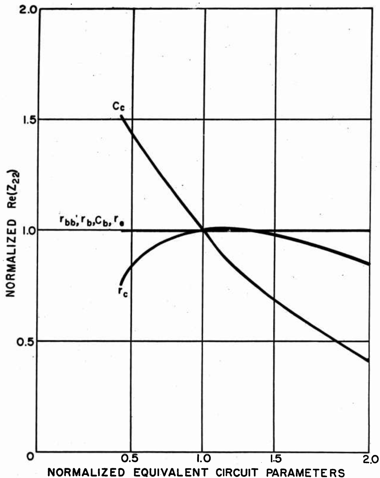
Figure 12. Real part of Z_{22} versus equivalent circuit parameters. Common emitter, collector, base configuration.
