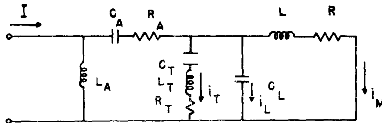
Figure 14. - Electrical analog circuit for abdomen-chest-mouth system. L_A is abdominal mass, C_A is elasticity of abdominal wall, diaphragm, etc., R_A is resistance associated with abdominal mass; C_T , L_T , R_T are elasticity, mass, resistance of thorax; C_L is elasticity of air volume of lungs; L , R are mass and resistance for air flow into and out of the lungs. I is excitation velocity of torso; i_T , i_L , i_M are velocities of wall of thorax, compression of lung and of air flow.
