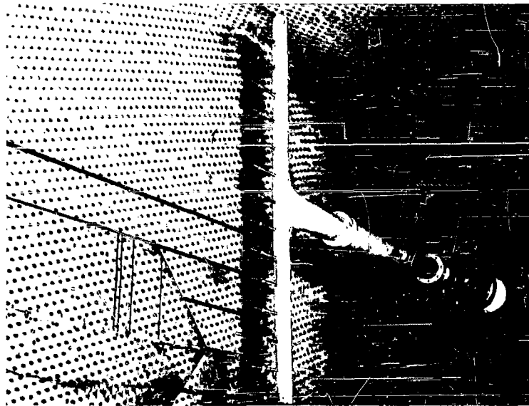
Fig. 9 Installation Photograph of the Wake Survey Rake
