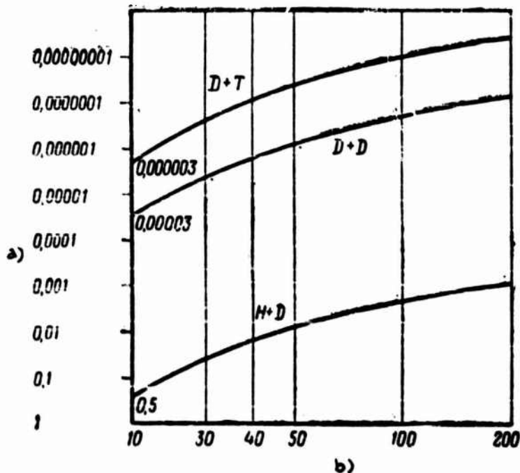
Fig. 14 - Relation between Duration of Several Nuclear Reactions and Temperature
