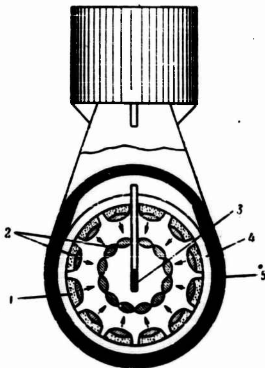
Fig.9 - Schematic Diagram of Atomic Bomb (Charged Divided into Several Parts):
