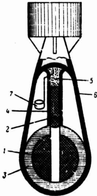
Fig.8 - Schematic Diagram of Atomic Bomb (Charge Divided into Two Parts):
