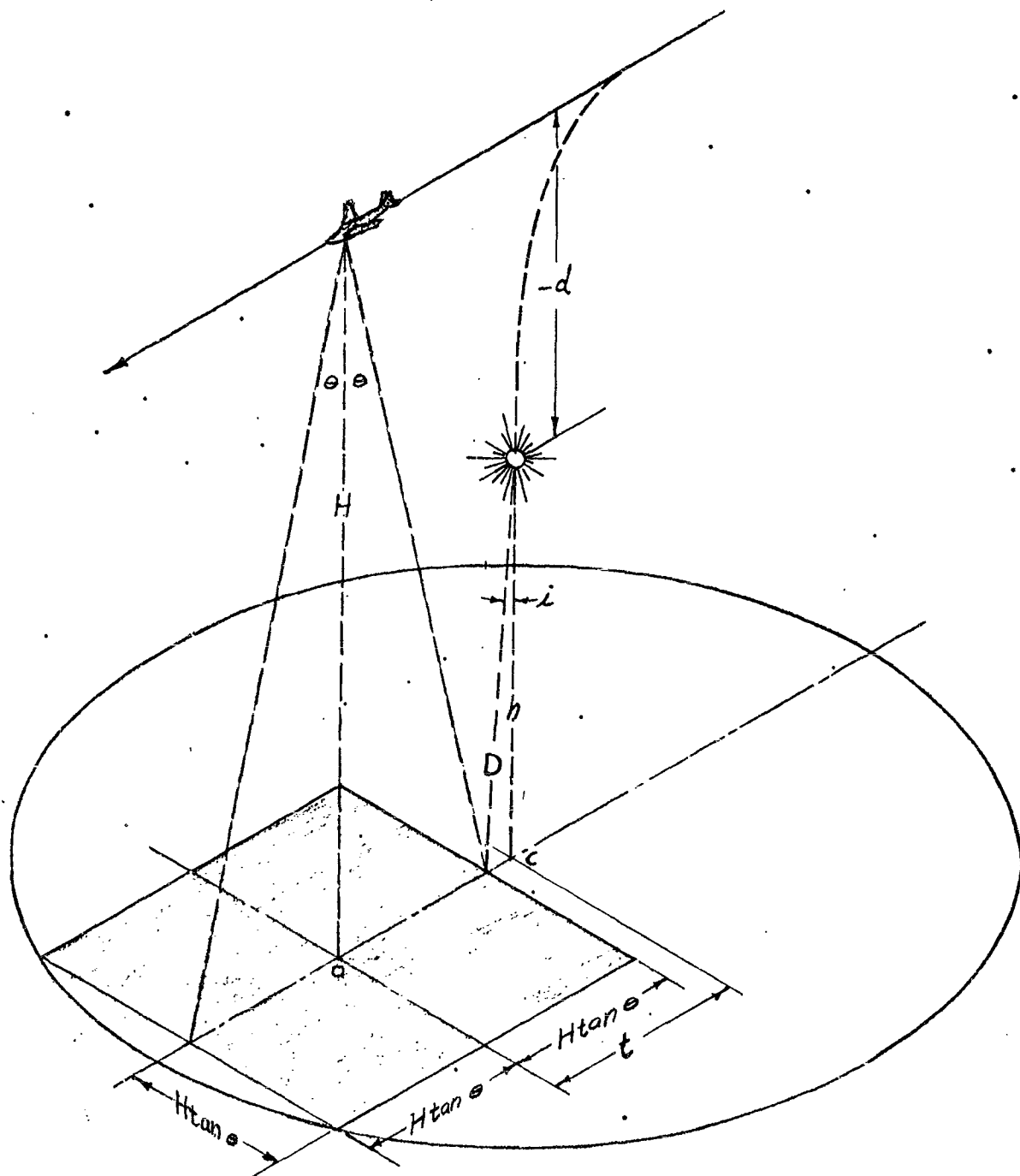
GEOMETRY OF FLIGHT LINE MAXIMUM SCENE ILLUMINATION BURST POINT NADIR OUTSIDE FIELD OF VIEW
