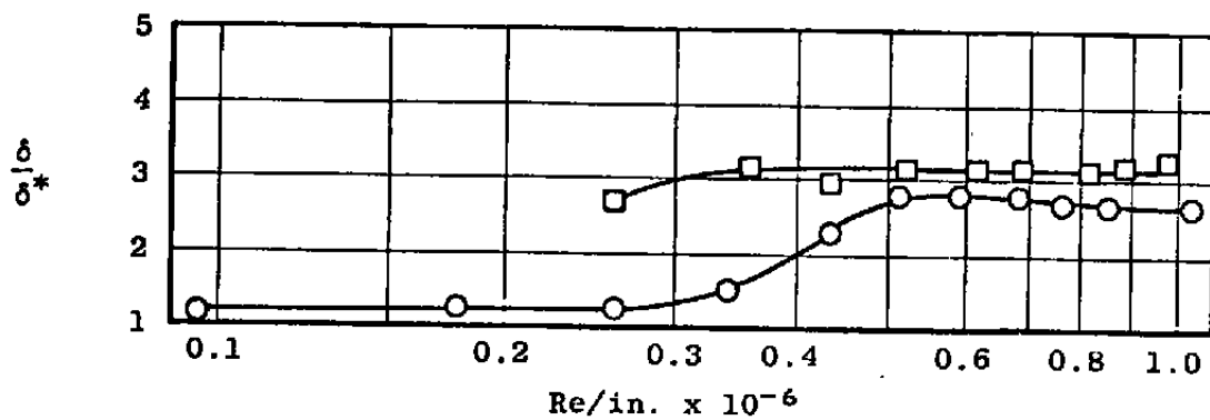
Fig. 7 Influence of Suction Slots on the Boundary-Layer Characteristics at Model Station 18.8 in.
