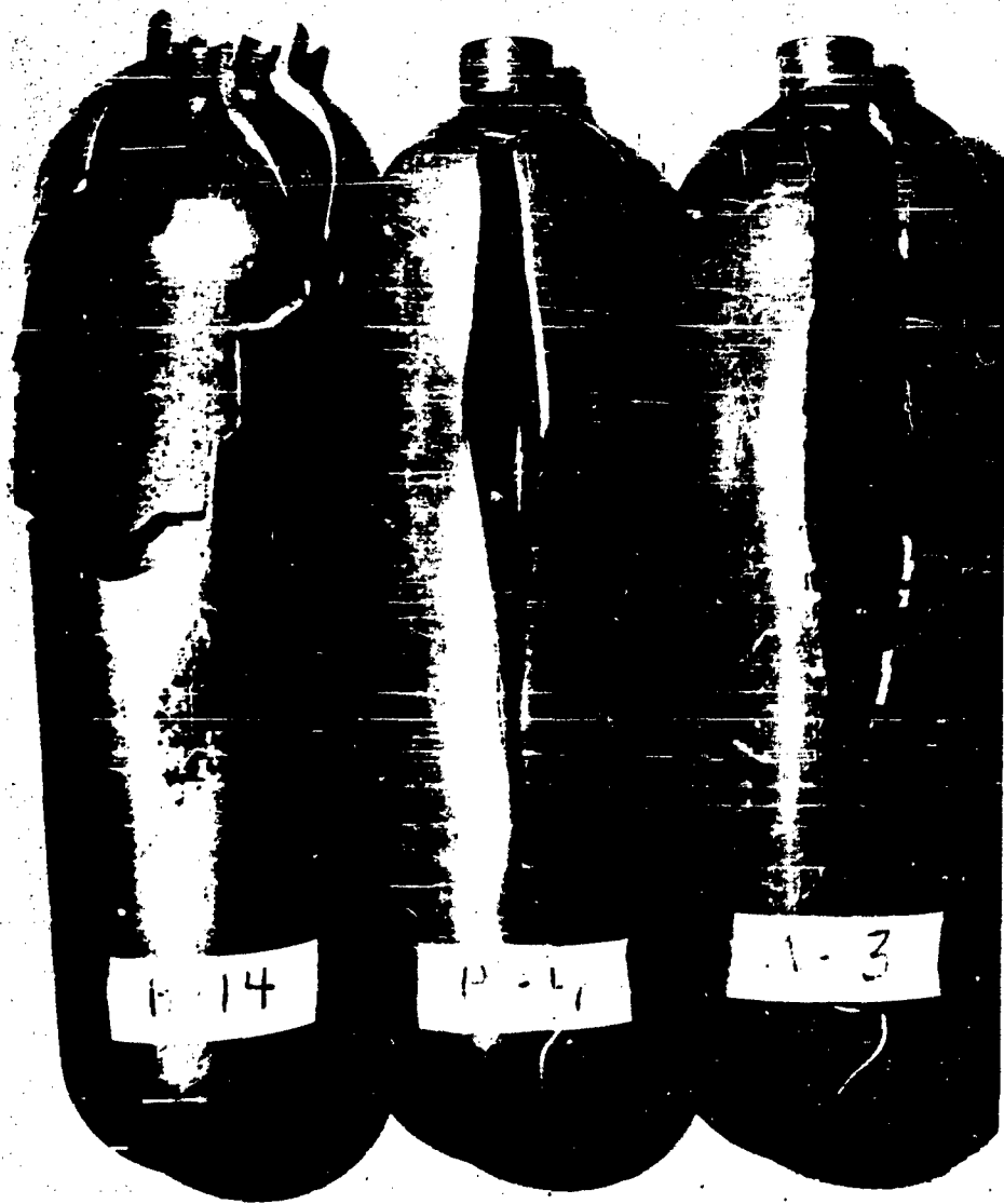
Figure 27. Typical vessels of AISI 4340 steel (240,000-262,000 psi nominal strength level) fractured at -105^{\circ}\text{F} .
