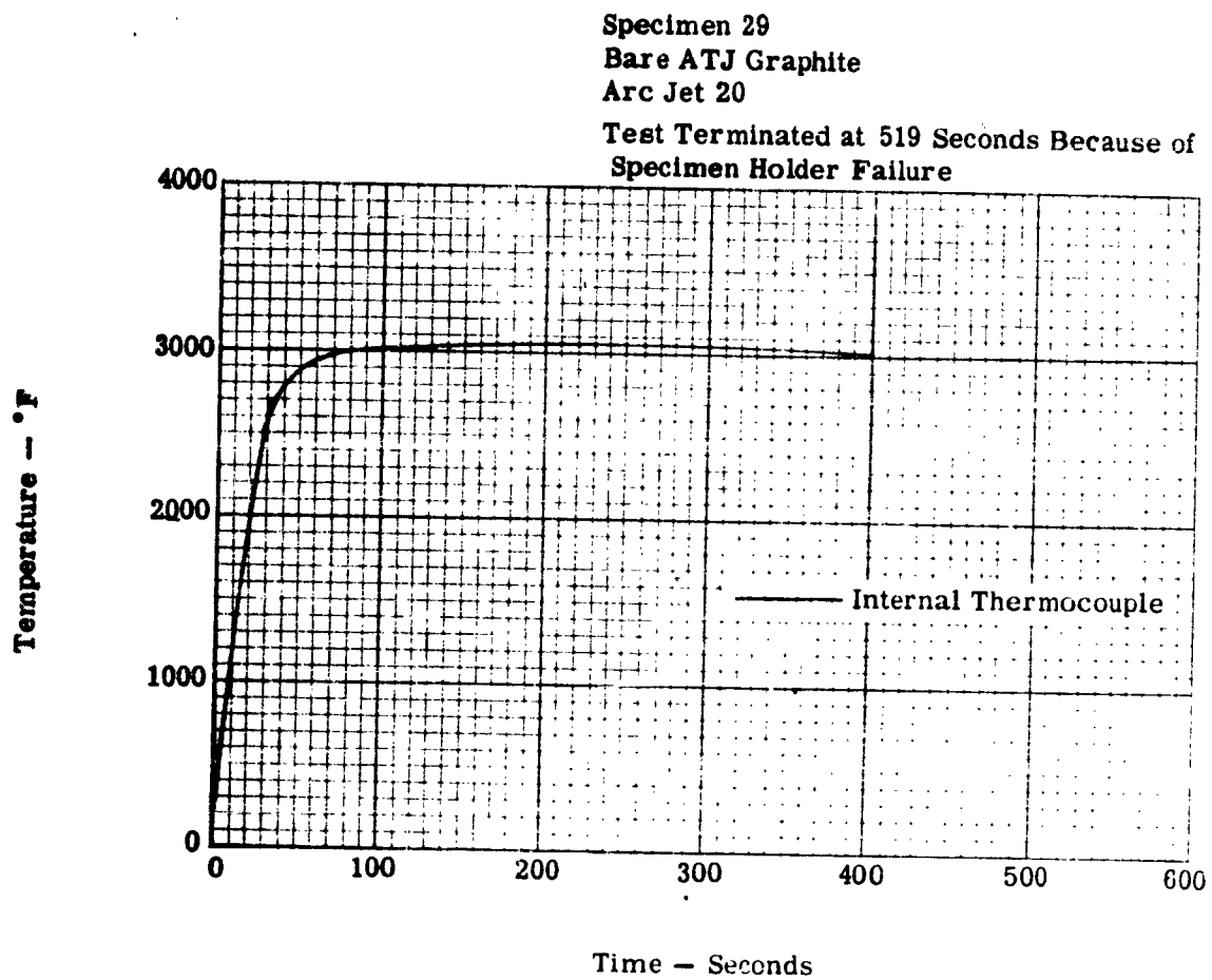
FIGURE 61. SPECIMEN 29 TEMPERATURE VS TIME, NASA LANGLEY RESEARCH CENTER.
