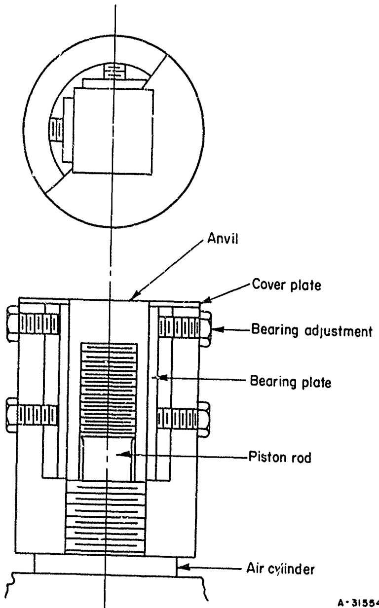
FIGURE 1. ANVIL ASSEMBLY
