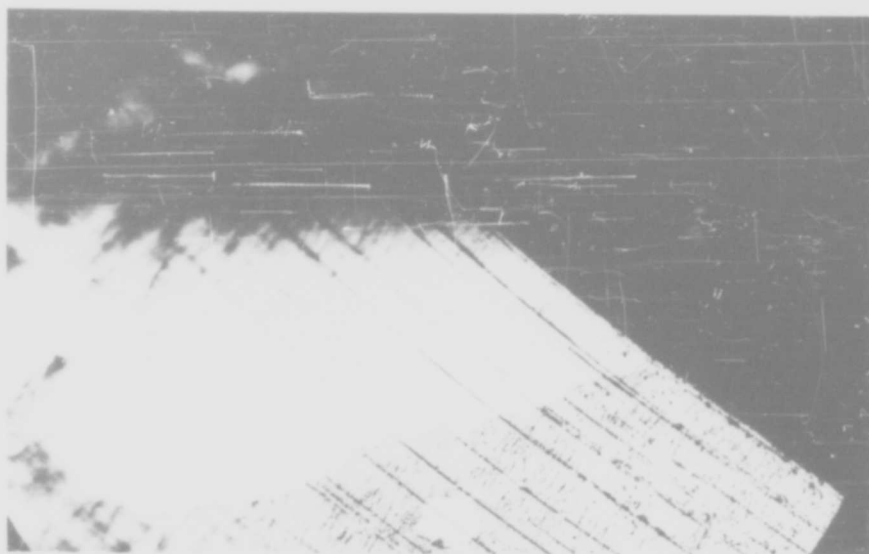
Fig. 23 Basal cleavages in cadmium -15.35 per cent magnesium alloy tested in tension a) specimen VII-6, -166^{\circ}\text{C} , away from main fracture \times 500 b) specimen VII-8, -126^{\circ}\text{C} , part of main fracture, \times 200
