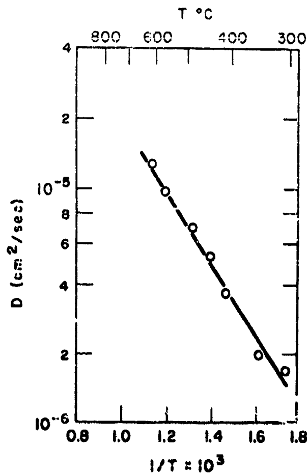
Fig. 28 - Temperature variation of diffusion coefficient for hydrogen in zirconium.(129)
