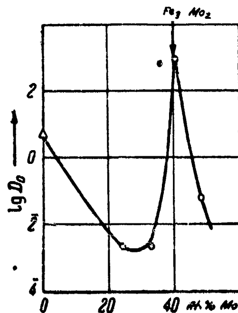
Fig. 11 - \text{Log } D_0 vs Atomic percent molybdenum for the iron-molybdenum system. (98)
