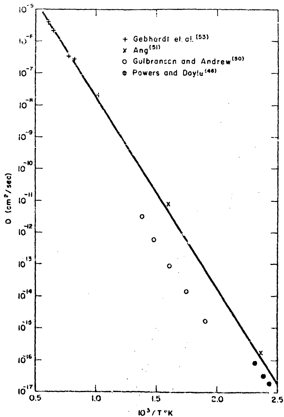
Fig. 7 - Temperature dependence of diffusion coefficient for tantalum-oxygen system.
