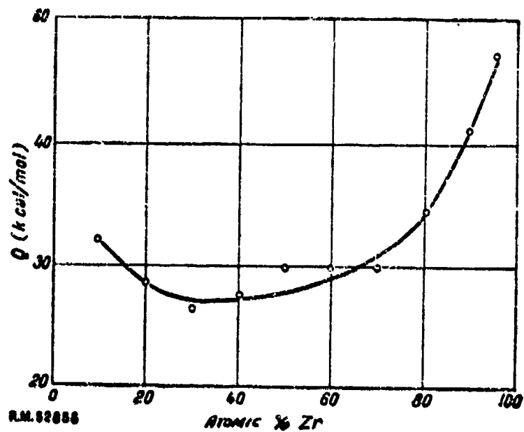
Fig. 32 - Variation of the activation energy for diffusion with composition for the zirconium-uranium system. (140)
