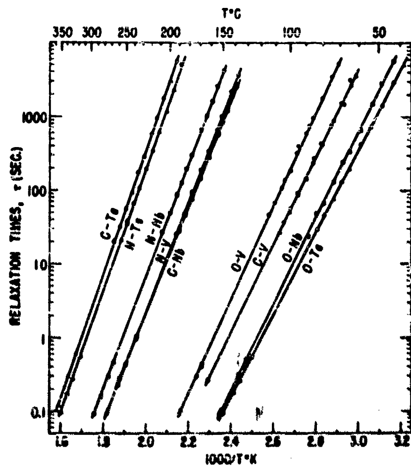
Fig. 4 - Relaxation times for stress-induced ordering vs 1/T for several alloys. (48)
