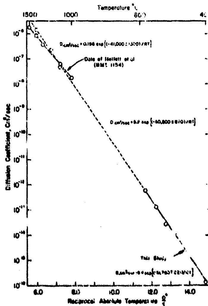
Fig. 30 - Temperature dependence of the diffusion coefficient of oxygen in zirconium. (133)
