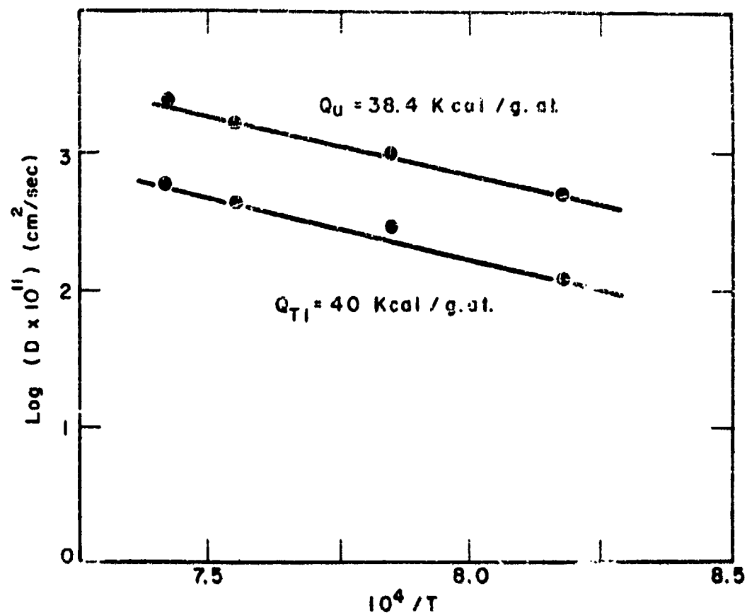
Fig. 48 - Temperature Dependence of intrinsic diffusion coefficients for uranium-titanium system. (180)
