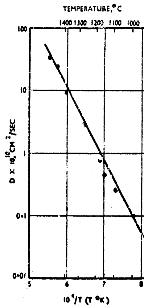
Fig. 39 - Temperature variation of the diffusion coefficient of nitrogen in titanium nitride. (171)
