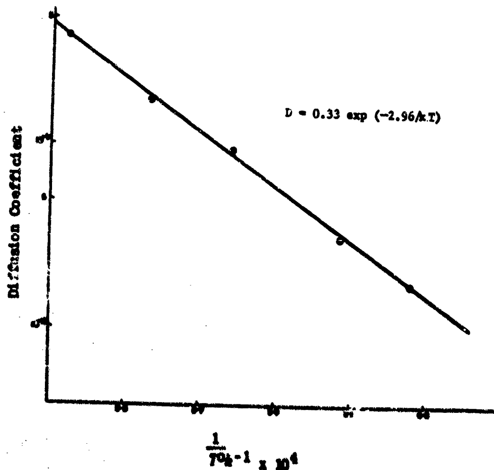
Fig. 26 - Log D vs 1/T for self-diffusion of platinum.(93)
