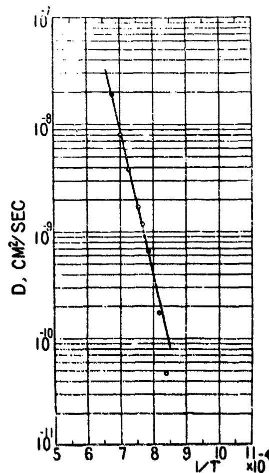
Fig. 36 - Influence of temperature on the interdiffusion coefficient of chromium in iron. (157)
