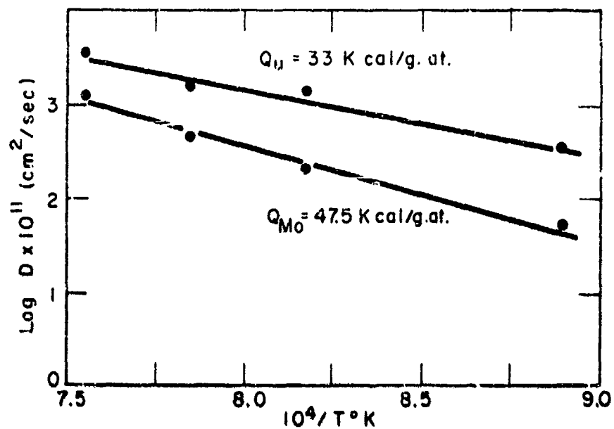
Fig. 19 - Temperature dependence of intrinsic diffusion coefficients for uranium-molybdenum system.(108)
