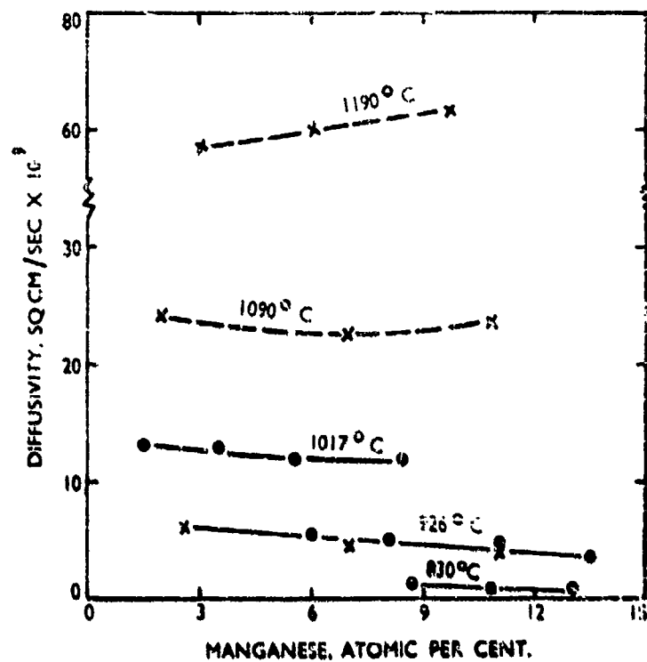
Fig. 43 - Variation of the interdiffusion coefficient with composition for the titanium-manganese system. (106) o = determined from transverse turnings x = determined from circumferential turnings
