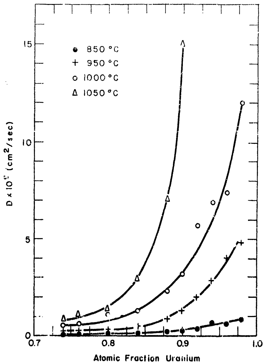
Fig. 17 - D vs composition for uranium-molybdenum system. (108)
