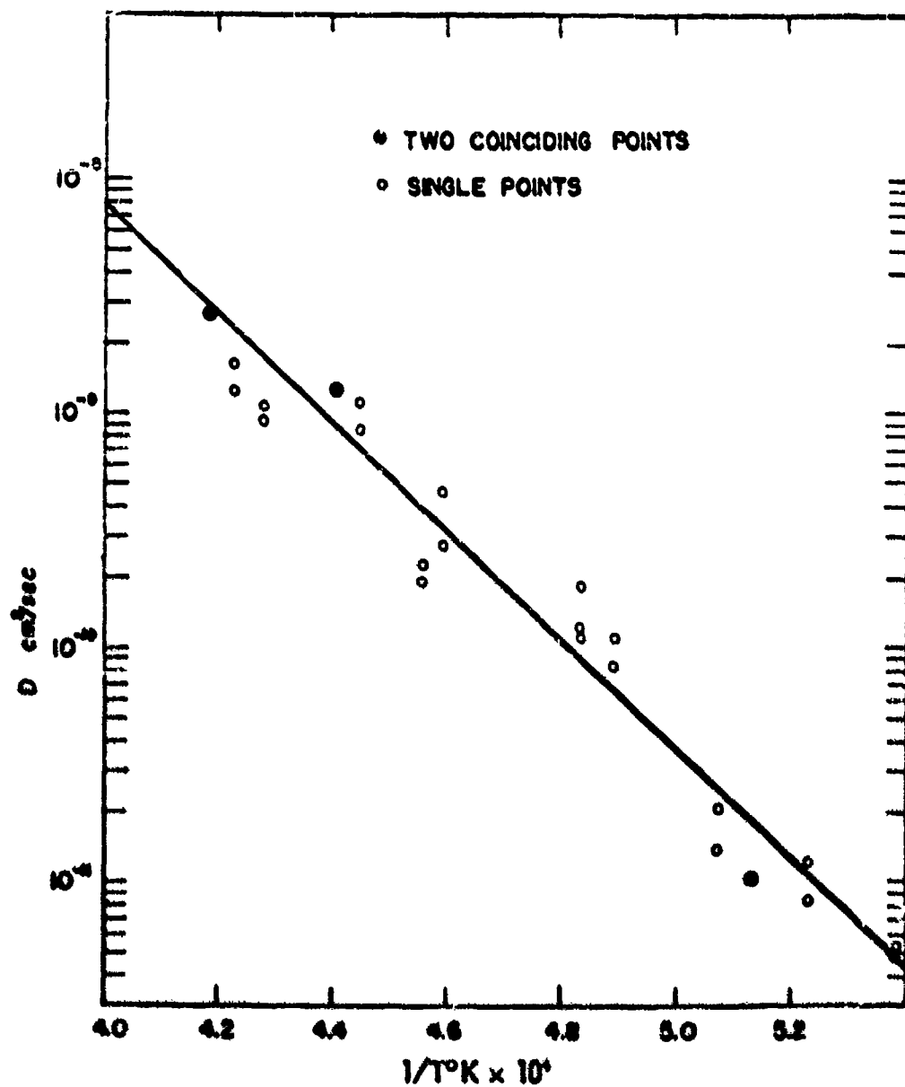
Fig. 20 - Log D vs 1/T for self-diffusion of niobium.(94)
