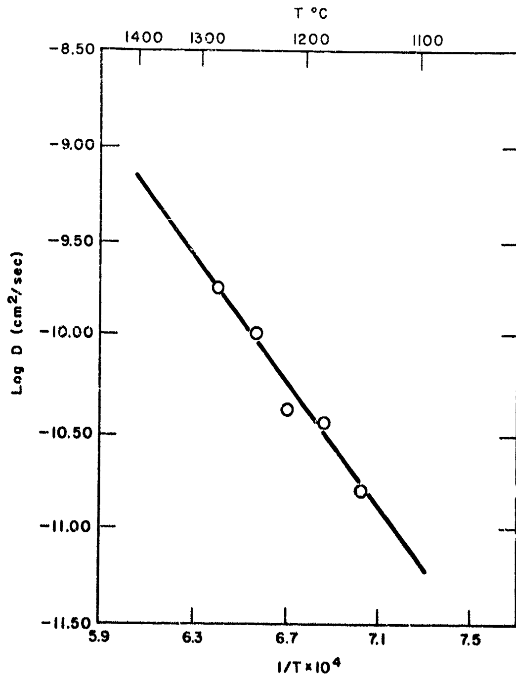
Fig. 2 - Log D vs 1/T is plotted for diffusion in tungsten-nickel alloys of high nickel concentration. (32)
