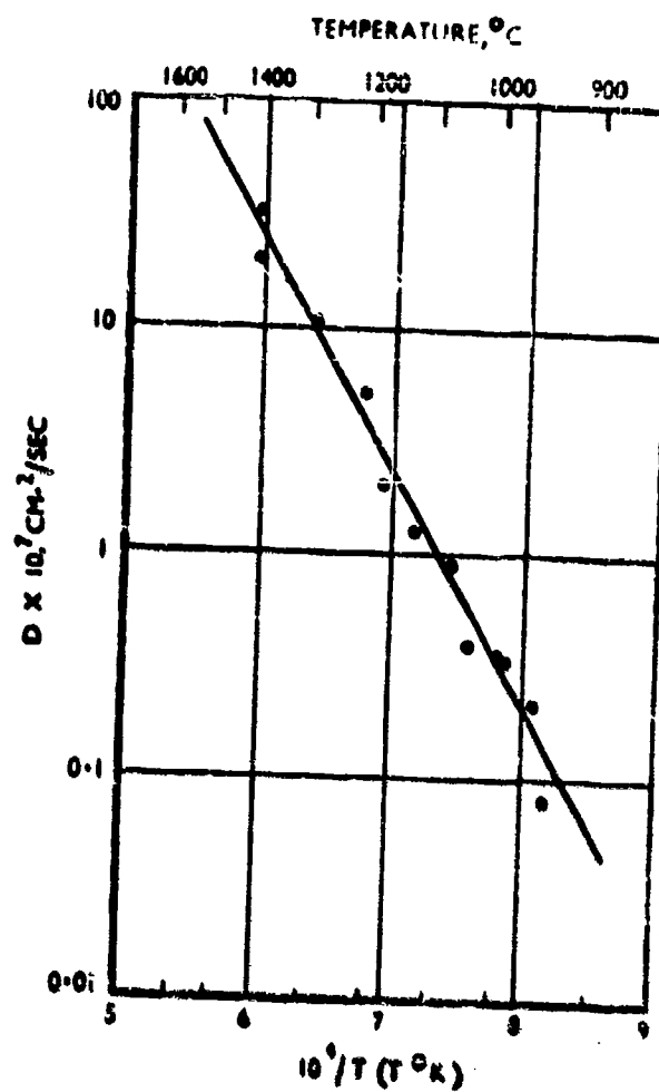
Fig. 40 - Temperature variation of the diffusion coefficient of oxygen in beta-titanium. (171)
