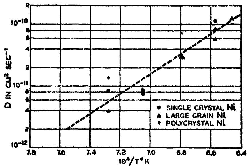
Fig. 3(b) - The temperature dependence of the diffusion from a tungsten layer into pure nickel. (33)
