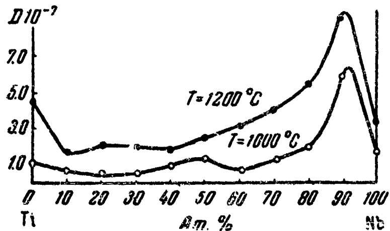
Fig. 22 - Variation of the diffusion coefficient of \text{Sc}^{46} with composition for the niobium-titanium system. (113)
