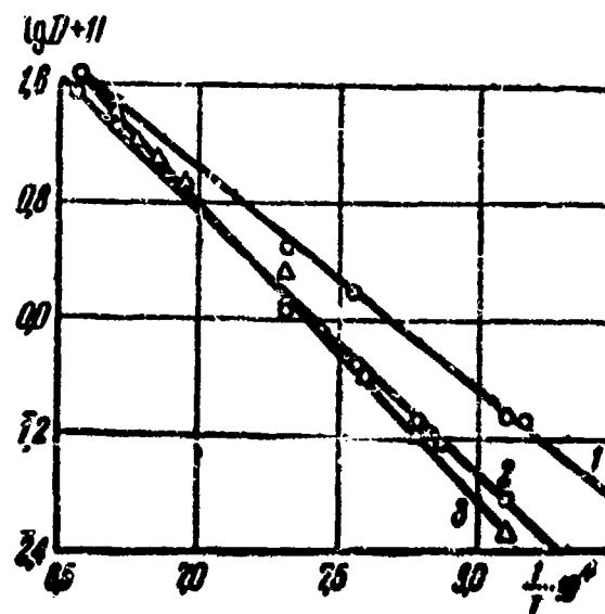
Fig. 49 - Temperature dependence of the diffusion coefficient of \text{Fe}^{59} in alloys of the systems: (1) Ni-Ti, (2) Ni-Ti-Cr, (3) Ni-Ti-Cr-W-Al. (181)
