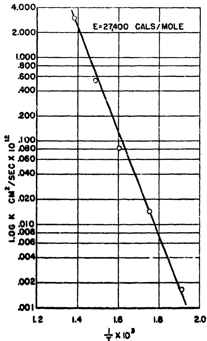
Fig. 6 - \log K vs 1/T for the reaction of tantalum with oxygen. (30)
