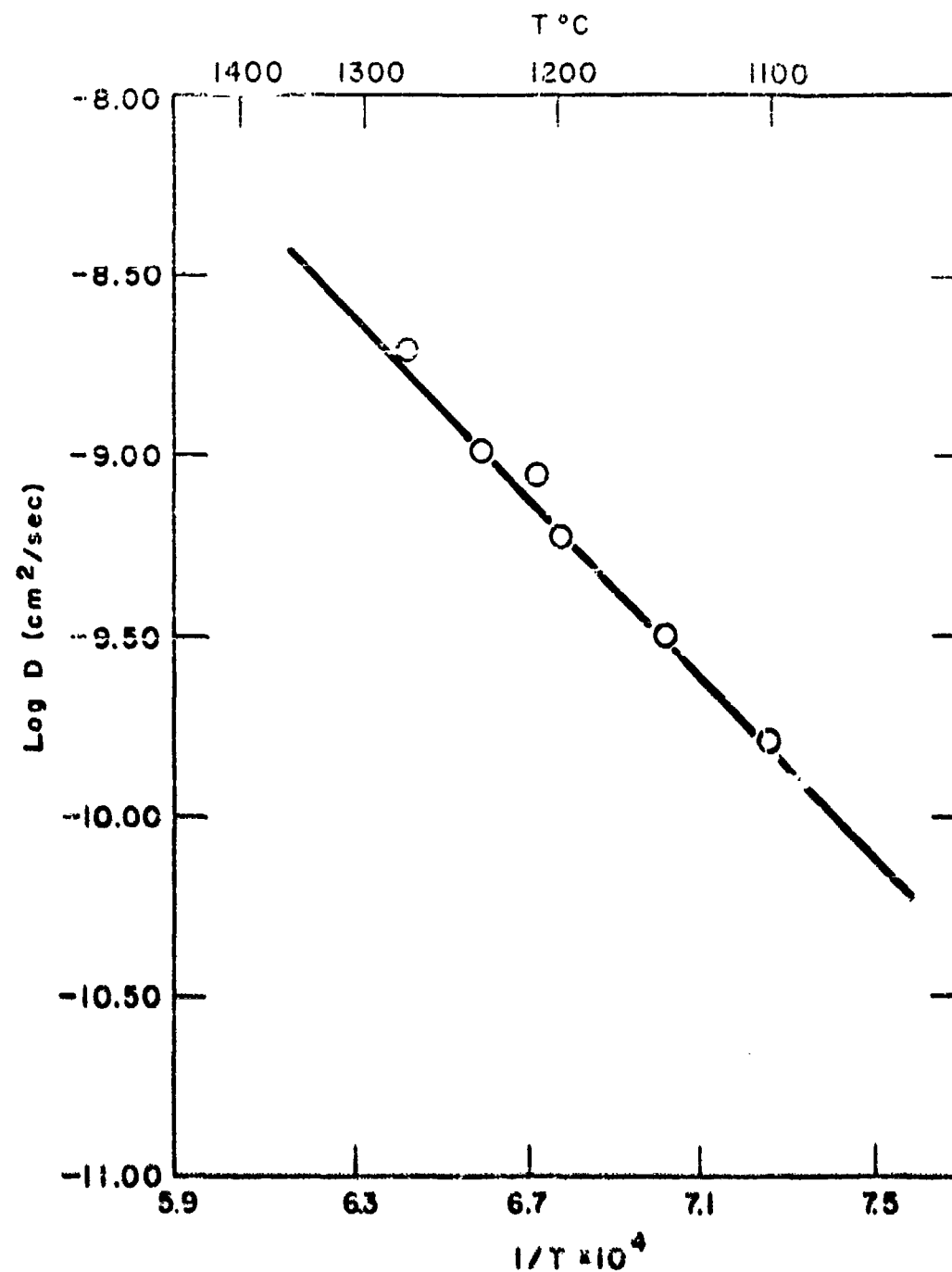
Fig. 44 - Log D vs 1/T is plotted for diffusion in titanium-nickel alloys of high nickel concentration. (32)
