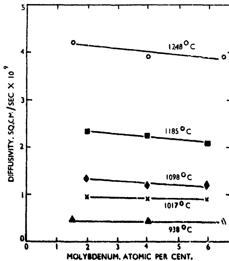
Fig. 16 - Variation of the interdiffusion coefficient with composition for the molybdenum-titanium system. (106)
