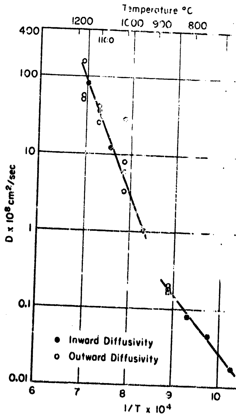
Fig. 41 - Diffusivity of oxygen in alpha and beta titanium
