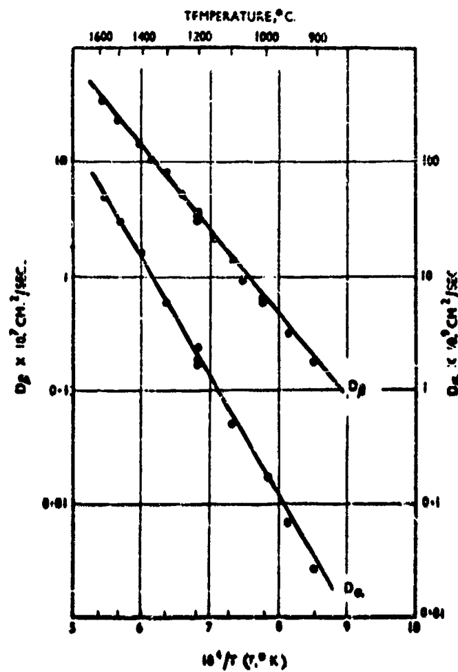
Fig. 30 - Temperature variation of the diffusion coefficient of nitrogen in alpha and beta-titanium. (171)
