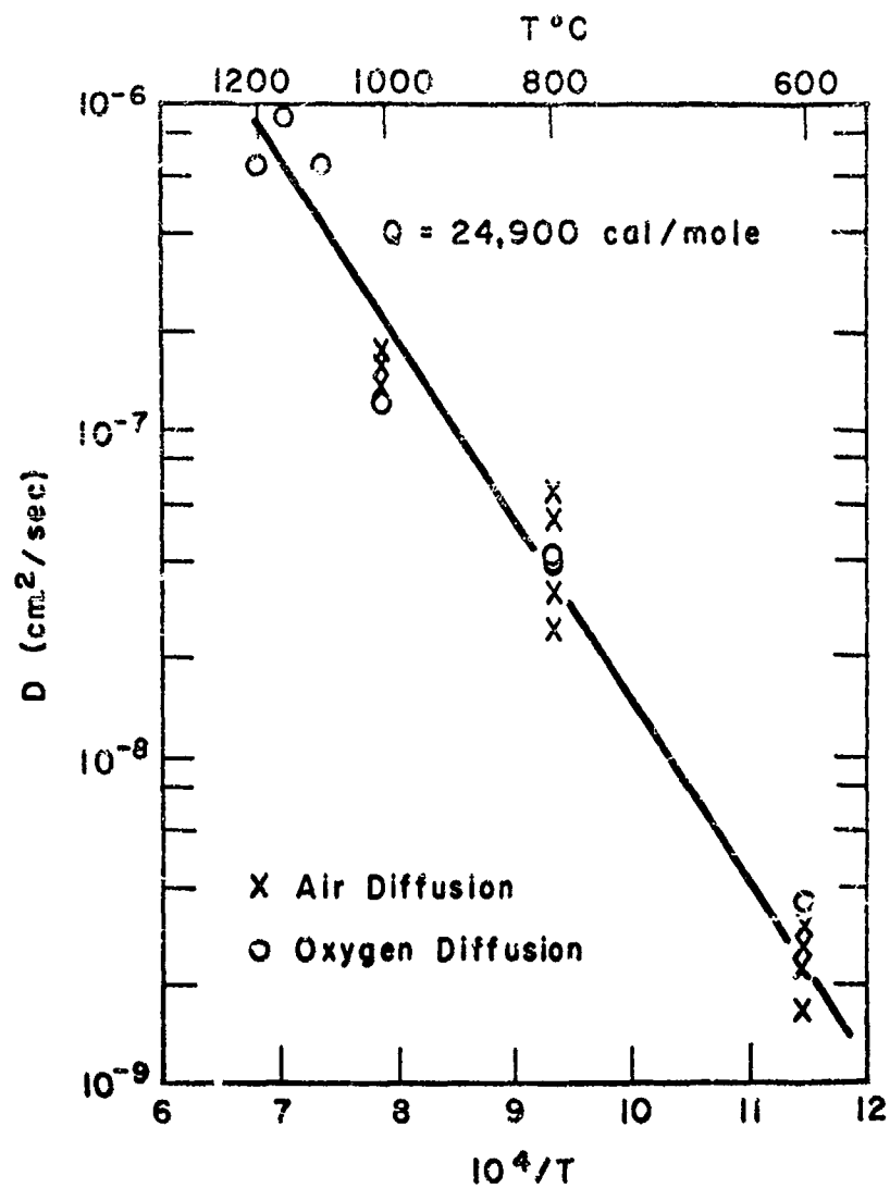
Fig. 21 - Temperature dependence of D for contamination of niobium in oxygen and air. (112)
