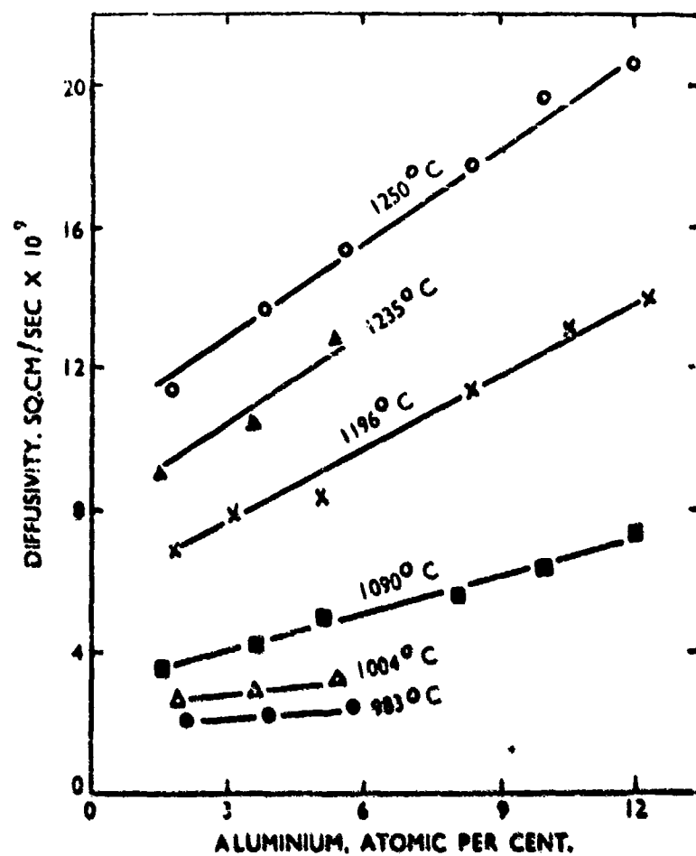
Fig. A2 - Variation of the interdiffusion coefficient with composition for the titanium-aluminum system. (106)
