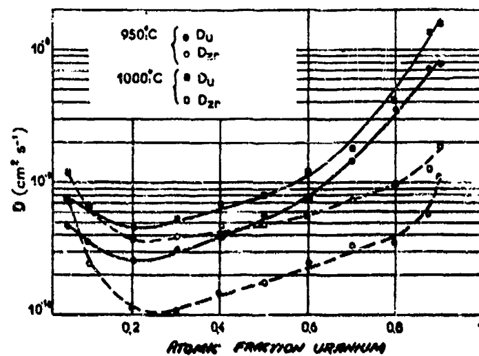
Fig. 34 - Variation of the intrinsic diffusion coefficients (192) with composition for the zirconium-uranium system.
