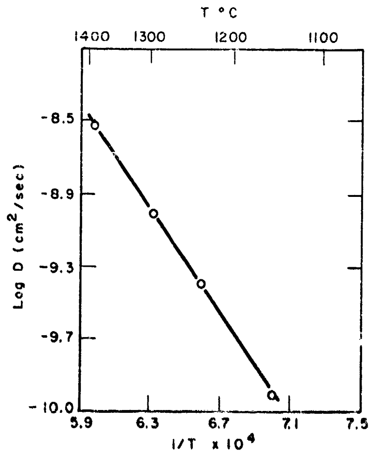
Fig. 15 - Log D vs 1/T for diffusion in molybdenum-nickel alloys of high nickel concentration. (104)
