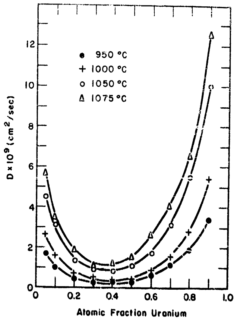
Fig. 46 - D vs composition for uranium-titanium system. (180)
