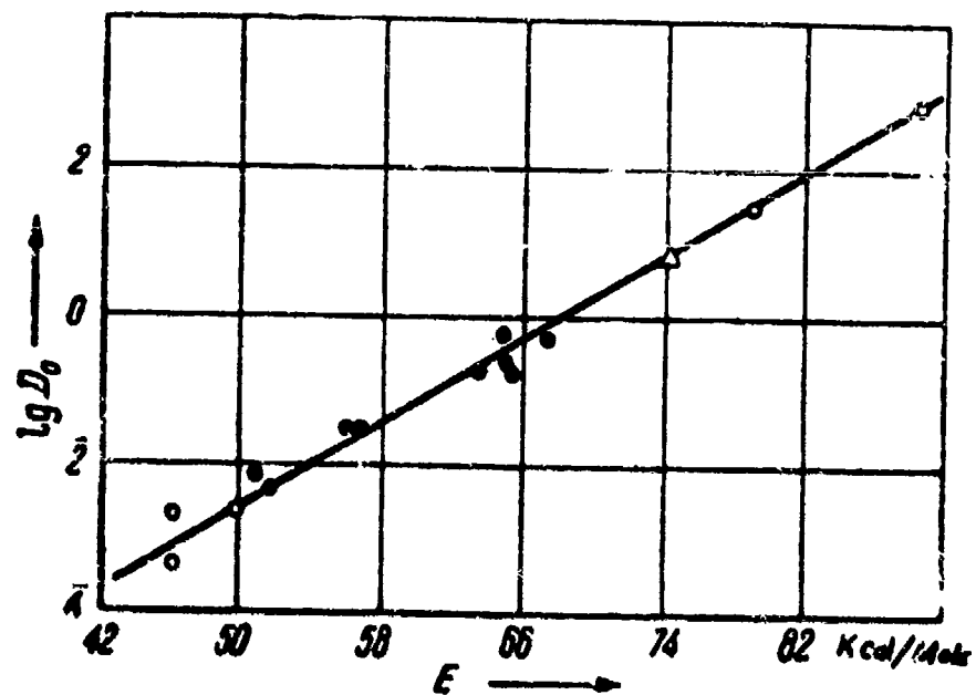
Fig. 12 - \lg D_0 vs the activation energy for o - Fe-Mo, (98) \Delta - Fe-self-diffusion (89) and e - Fe-Ni. (99)
