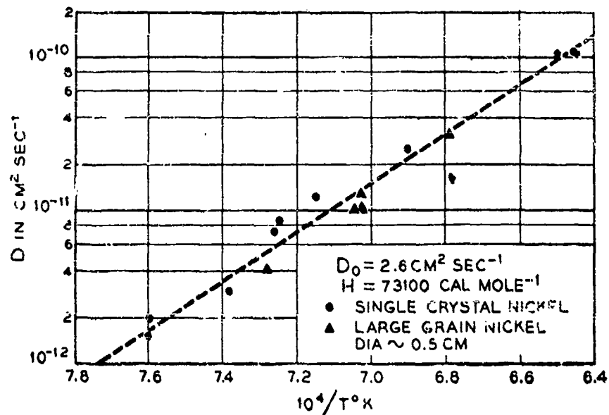
Fig. 3(a) - The temperature dependence of the diffusion from a tungsten-nickel alloy into pure nickel. (33)
