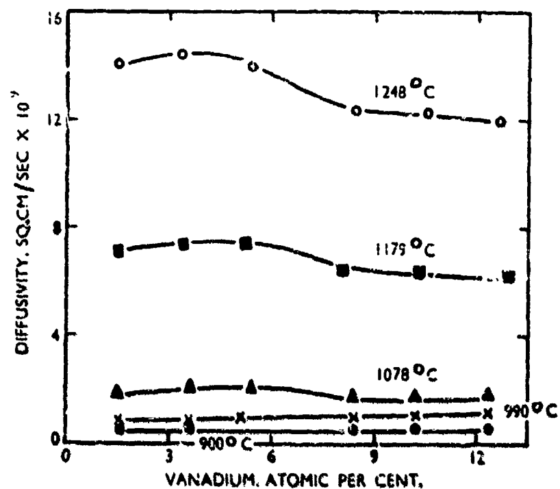
Fig. 35 - Variation of the interdiffusion coefficient with composition for the vanadium-titanium system. (106)
