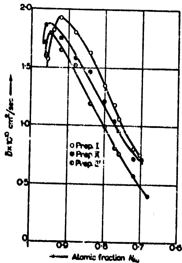
Fig. 27 - The dependence of D on composition. I and II diffused at 1038^\circ\text{C} , III diffused at 1002^\circ\text{C} . (117)
