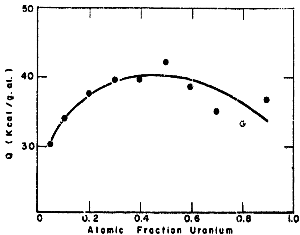
Fig. 47 - Dependence of Q on composition for the uranium-titanium system. (180)
