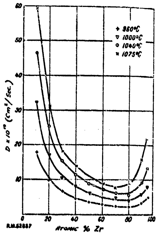
Fig. 31 - Variation of the diffusion coefficient with composition for the zirconium-uranium system. (140)
