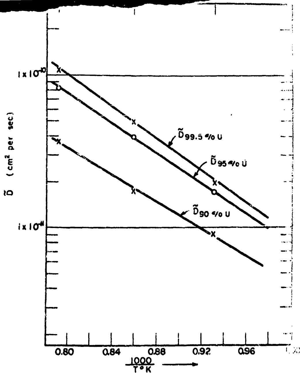
Fig. 24 - \tilde{D} as a function of 1/T for uranium-niobium diffusion. (11)
