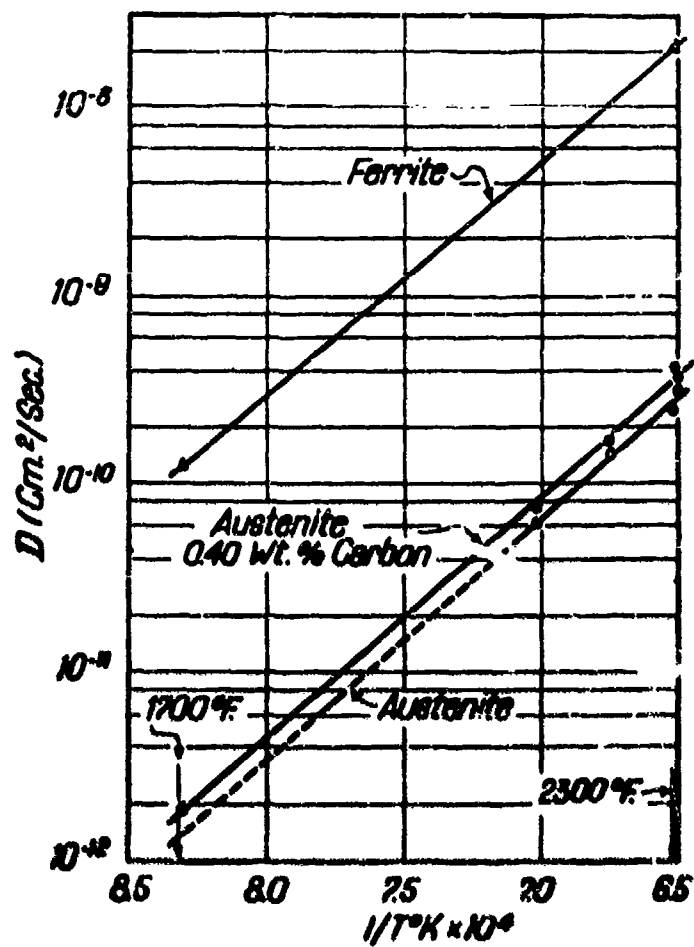
Fig. 13 - Effect of temperature on the coefficient of diffusion of molybdenum in austenite and in ferrite. (101)
