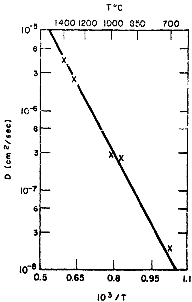
Fig. 5 - Temperature dependence of the diffusion coefficient for oxygen in tantalum. (53)
