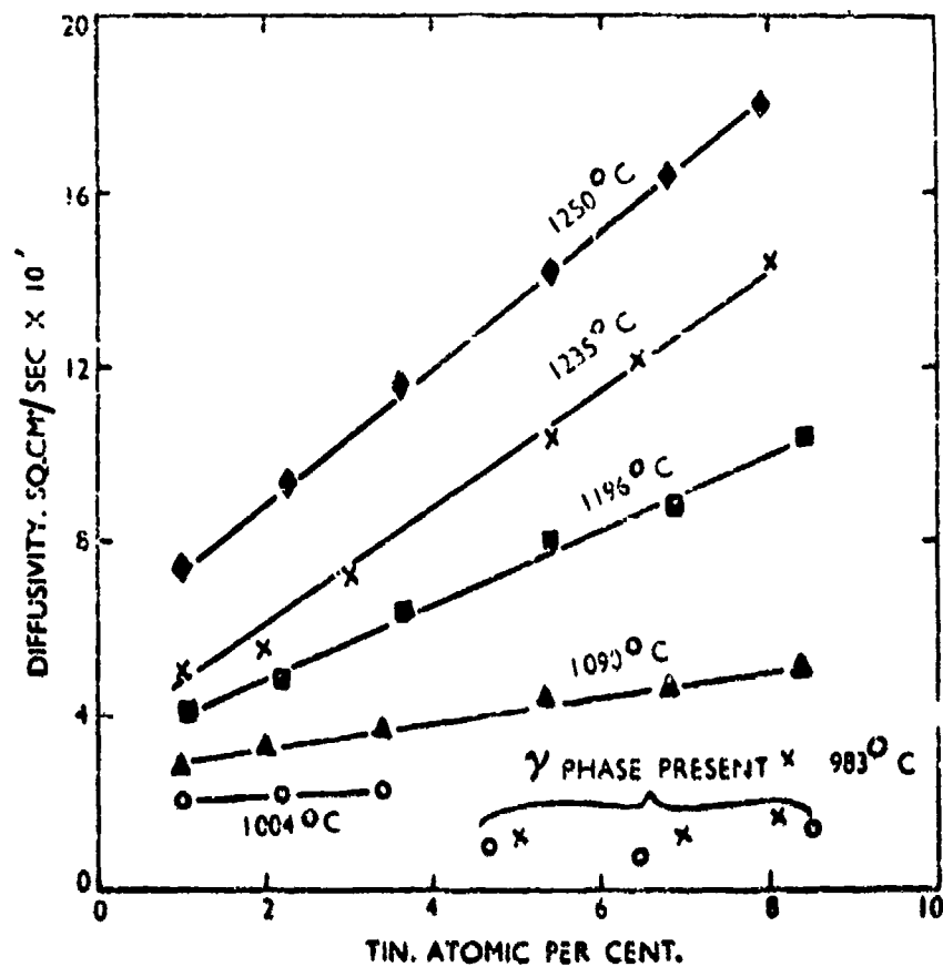
Fig. 45 - Variation of the interdiffusion coefficient with composition for the titanium-tin system. (106)
