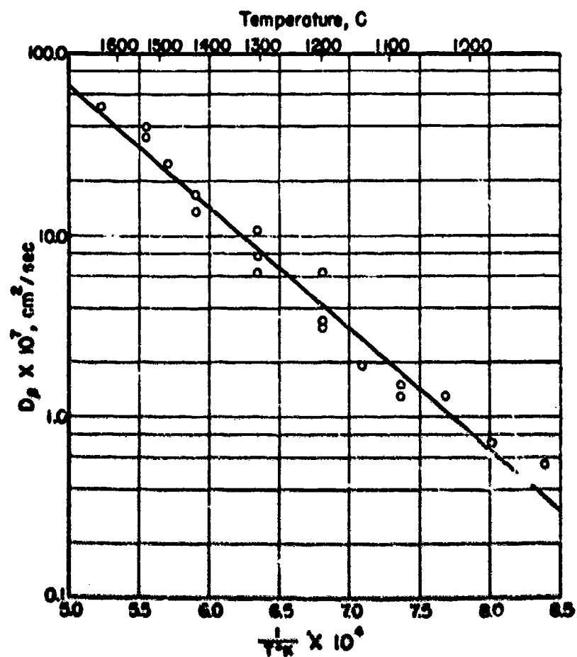
Fig. 29 - Variation of the diffusion coefficient with temperature for diffusion of nitrogen in zirconium. (132)
