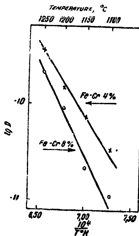
Fig. 37 - \log D vs 1/T for diffusion of Fe^{59} in Fe - 4% Cr and Fe - 8% Cr Alloys. (158)
