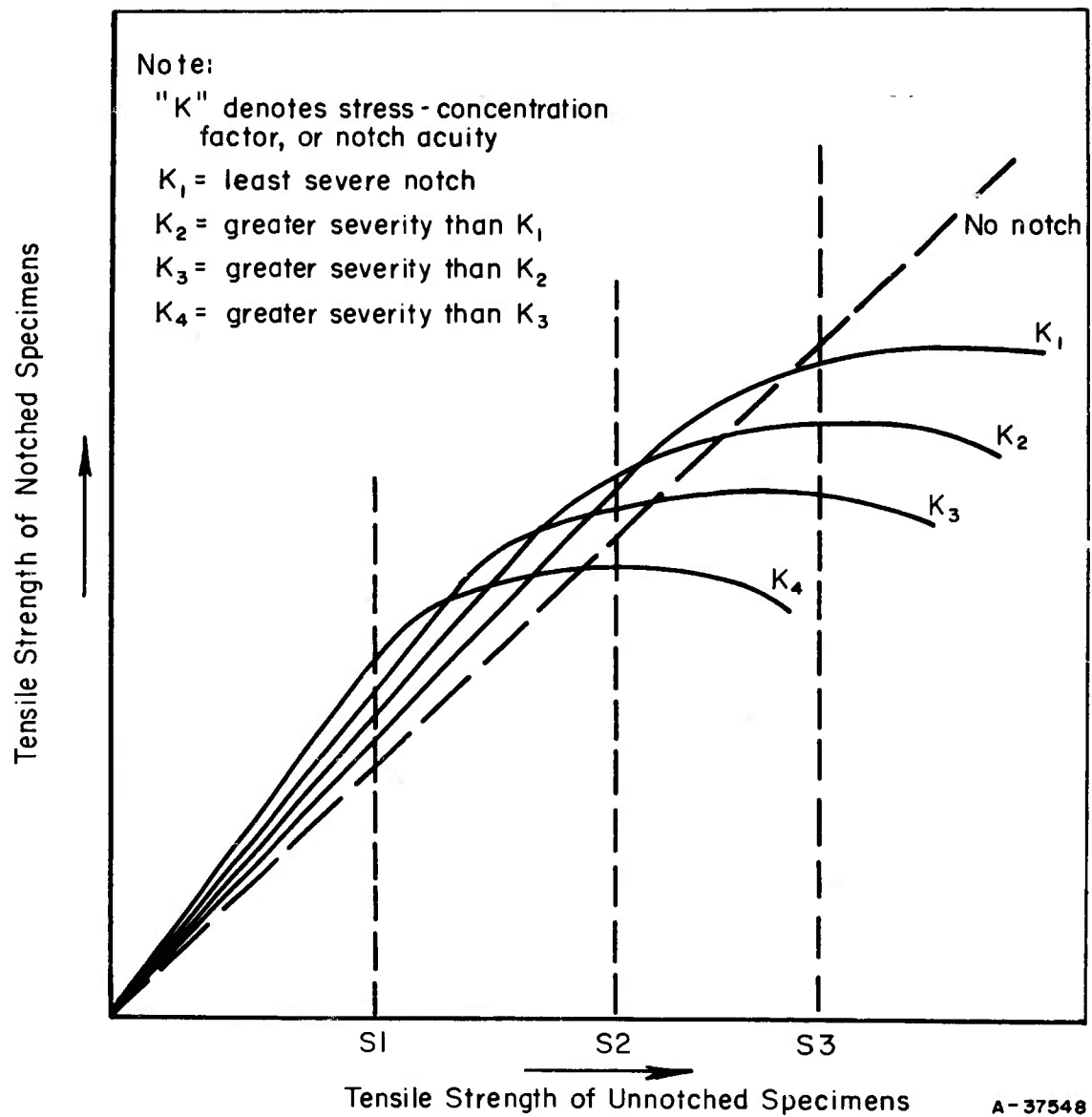
FIGURE 13. SCHEMATIC REPRESENTATION OF THE EFFECT OF STRENGTH LEVEL AND STRESS-CONCENTRATION FACTOR ON THE TENSILE STRENGTH OF NOTCHED SPECIMENS
