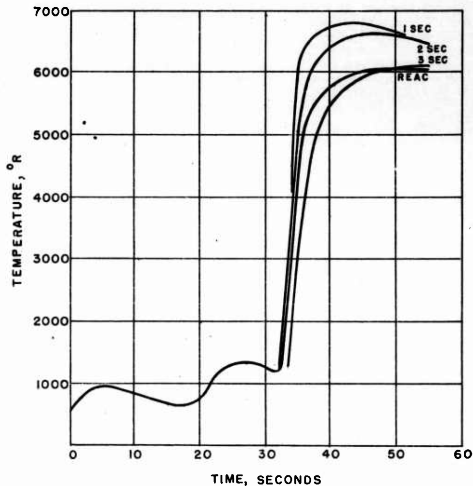
FIG. 17. Outside Wall Temperature Versus Time Comparison-- Zero Emissivity, Astrolite.
