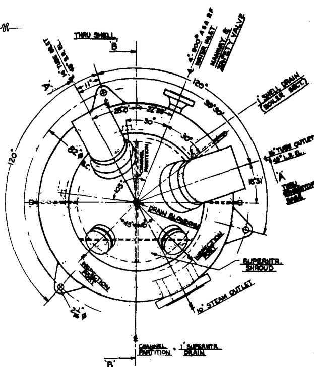
BOTTOM VIEW LOOKING UP
