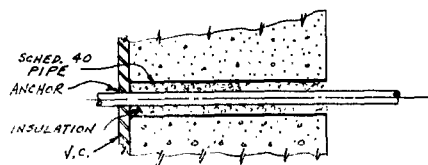
TYPICAL DETAIL FOR LINES UNDER 300°F.
