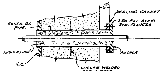
TYPICAL DETAIL FOR LINES OVER 300°F.
