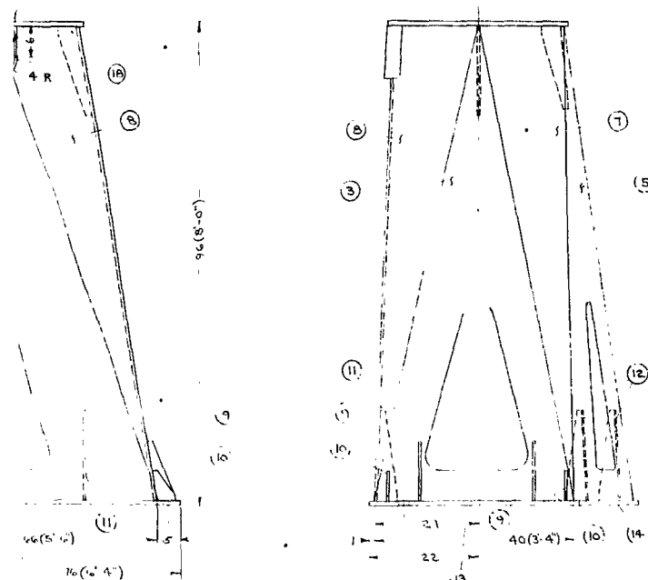
SECTION B-B SCALE 3"=1'-0"
