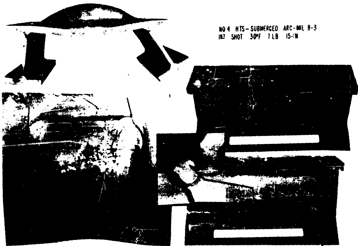
Figure 5 - Test specimen No. 4 after one explosive shot. Arrows indicate extent of ruptures. Insert shows submerged-arc weld failure.
