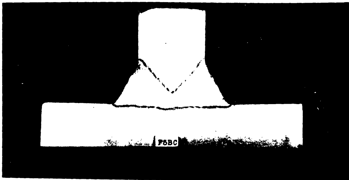
Figure 12 — Peened Specimen
