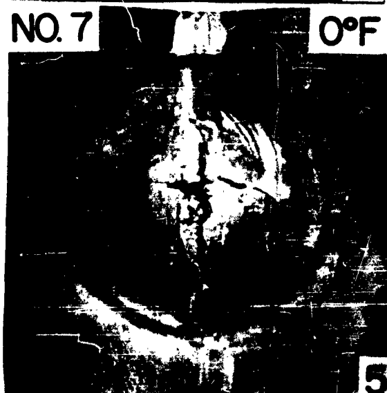
Figure 6 — Explosion-bulge test sample with modified sub-arc weld. Weld crown removed and tested to visible signs of failure (top), and under conditions of forced propagation (bottom).
