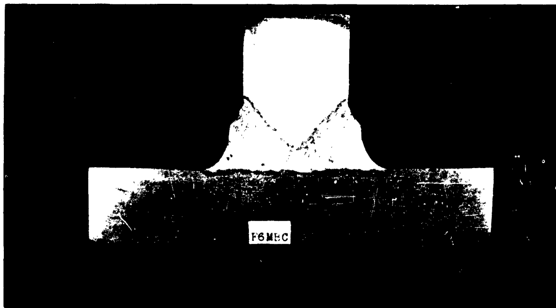
Figure 20 — Ground and Peened Specimens
