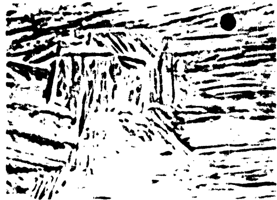
(f) M_f - 830 F, Time 23 Minutes
