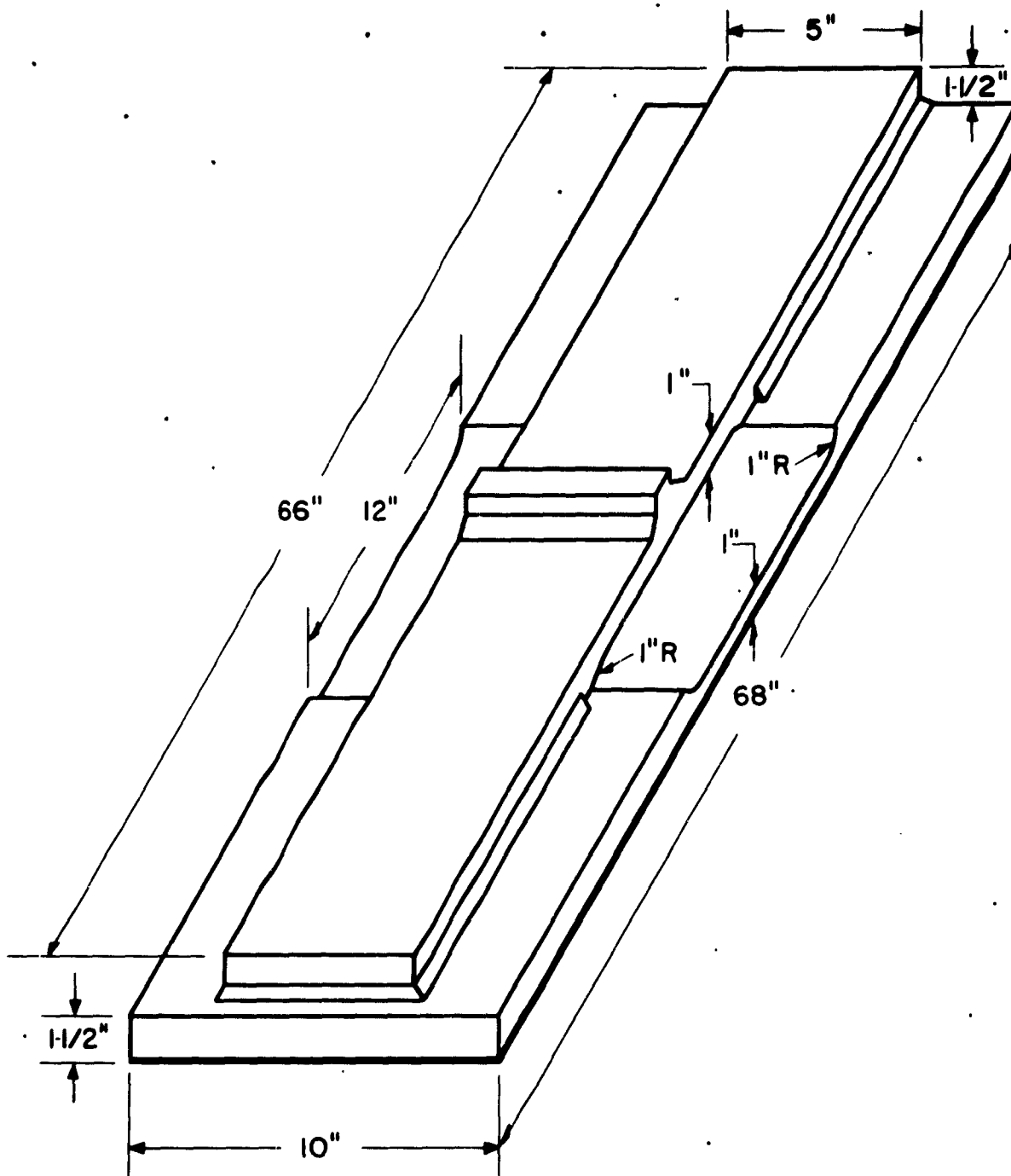
Figure 1 — Large Scale Beam Type Fatigue Specimen
