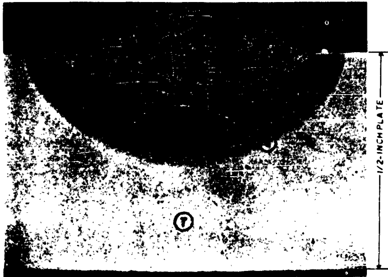
Figure 22. Photomicrograph of bead weld in USS "T-1" steel plate welded at 70 F. Numbered circles identify the zones described below. Etched in Nital. X7.
