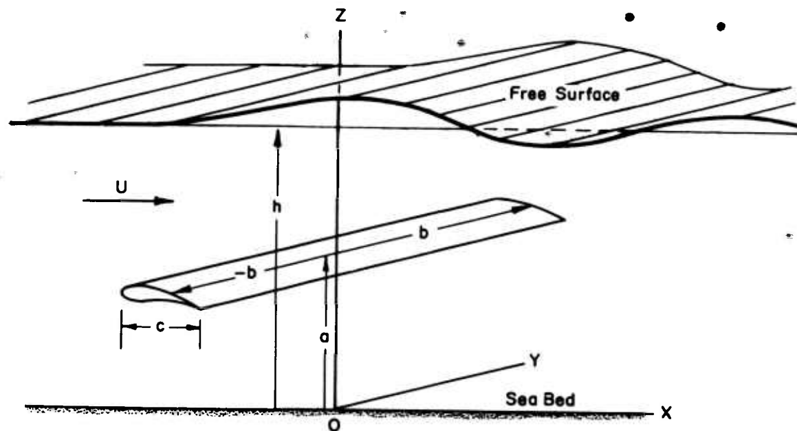
Figure 1 - Coordinate System for a Hydrofoil in Shallow Water
