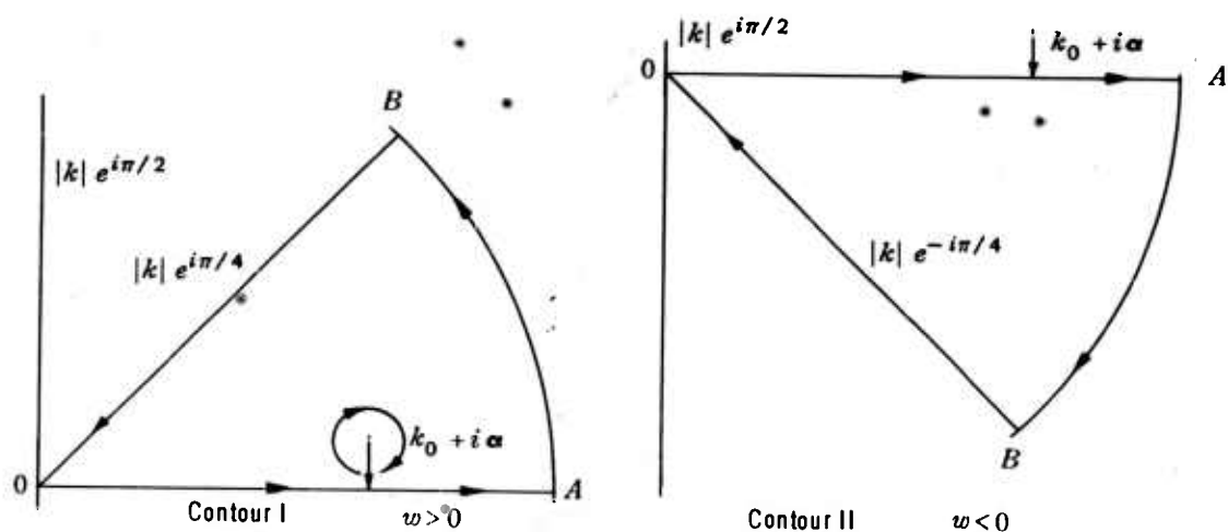
Figure 2 - Contours in the Complex k -Plane for Evaluating the Integrals
