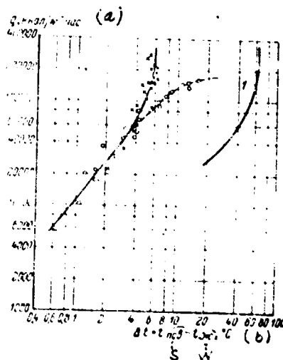
Fig. 99. Heat transfer from boiling mercury containing additives of Na, Mg, Ti. (1) Farmer solution; (2) - 0.1% Na; (3) - 0.02% Mg and 0.0001% Ti. (a) q , kcal/m 2 hr; (b) temperature drop equals the temperature of the surface minus the temperature of the liquid °C.
