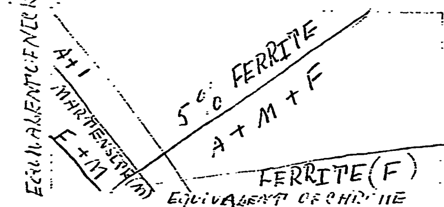
Fig. 37. Structural Diagram for casting chrome-nickel steel.
