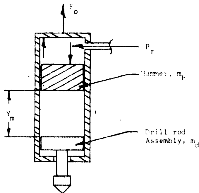
Schematic Diagram of Contact-Force Recoilless Impactor
