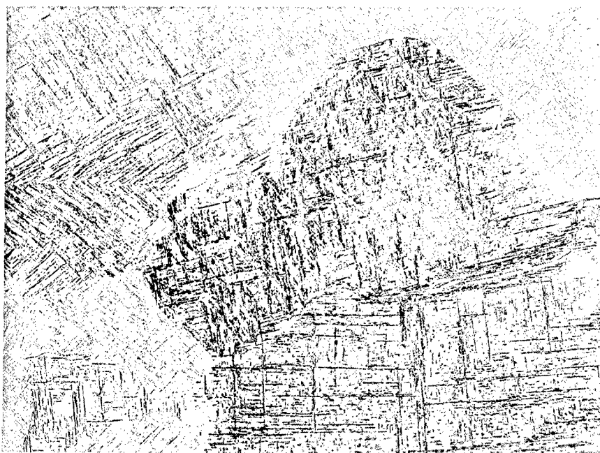
FIGURE 9. WELD-METAL STRUCTURE OBTAINED BY DEPOSITING Ti-6Al-4V FILLER WIRE IN Ti-6Al-4V BASE PLATE
