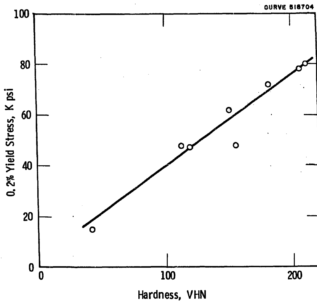
Fig. 62--Yield stress at 2200 0 F as a function of hardness at 2000 0 F
