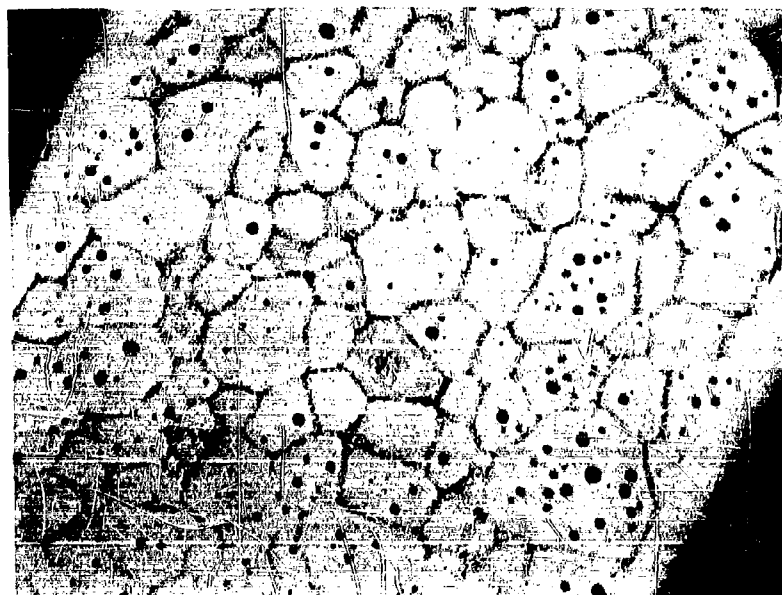
Fig. 18--Ta-6.3 Zr, 15 minutes at 2600 0 C, radiation quenched. 100X
