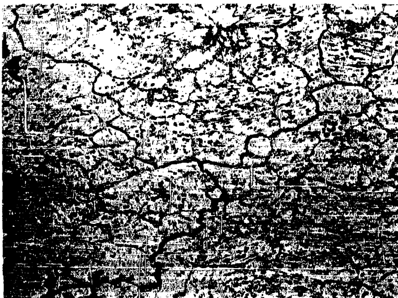
Fig. 8--Microstructure of a Ta-8 Zr consumably arc melted billet which exploded during Dynapak extrusion. Billet was held 2 minutes at 1750°C, allowing the billet 7 minutes to reach temperature prior to extrusion. 100X
