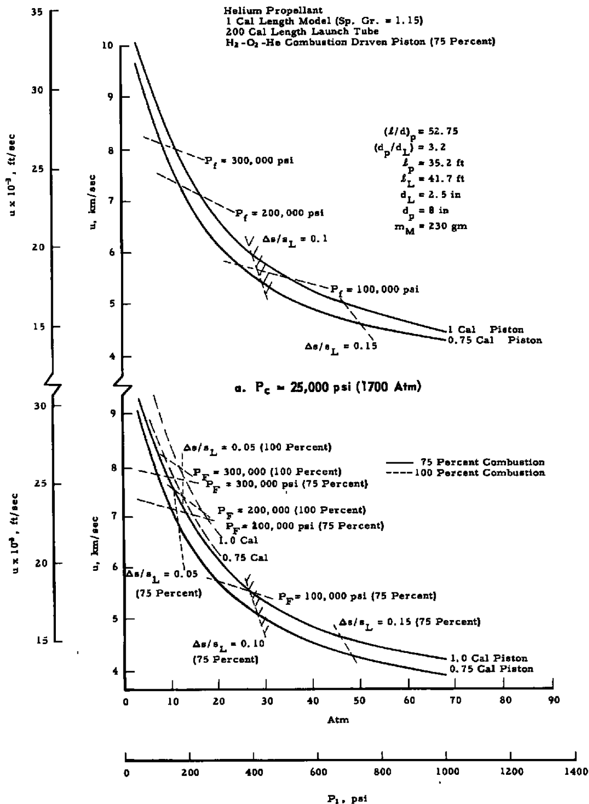
Fig. 18 Estimated Performance of Launcher
