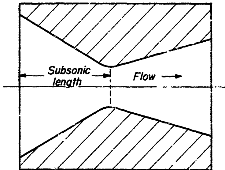
Conical nozzle
