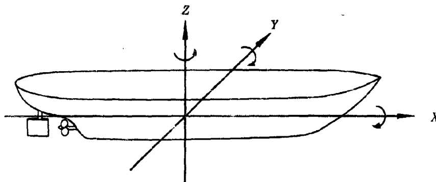
Figure 2-1 – Axes through the Center of Gravity of a Ship with Respect to Which Forces and Moments Exerted by the Water May Be Defined
