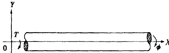
Figure 3-3 - Cylindrical Shaft with Axis Coinciding with OX and Twisting about OX
