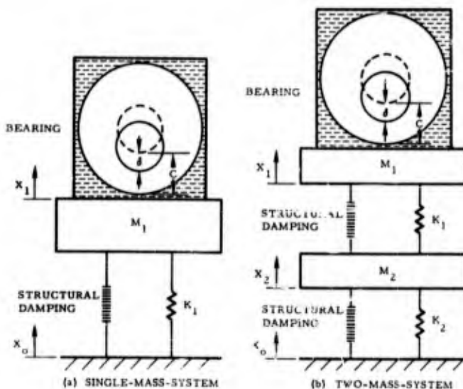
Fig. 1 - Single-mass and two-mass representations of mounting structure and bearing
