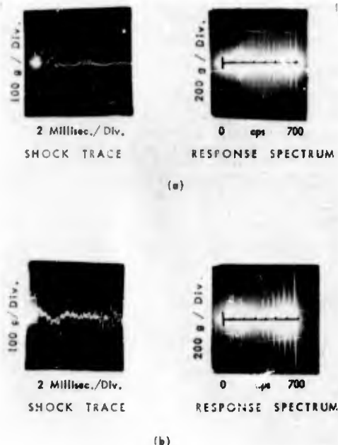
Fig. 11 - The response of the analyzer to shocks resulting from field environment: (a), a pivot drop of a solid, simple structure and (b), the pivot drop of a complex structure
