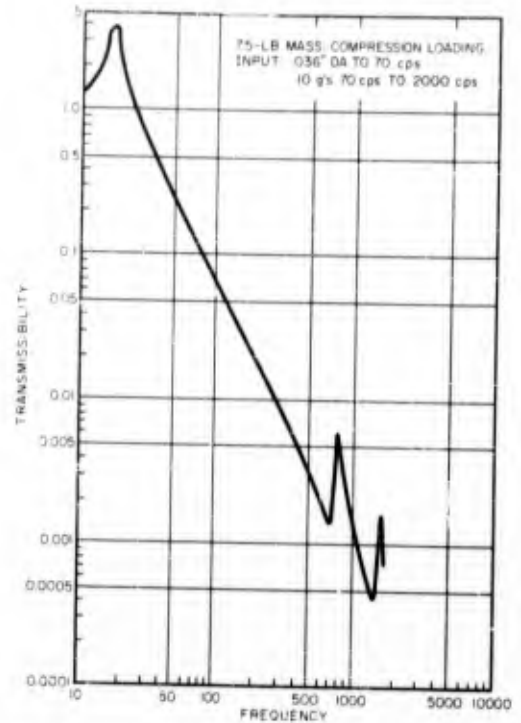
Fig. 7 - Vibration transmissibility for coupled-compression isolator (aircraft type)
