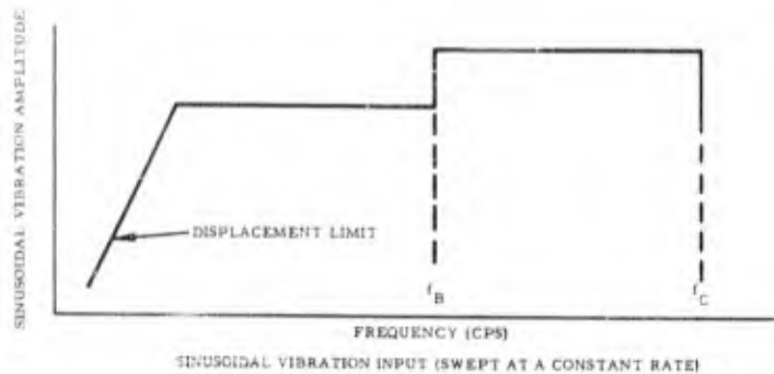
Fig. 4 - Typical acceleration profiles for combined, random- and sinusoidal-vibration input
