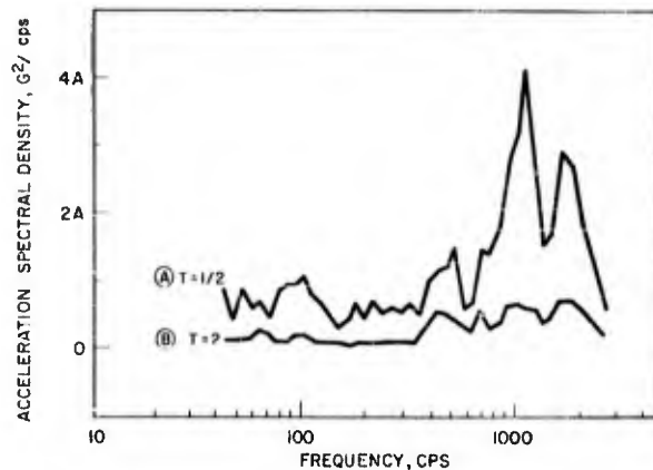
Fig. 9 - Spectra at t seconds from beginning
