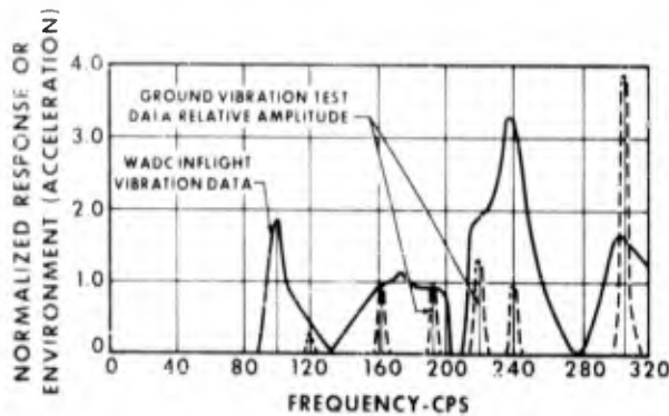
Fig. 4 - High-frequency correlation of flight-environment and ground-vibration test data
