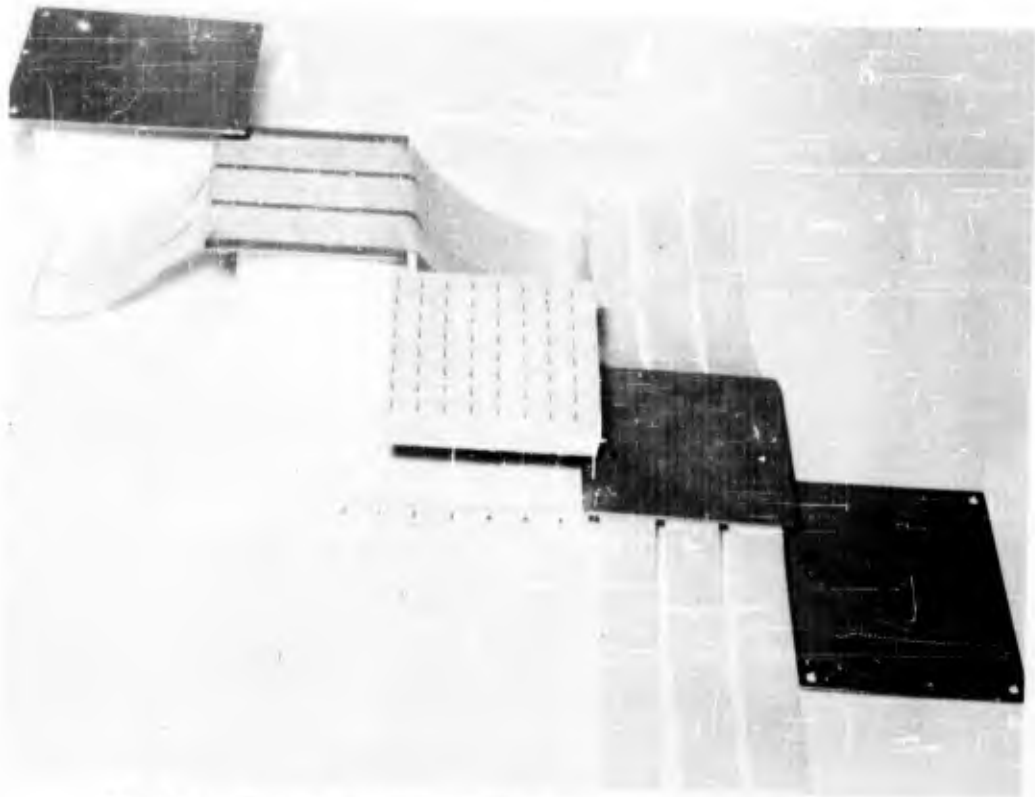
Fig. 8 - Assembly of the experimental coupled-compression shock isolator
