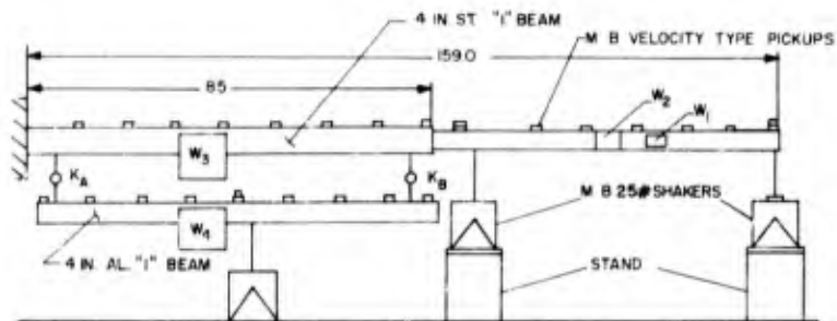
Fig. 3 - Restrainted two-beam system (laboratory test)
