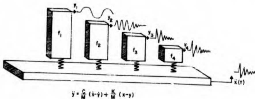
Fig. 1 - Idealized equipment
