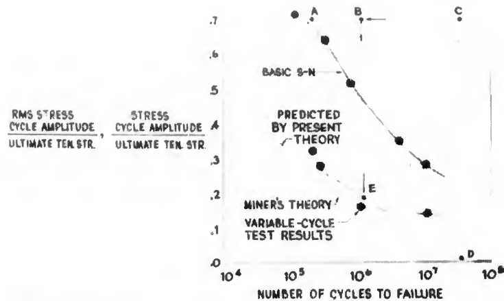
Fig. 18 - Variable-cycle, random-load, fatigue-test results for notched 2024-T3 sheet in reversed bending, Trotter [22], 1956.
