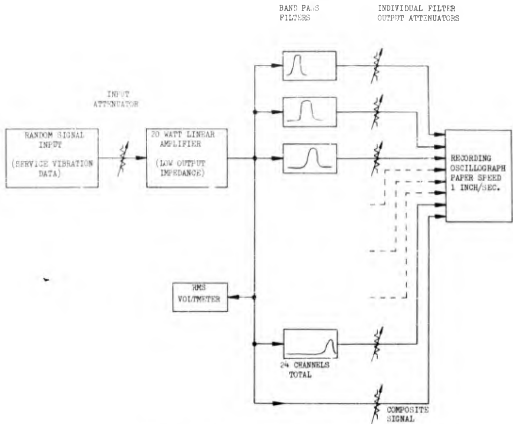
Fig. 2 - Diagram of the comb filter unit
