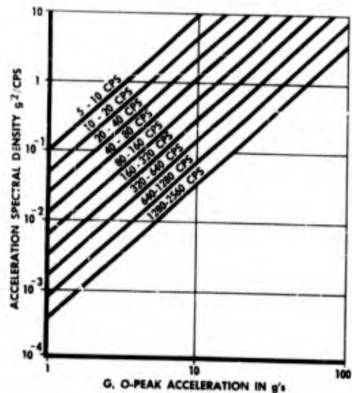
Fig. 6 - Equivalence curves for random noise versus sweep
