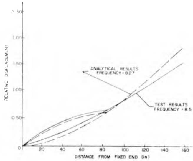
Fig. 4 - Restrained two-beam system (first mode)
