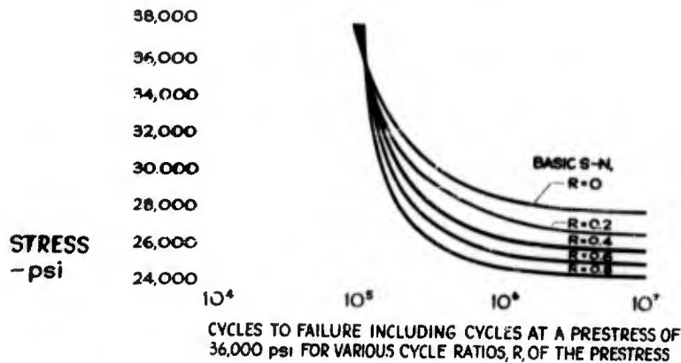
Fig. 2 - Results of rotating-beam tests of SAE 1020 steel, Kommers [14], 1945
