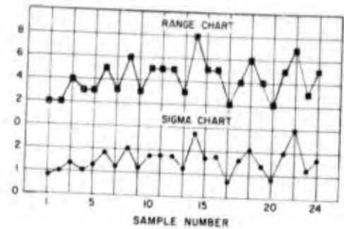
Fig. 8 - Range and standard deviation similarity
