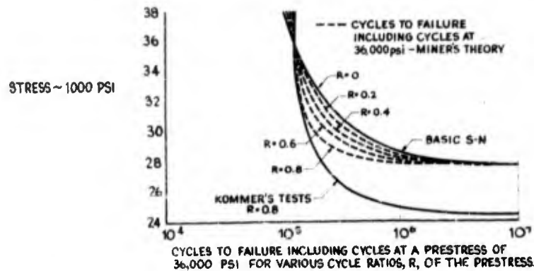
Fig. 5 - Comparison of Miner's theory with test results for SAE 1020 steel, Kommers [14], 1945
