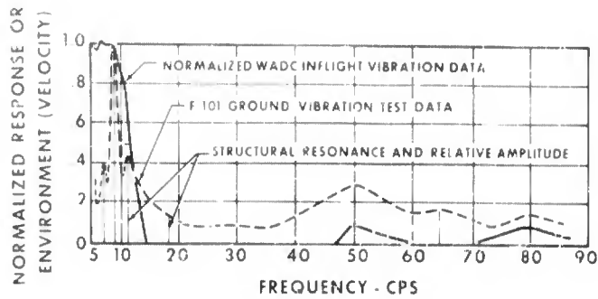
Fig. 3 - Low-frequency correlation of flight-environment and ground-vibration test data
