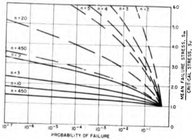
Fig. 11 - Probability of failure vs mean failure stress, as a function of sample size for two ranges: R = 3.00 S_c and R = 0.500 S_c
