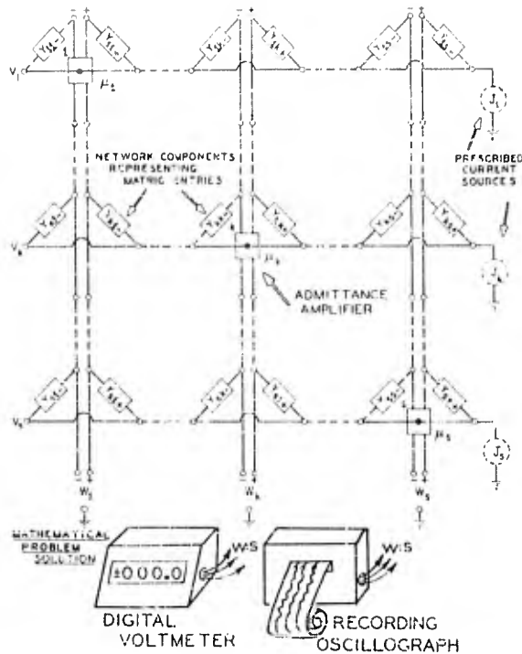
Fig. 1 - Electronic synthesis network which is homeomorphic to mathematical matrix Eq. (1)
