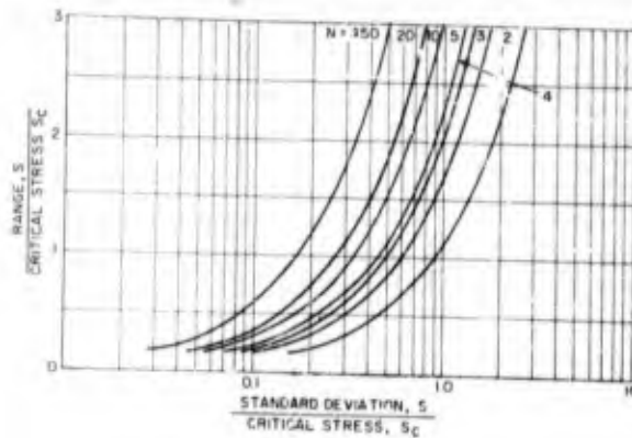
Fig. 9 - Range vs standard deviation as a function of n
