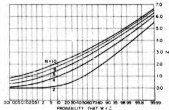
Fig. 7 - Probability of the relative range w = R/\sigma for various sample sizes
