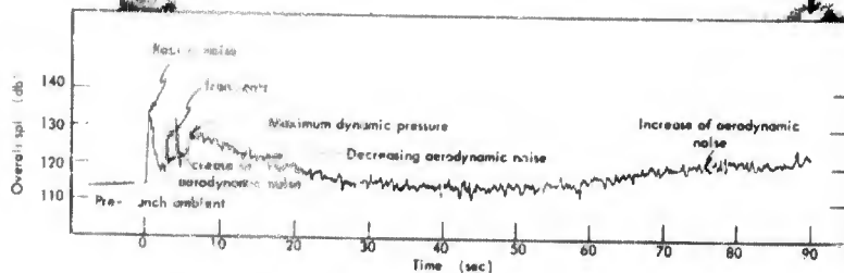
Fig. 2 - Graphic level recording of variation of over-all noise level inside forward compartment of a small missile during its flight
