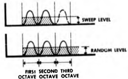
Fig. 4 - Consideration of response due to sinusoidal sweep and random noise for modes in other octaves
