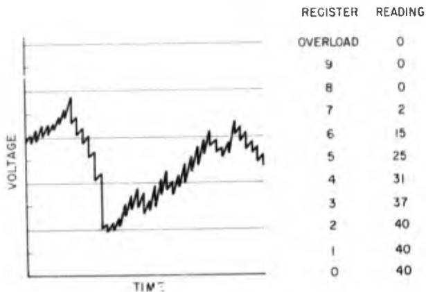
Fig. 4 - Operation of the discriminators in the M. S. mode
