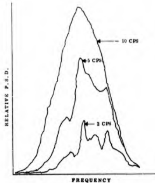
Fig. 1 - Complex resonances which are not shown by a 10-cps filter are revealed by a 2-cps filter. The 10-cps filter has five times as much energy in its passband as does the 2-cps filter, therefore, the area under the 10-cps filter plot is five times greater than the 2-cps plot. Generally, the plots are normalized by dividing the filter output by its bandwidth, and so obtaining the energy per cycle. In such cases, the area under all plots will be the same.
