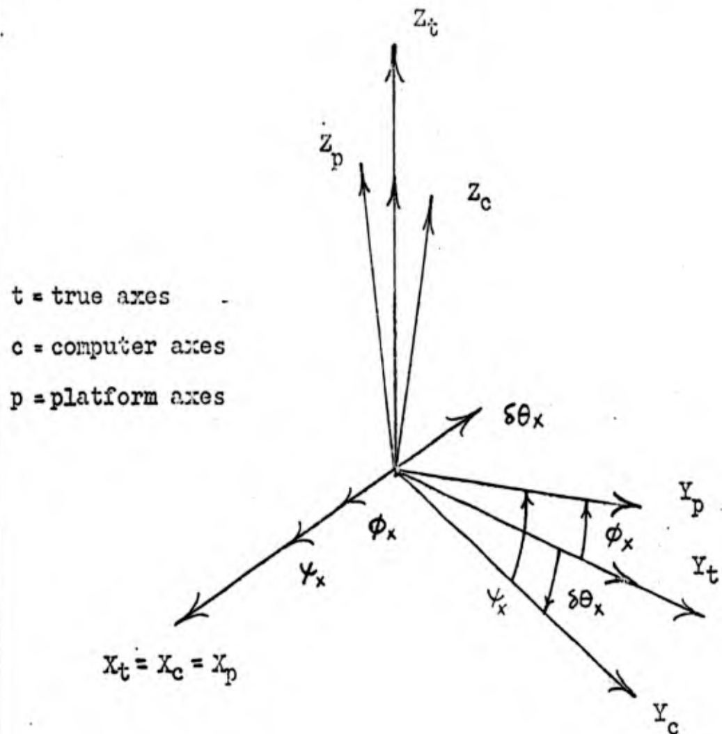
Figure 3 Relationship Between Vector Angles \phi , \delta\theta , and \psi .
