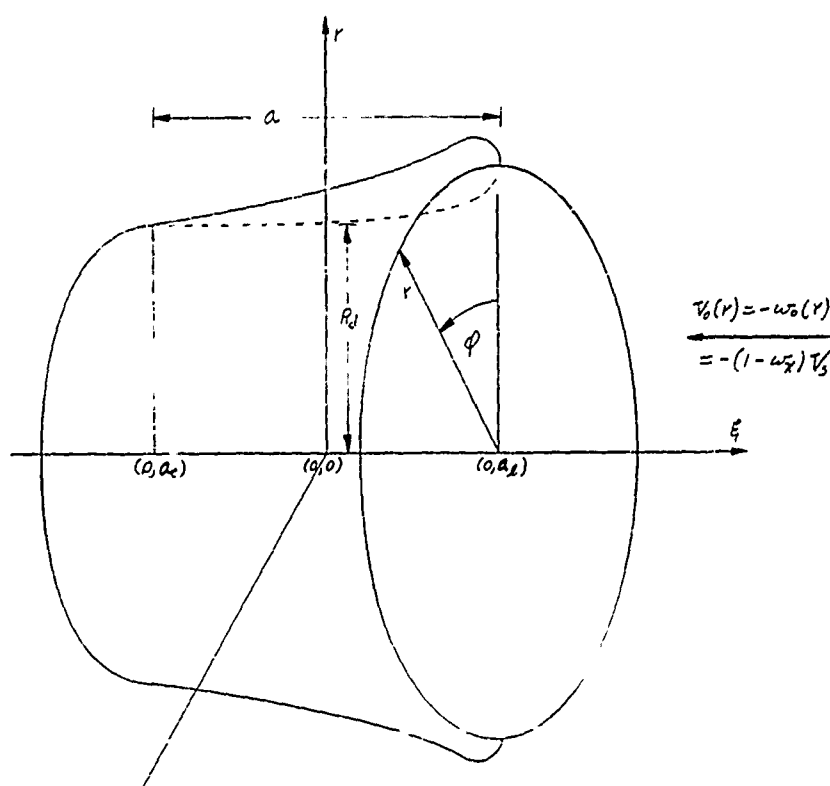
Figure 1. The annular airfoil coordinate system
