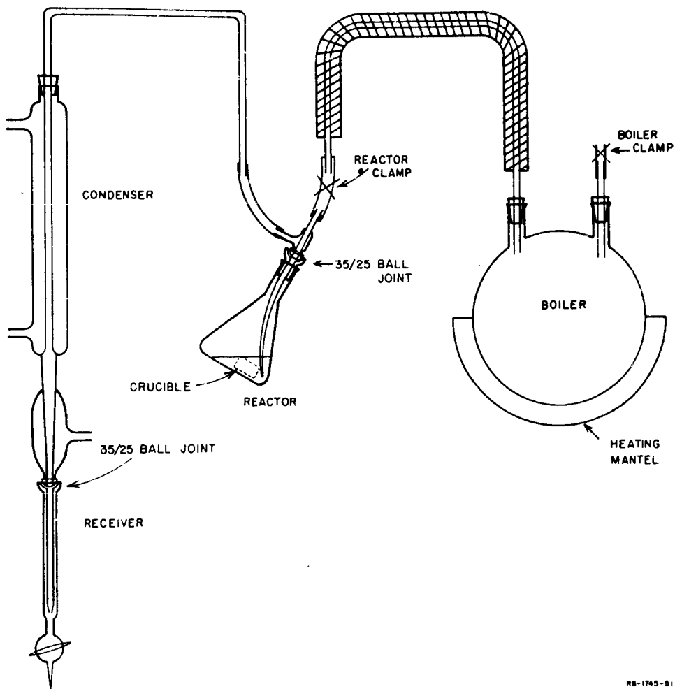
FIG. A-1 APPARATUS FOR DETERMINATION OF N 2 IN Li
