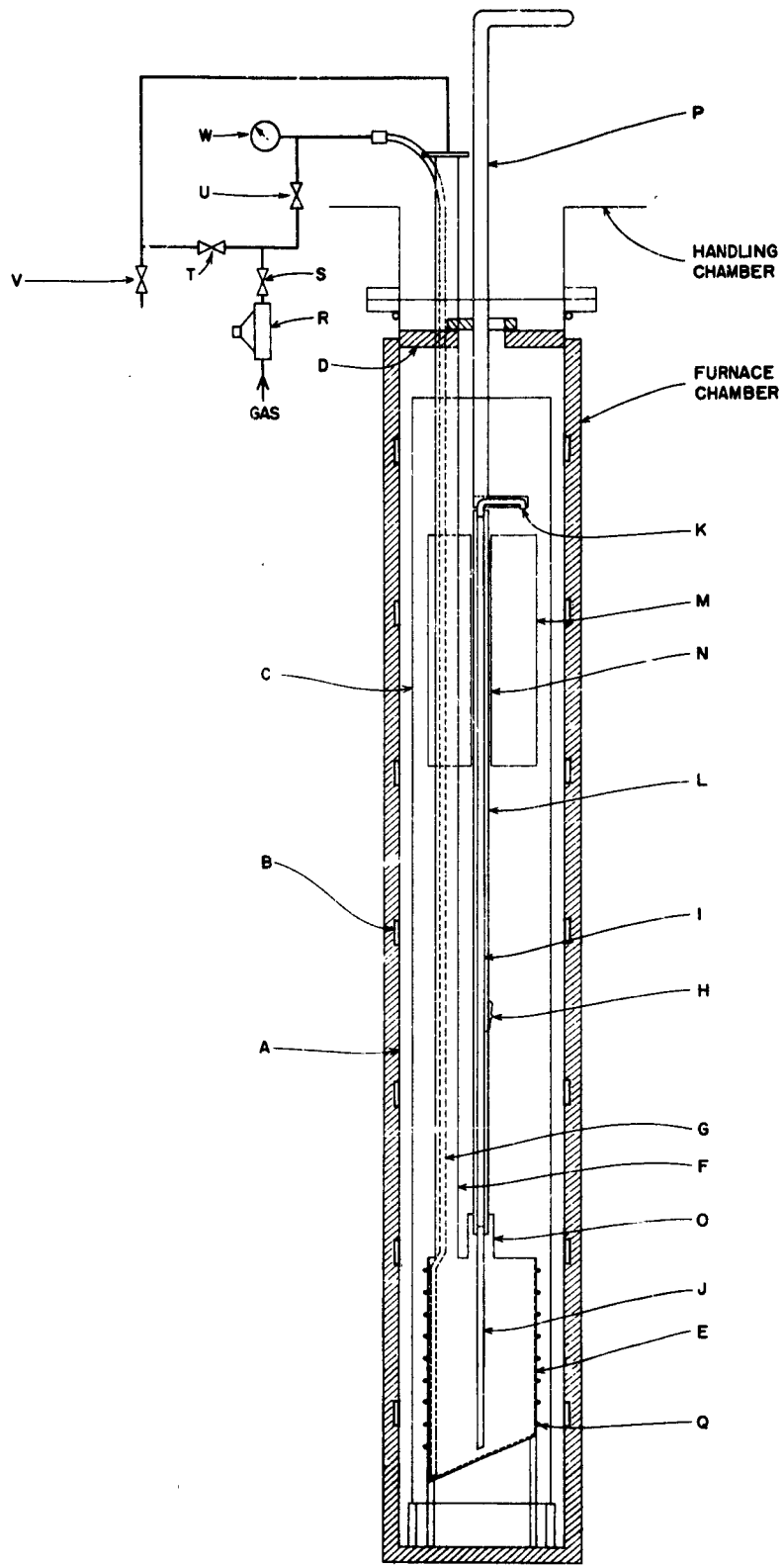
FIG. 3 FURNACE AND TESTING ASSEMBLY
