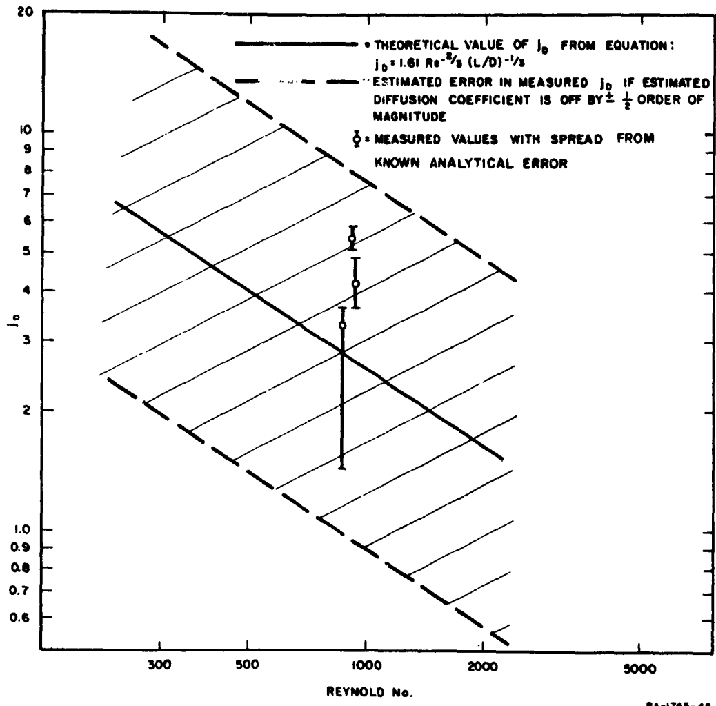
FIG. 6 j FACTOR VS REYNOLDS NUMBER FOR CONDITIONS OF RUN 1
