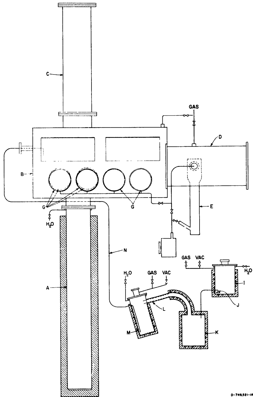
FIG. 2 VACUUM AND INERT ATMOSPHERE CHAMBER FOR HANDLING LITHIUM. LITHIUM PURIFICATION TRAIN
