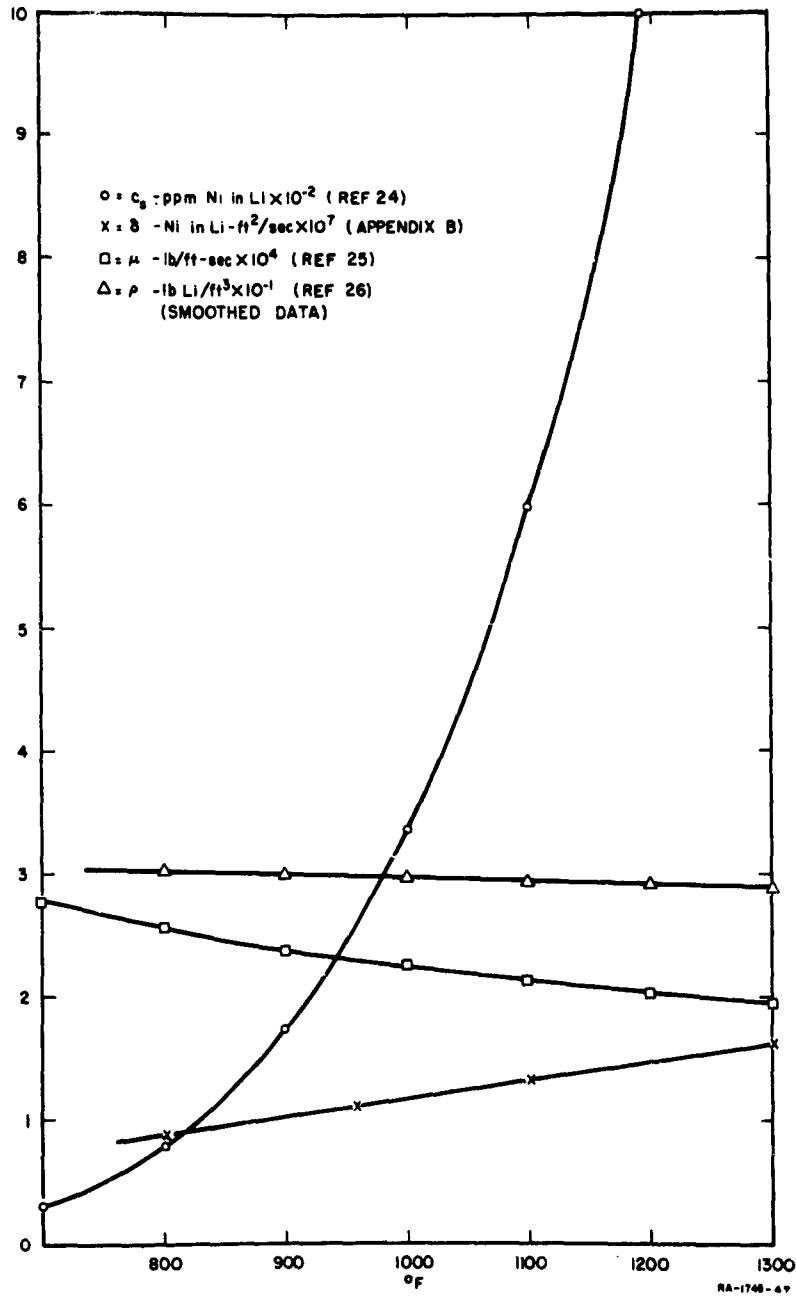
FIG. 5 PHYSICAL PROPERTIES OF LITHIUM
