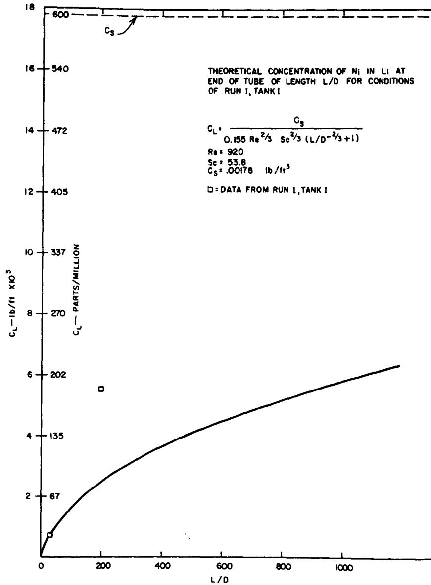
FIG. 8 THEORETICAL CONCENTRATION OF NI IN LI AT END OF TUBE OF LENGTH L/D FOR CONDITIONS OF RUN 1, TANK 1
