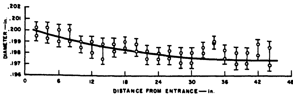
FIG. 7 INSIDE DIAMETER OF NICKEL TUBES AFTER RUNS 1 AND 2
