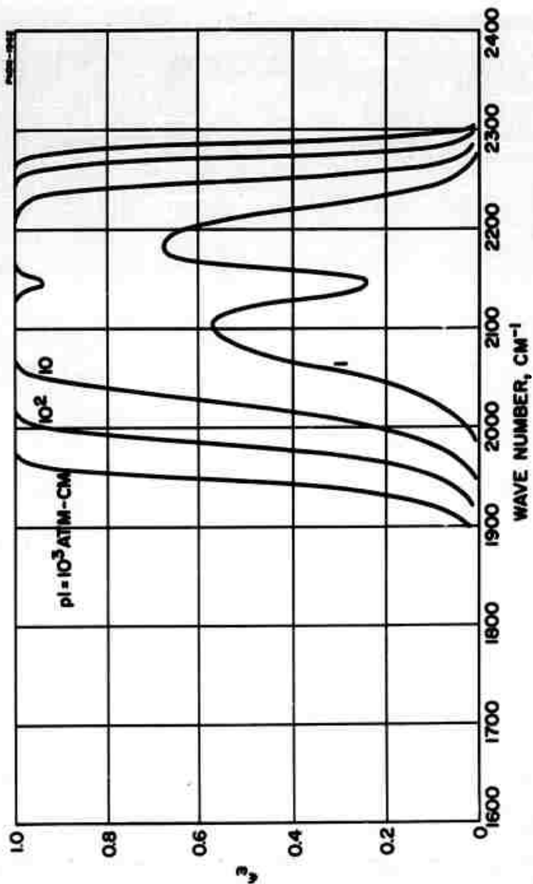
FIGURE 2 SPECTRAL EMISSIVITY OF CO AT T = 600^\circ\text{K} (WEAK LINE APPROXIMATION)
