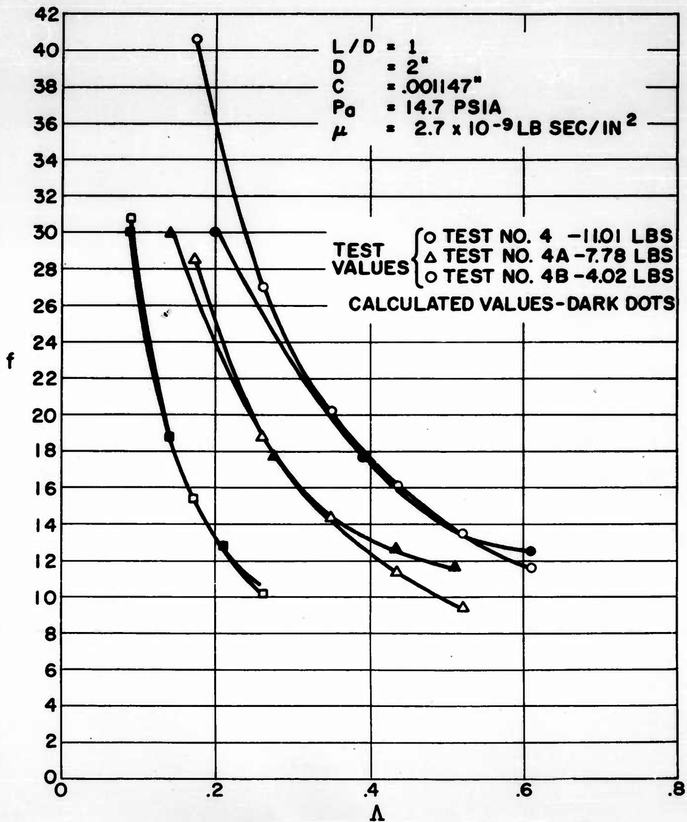
Fig. 13. Plots of \Lambda vs. f .
