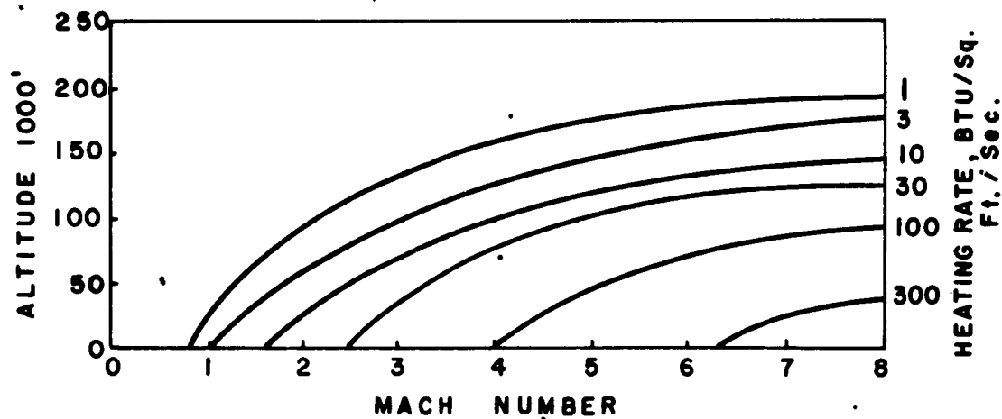
Figure 2 Maximum Heating Rate as a Function of Altitude and Mach Number (After Rowe, 12)
