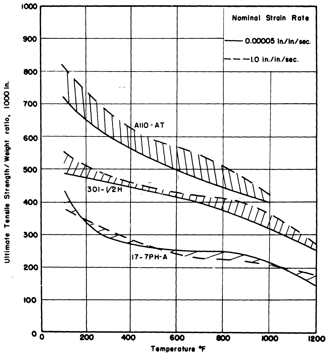
Figure 73 Effect of Temperature After 10-Sec Heating Time and 1800-Sec Holding Time on the Ultimate Tensile Strength of Several Test Metals Over a Range of Strain Rates from 0.00005 to 1.0 in./in./sec. (adapted from WADC TR 55-199 Pt 2).
