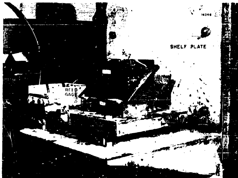
Fig. 9 - Shelf plate with 261-lb load. The instruments are oriented for shock blow.
