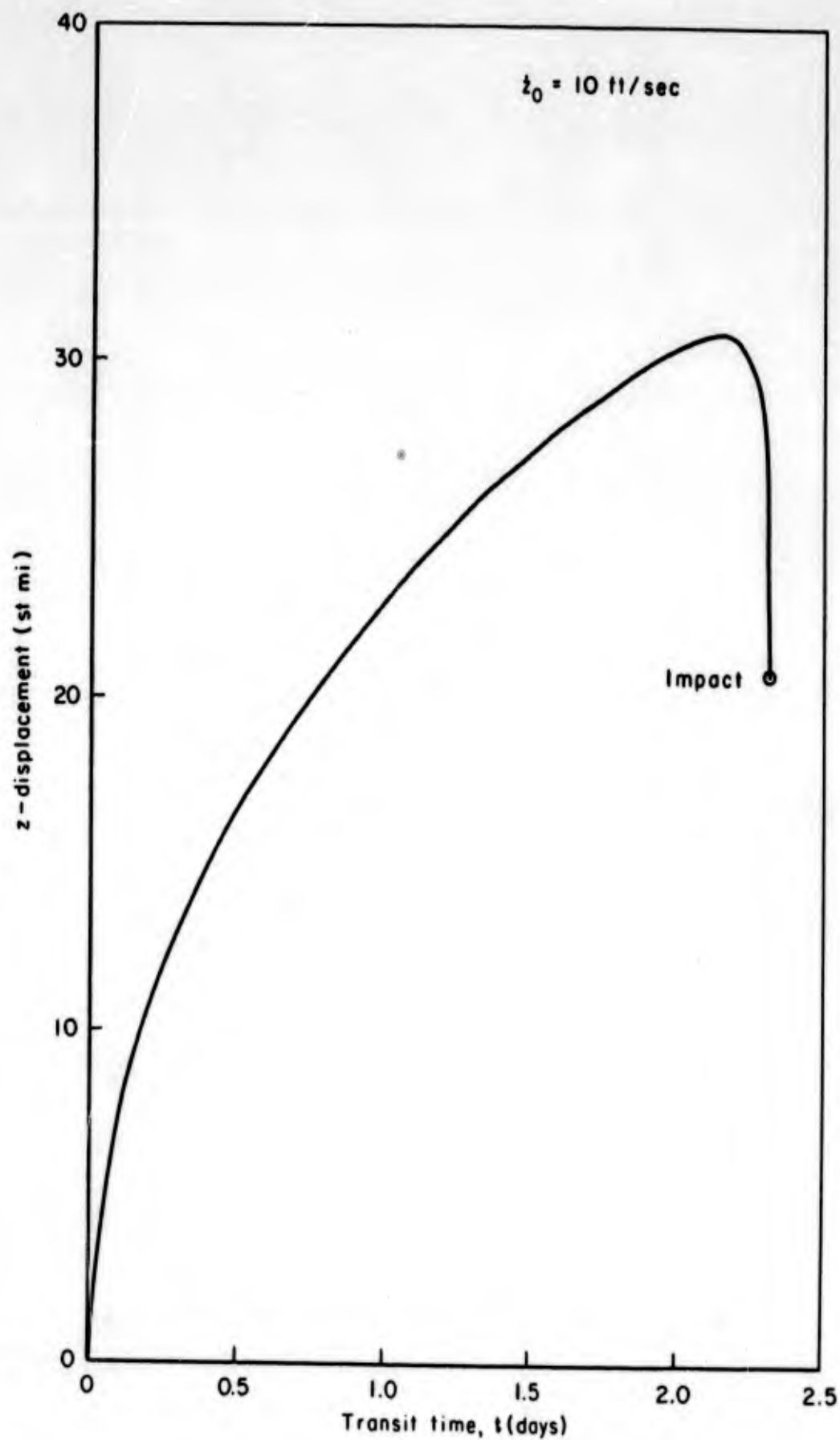
Fig.33 — Out-of-plane displacement (design case)
