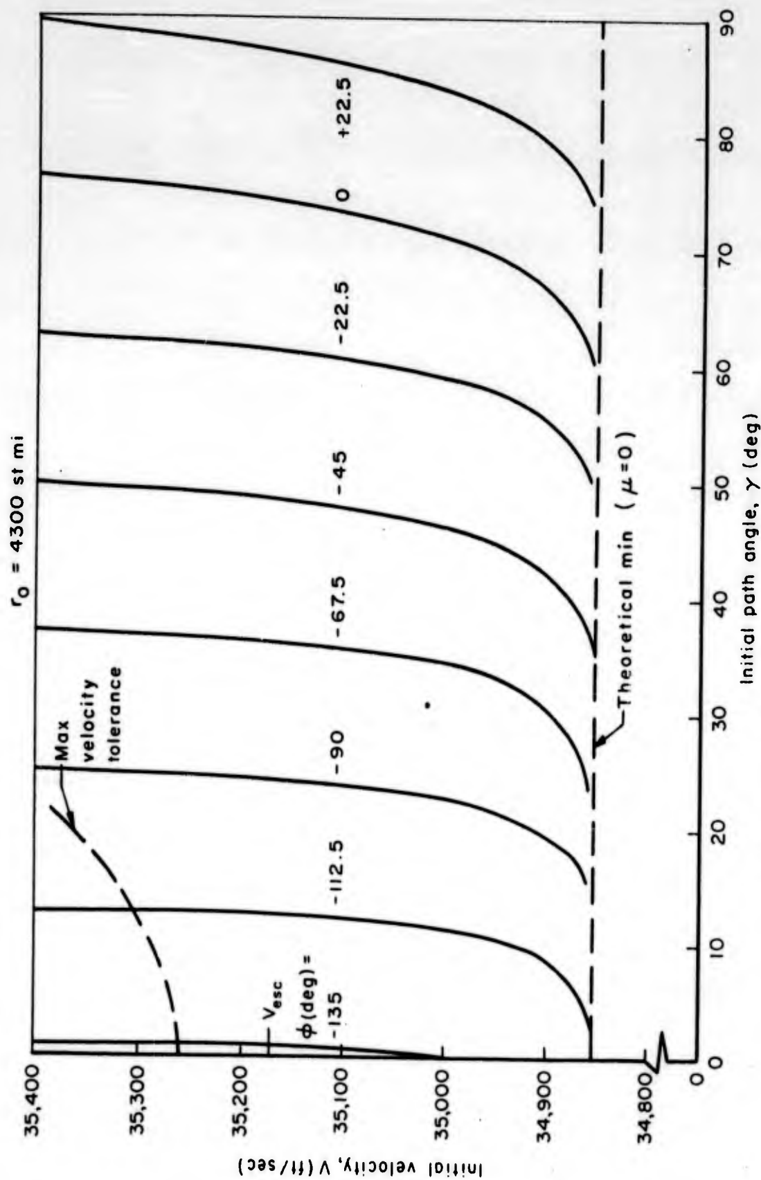
Fig. 5 — Initial conditions — direct motion (inertial system)
