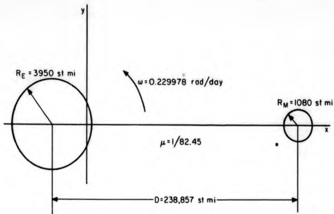
Fig.1—Earth—moon model
