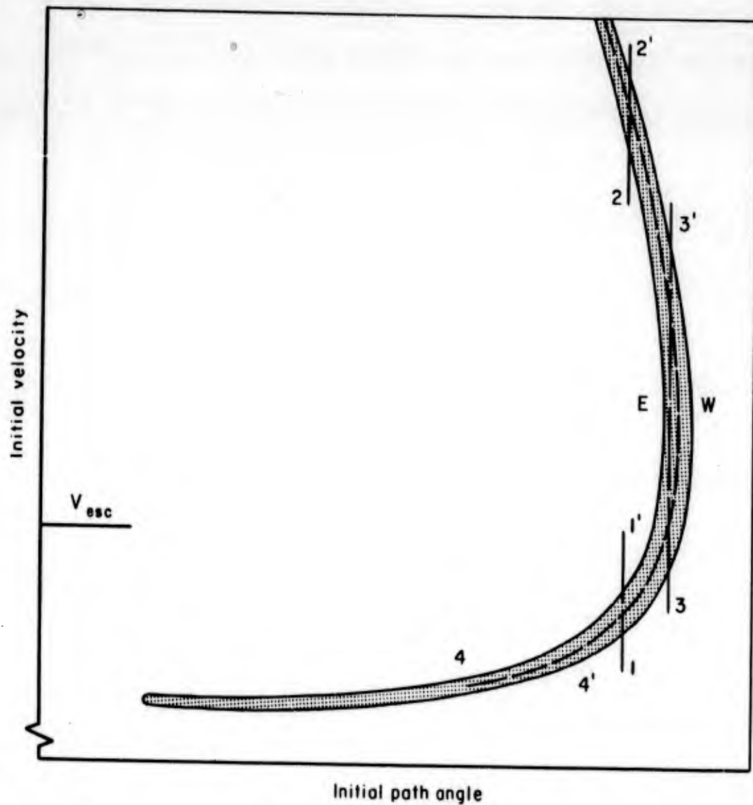
Fig. II — Hit band for a typical initial position at the earth
