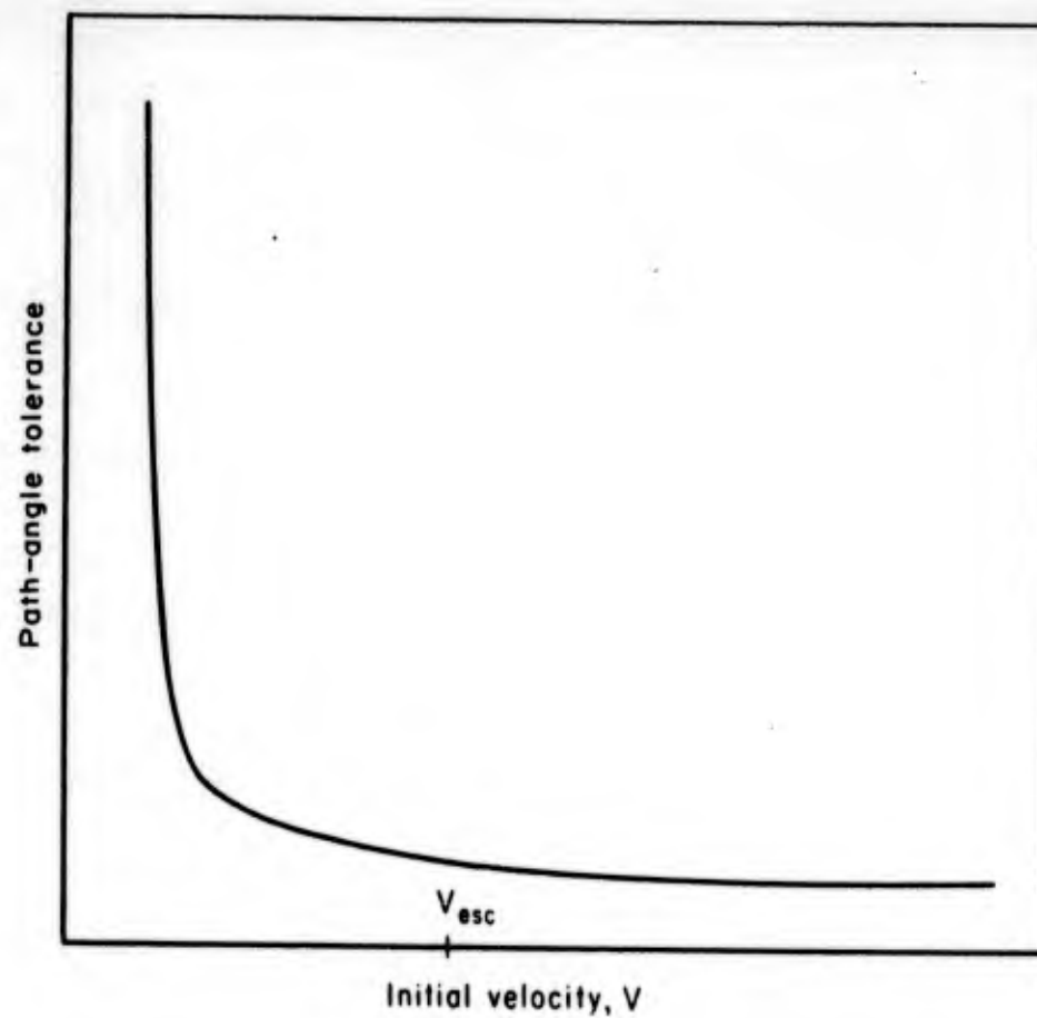
Fig.13— Initial path-angle tolerance as a function of initial velocity
