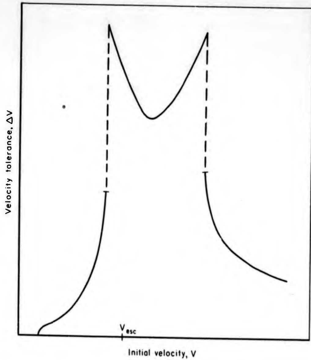
Fig.12 — Initial velocity tolerance as a function of initial velocity
