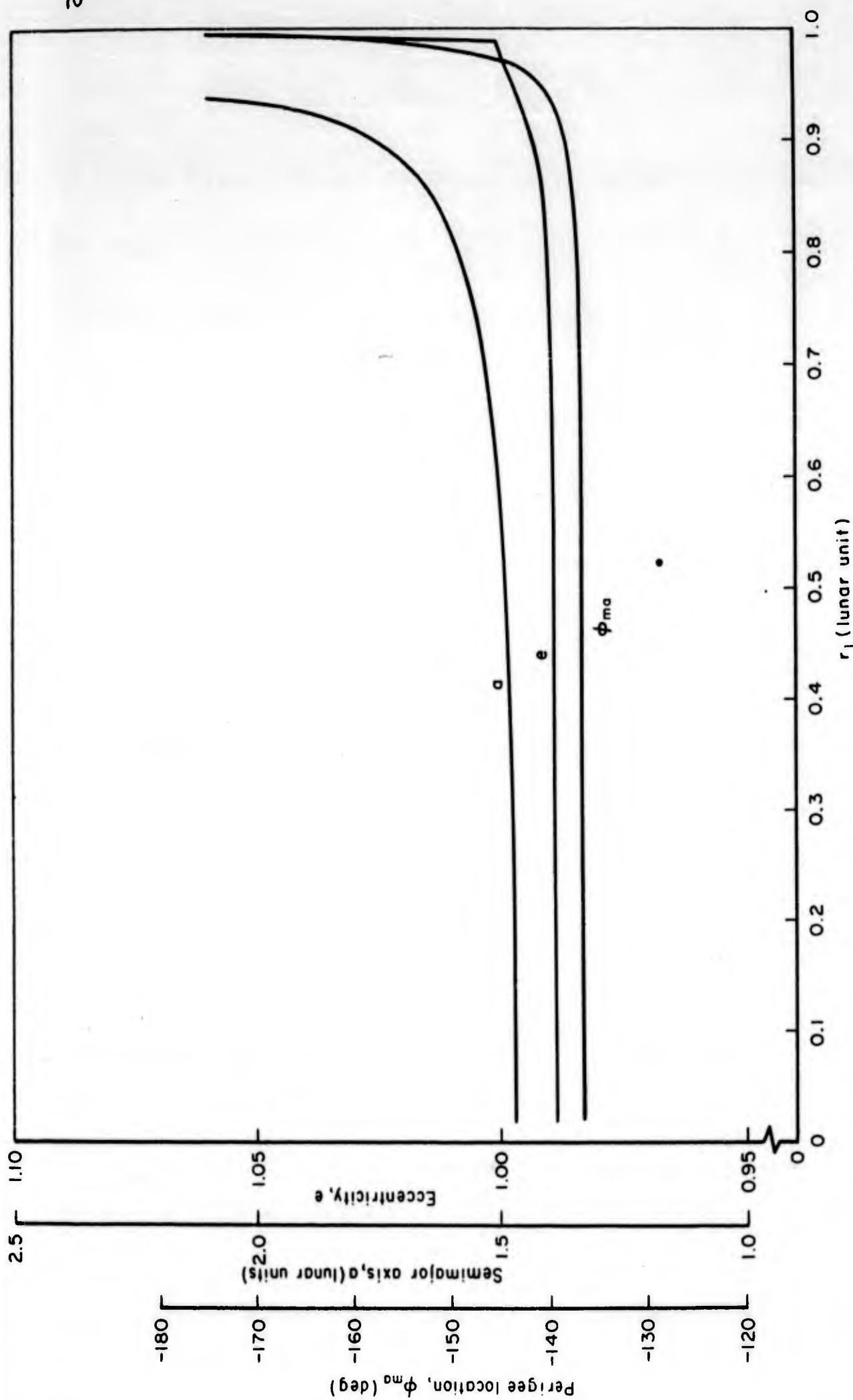
Fig. 29— Instantaneous conic elements relative to the earth (design case)
