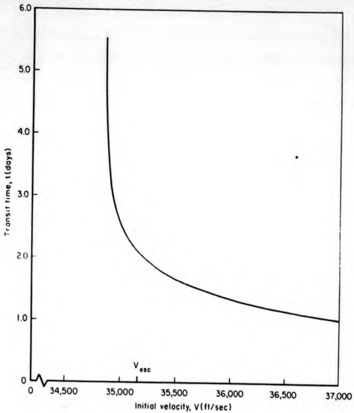
Fig.10—Transit time
