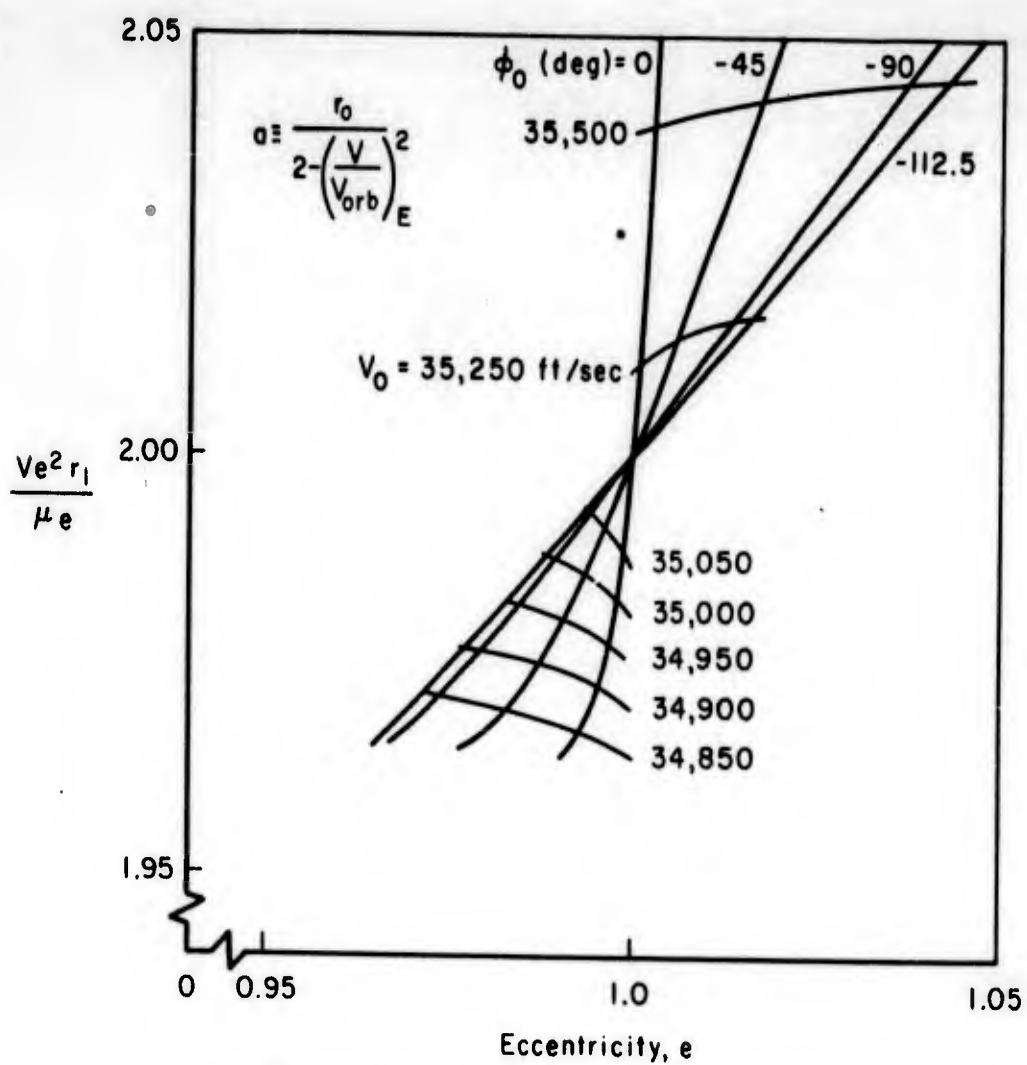
Fig. 7 — Initial conic parameters (direct motion)
