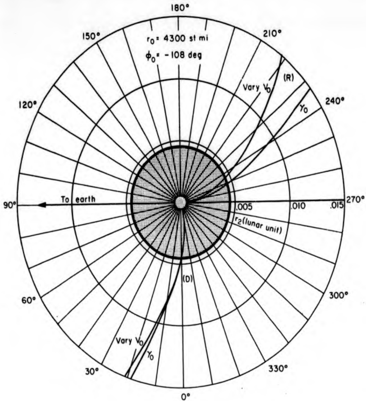
Fig.22 — Perilune position
