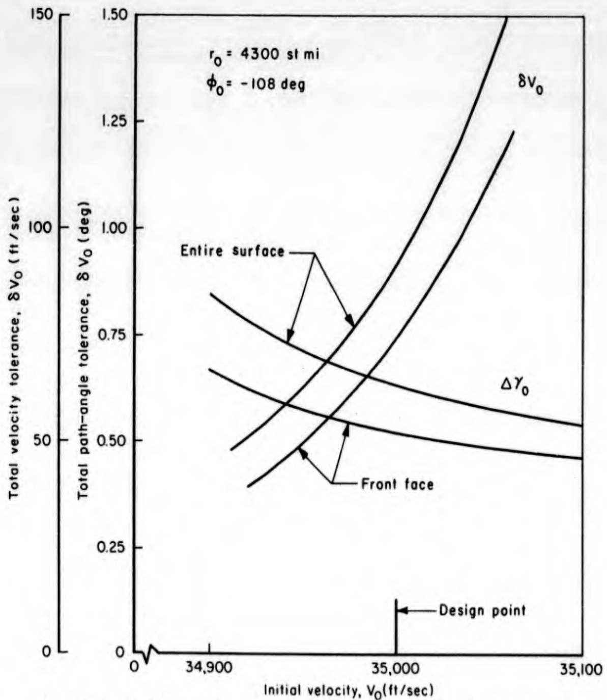
Fig. 17 — Initial tolerances as a function of initial velocity
