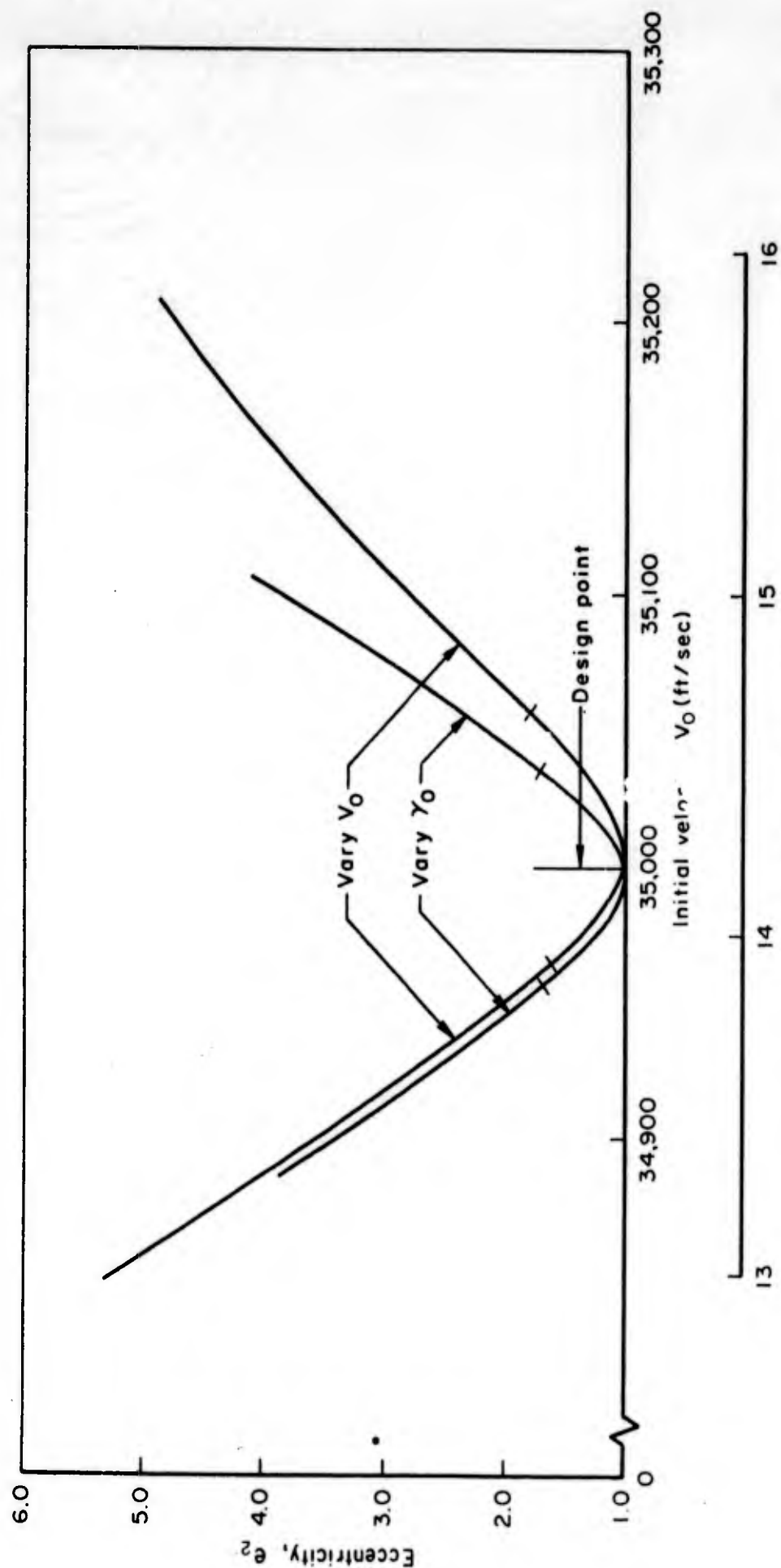
Fig. 20 — Eccentricity relative to the moon
