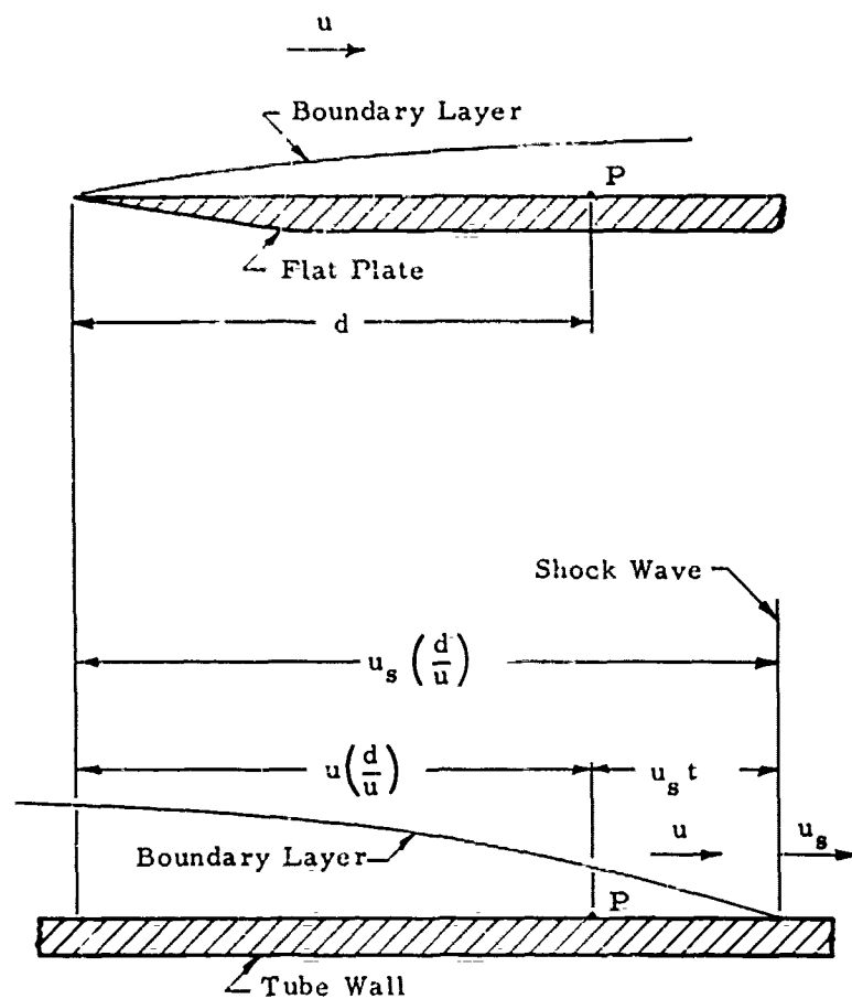
Figure 10. Flat Plate Analogy
