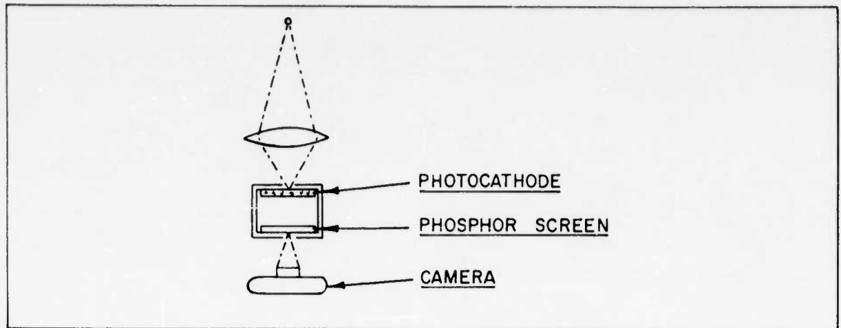
Figure 2a. The Basic Image-Converter System
