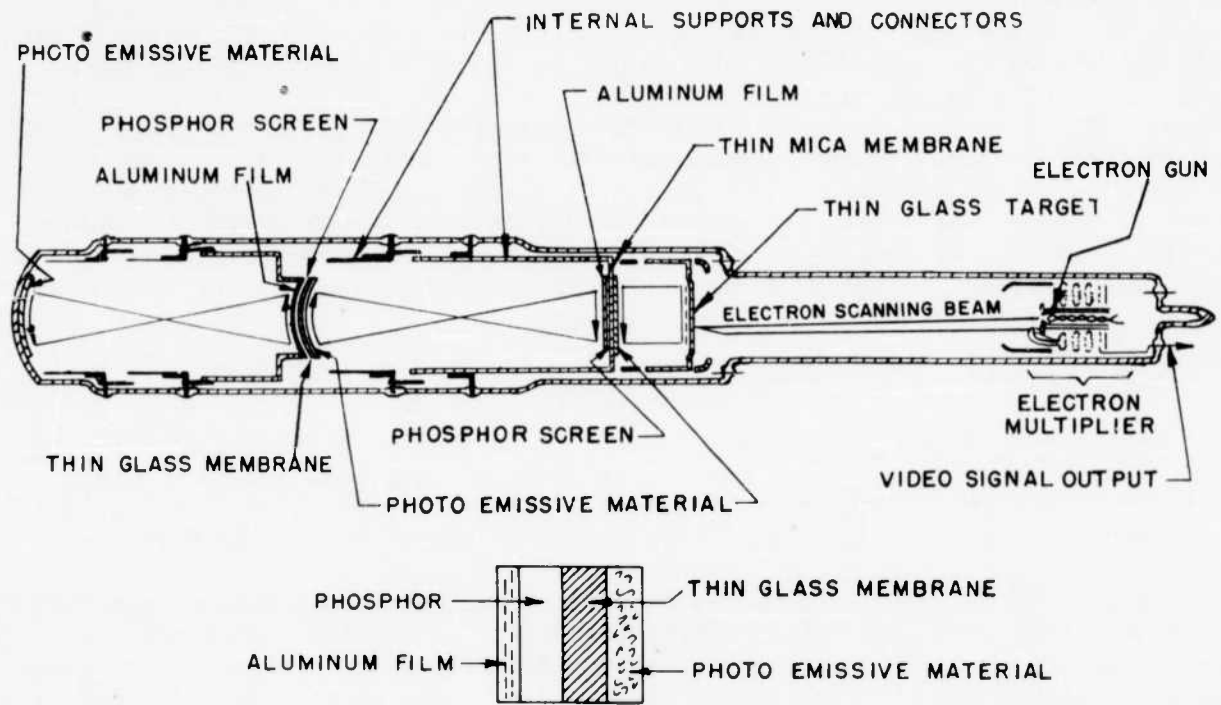
Figure 3c. Two Stage Intensifier Image Orthicon
