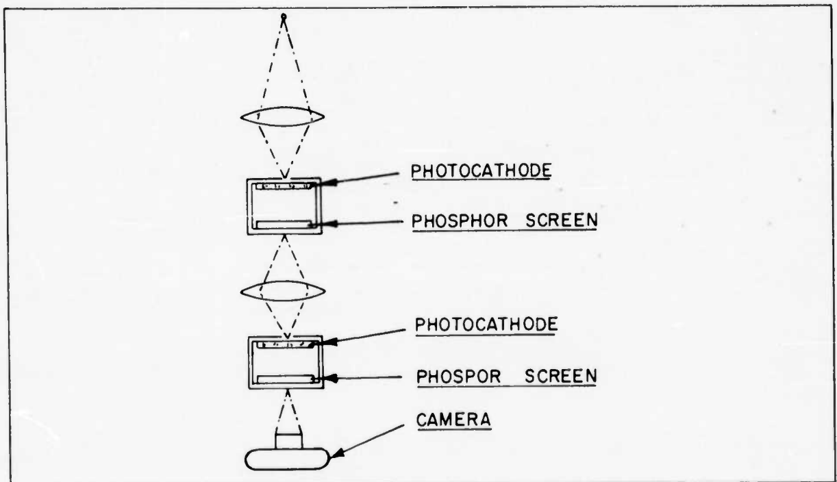
Figure 2b. The Image-Converter System Optically Cascaded
