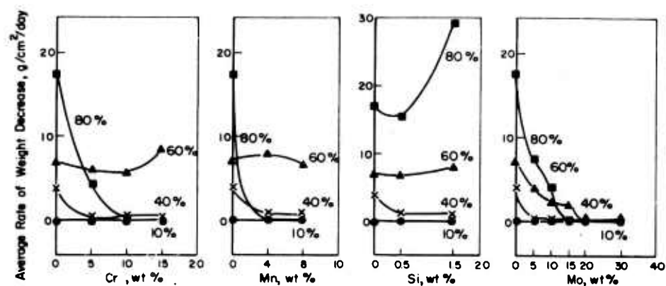
a. In Various Concentrations of H 2 SO 4 at Boiling Temperature
