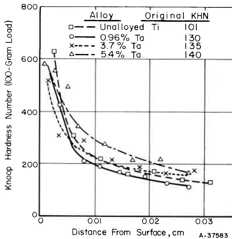
FIGURE 18. HARDNESS-CONTAMINATION CURVES IN TITANIUM-TANTALUM ALLOYS EXPOSED 6 HOURS AT 900 C (1652 F) IN STILL AIR (2)
