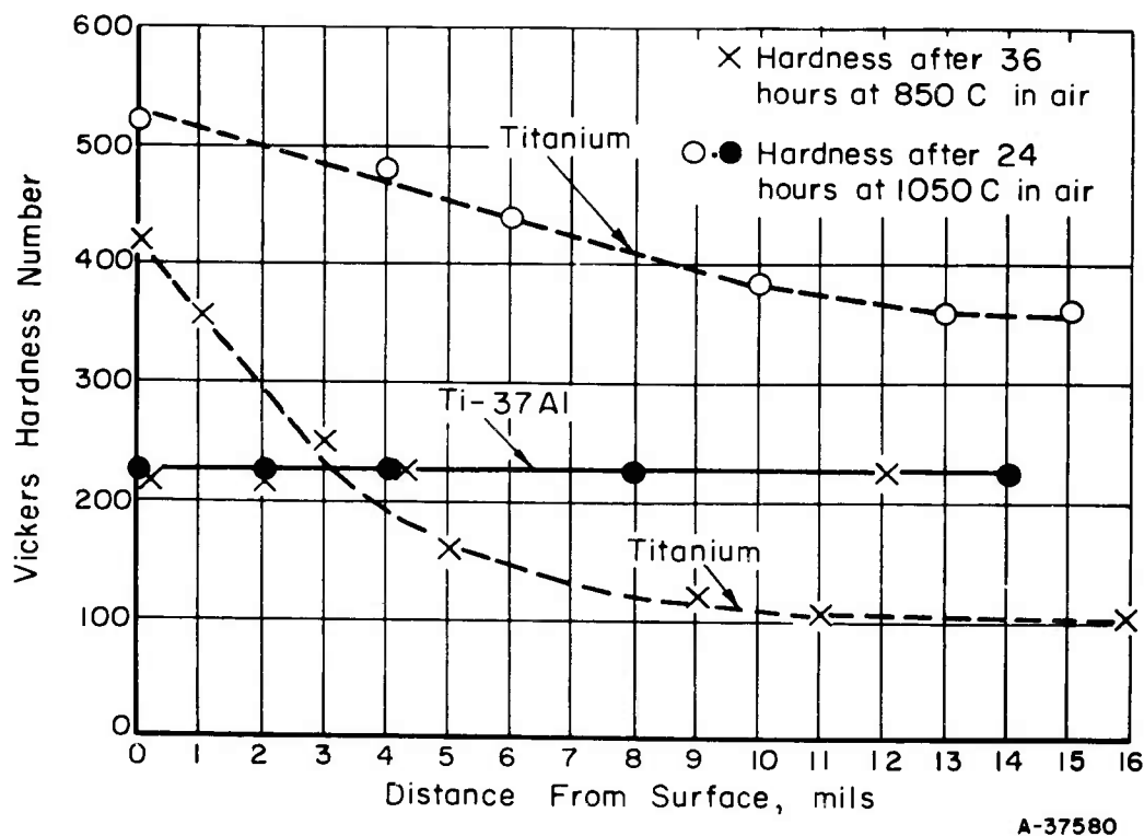
FIGURE 15. HARDNESS DATA FOR A GAMMA-PHASE IODIDE TITANIUM-37 PER CENT ALUMINUM ALLOY (45)
