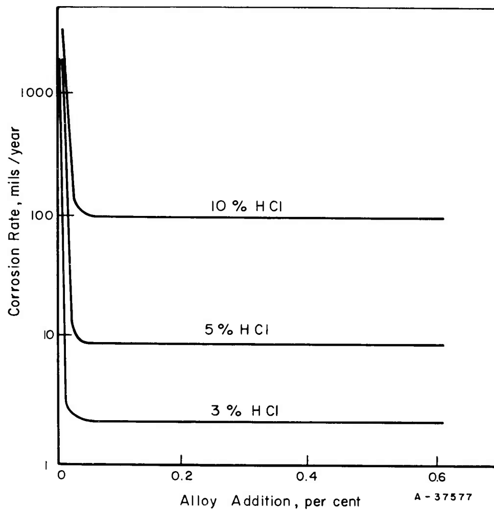
FIGURE 12. EFFECT OF PLATINUM AND PALLADIUM ADDITIONS ON CORROSION RATE OF TITANIUM IN BOILING HYDROCHLORIC ACID SOLUTIONS (37)
