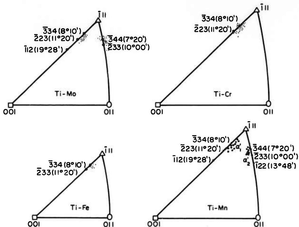
FIGURE 57. LOCATION OF POLES OF MARTENSITE HABIT PLANES IN TITANIUM-MANGANESE (150) , TITANIUM-MOLYBDENUM (148) , TITANIUM-IRON (148) , AND TITANIUM-CHROMIUM (148) ALLOYS IN STEREOGRAPHIC TRIANGLES
