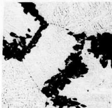
750X 6859 a. 5 minutes (10HF-60HNO 3 -30 glycerine)
