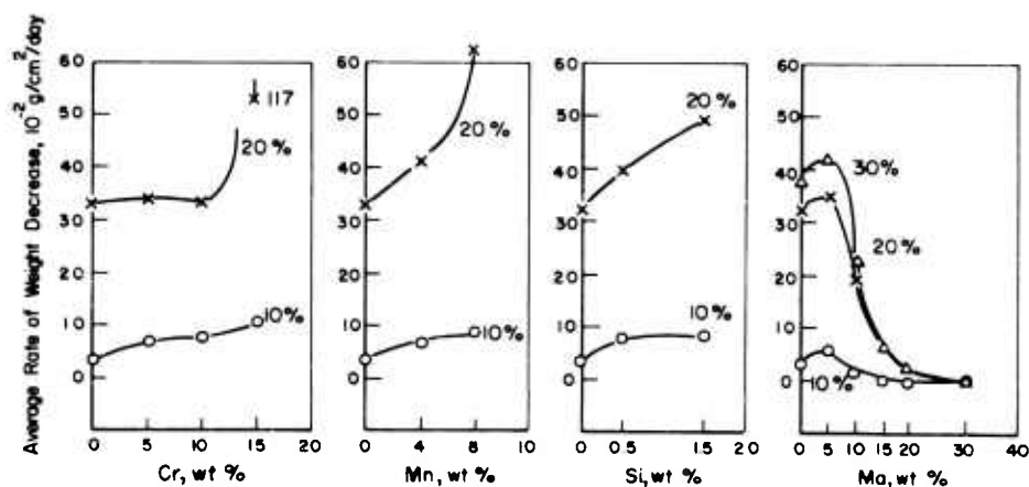
b. In HCl at Boiling Temperature
