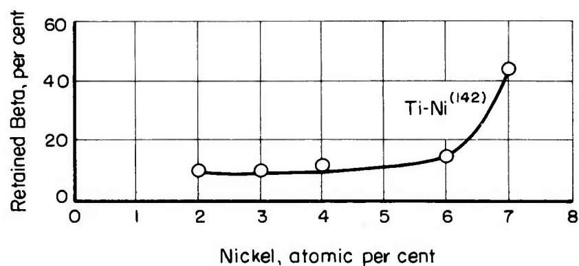
FIGURE 55. EFFECT OF ALLOY COMPOSITION ON THE COMPLETION OF THE BETA-TO-ALPHA PRIME TRANSFORMATION
