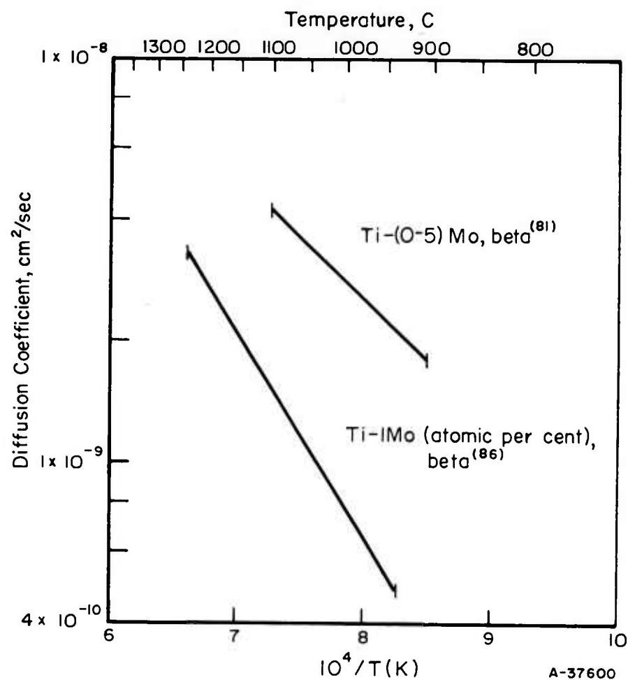
FIGURE 35. EFFECT OF TEMPERATURE ON THE DIFFUSION OF MOLYBDENUM IN DILUTE TITANIUM-MOLYBDENUM ALLOYS
