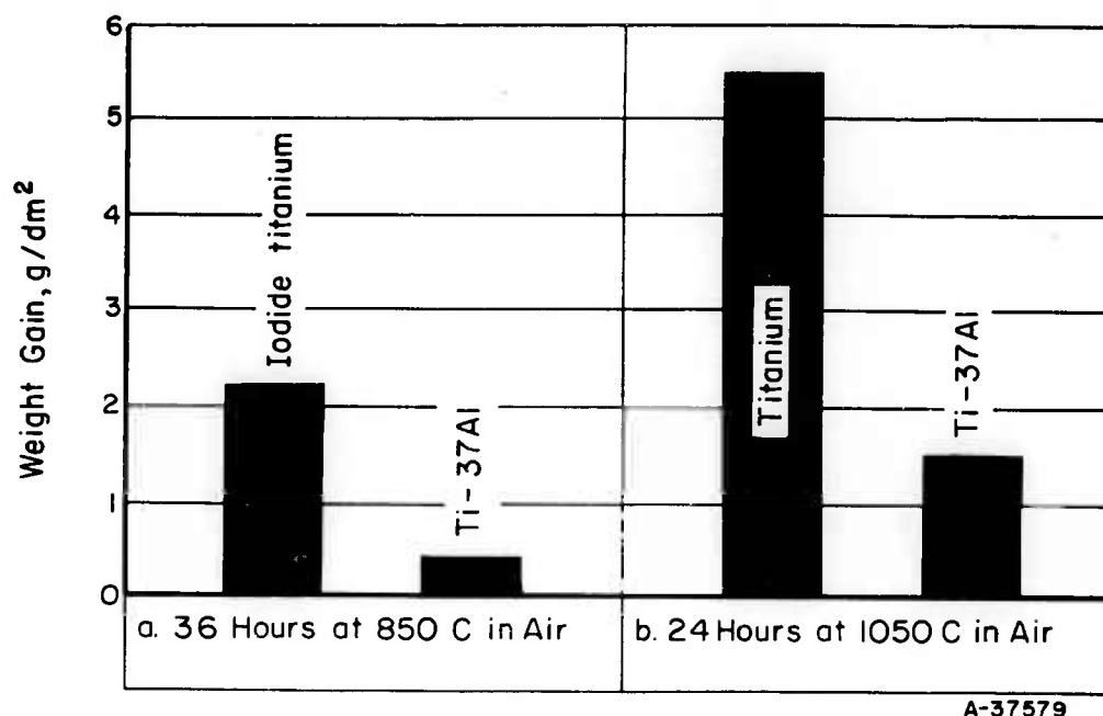
FIGURE 14. WEIGHT-GAIN DATA FOR A GAMMA-PHASE IODIDE TITANIUM-37 PER CENT ALUMINUM ALLOY (45)
