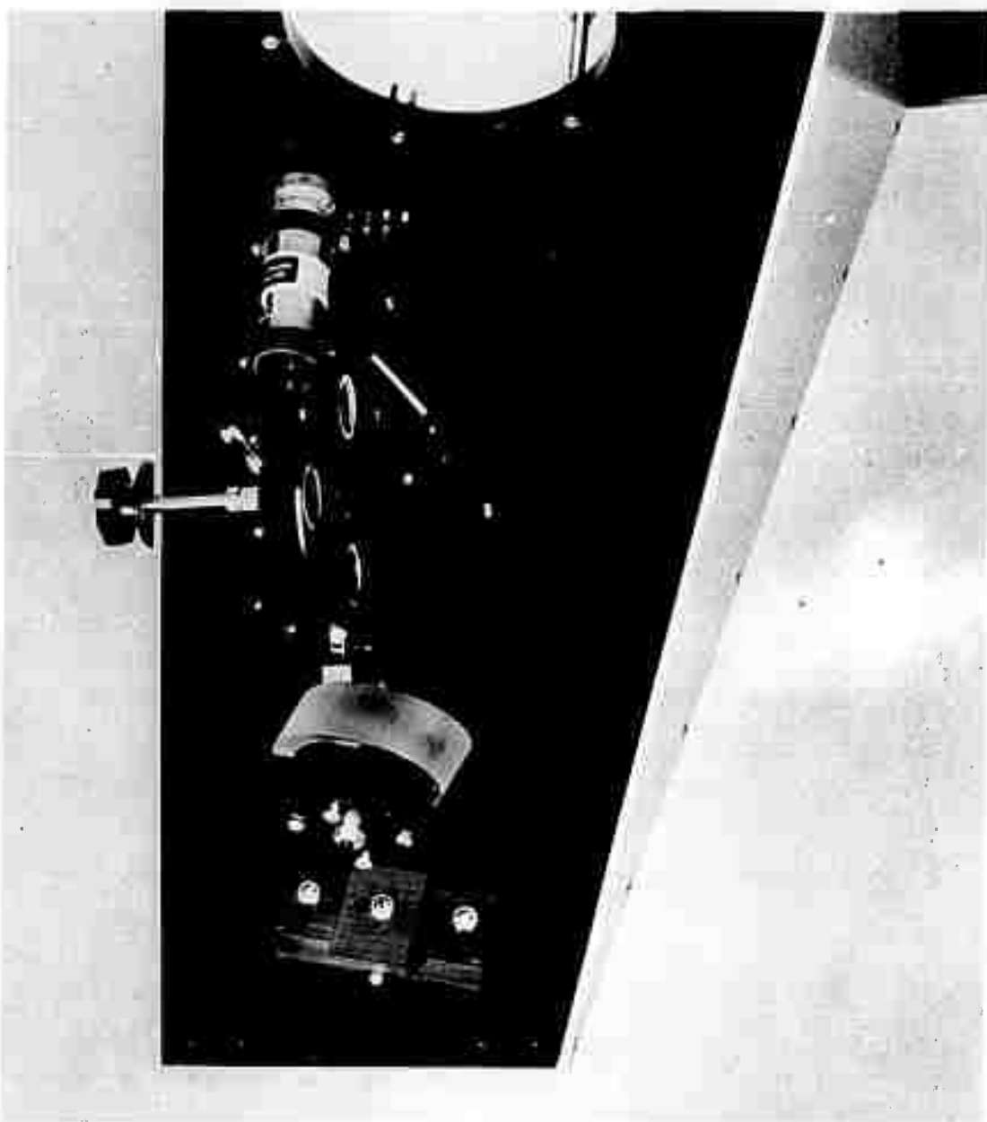
Figure 9. CLOSEUP OF DETECTOR SECTION OF PHOTOMETER HEAD
