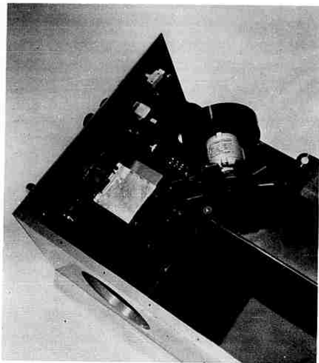
Figure 5. TWO MIRROR CHOPPING SYSTEM AND REFERENCE BLACKBODY
