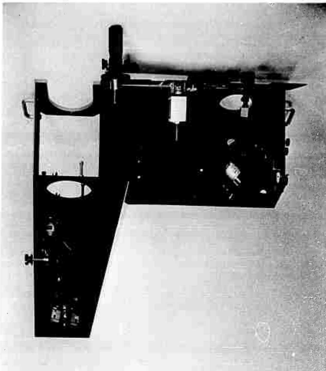
Figure 7. PHOTOMETER HEAD WITH FRONT PANEL TIPPED BACK
