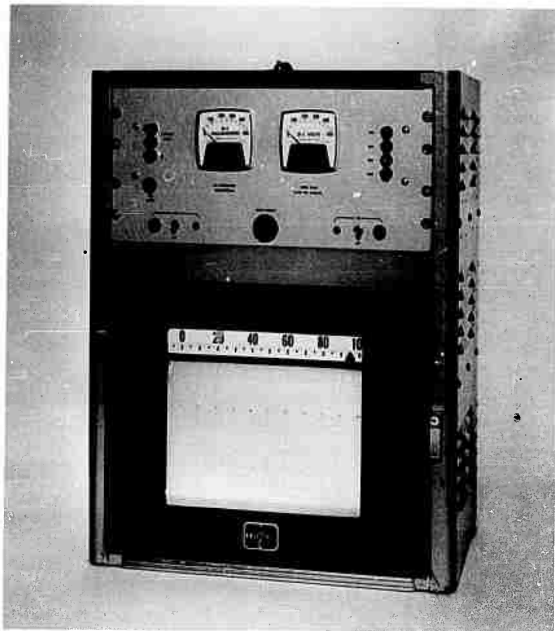
Figure 11. RECORDER RACK
