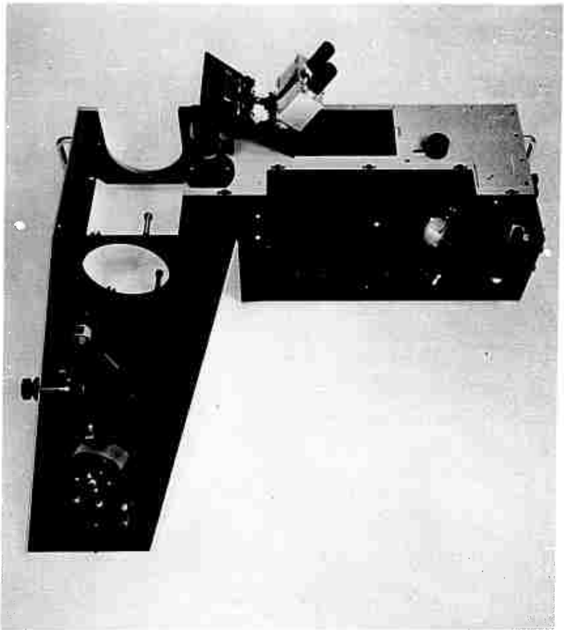
Figure 12. PHOTOMETER HEAD SHOWING PREAMPLIFIERS
