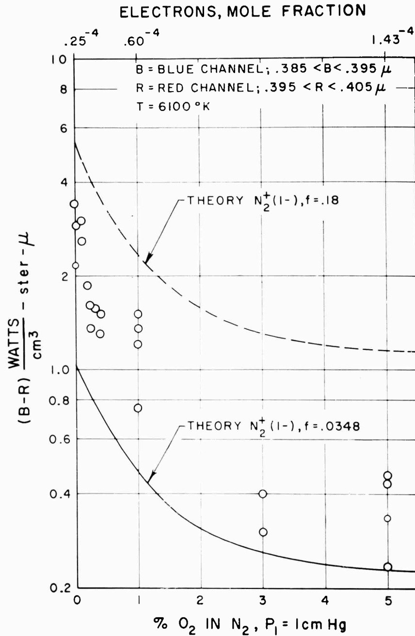
Fig. 6 Intensity difference across 3914 N_2^+(1-) band head versus oxygen contamination. The two theoretical lines are based upon the f-number reported by Keck et al 1 (.18) and Bennet and Dalby 2 (.0348). The depressing effect on the N_2^+ radiation by excess electrons is demonstrated here since NO readily dissociates to NO^+ and e^- .
