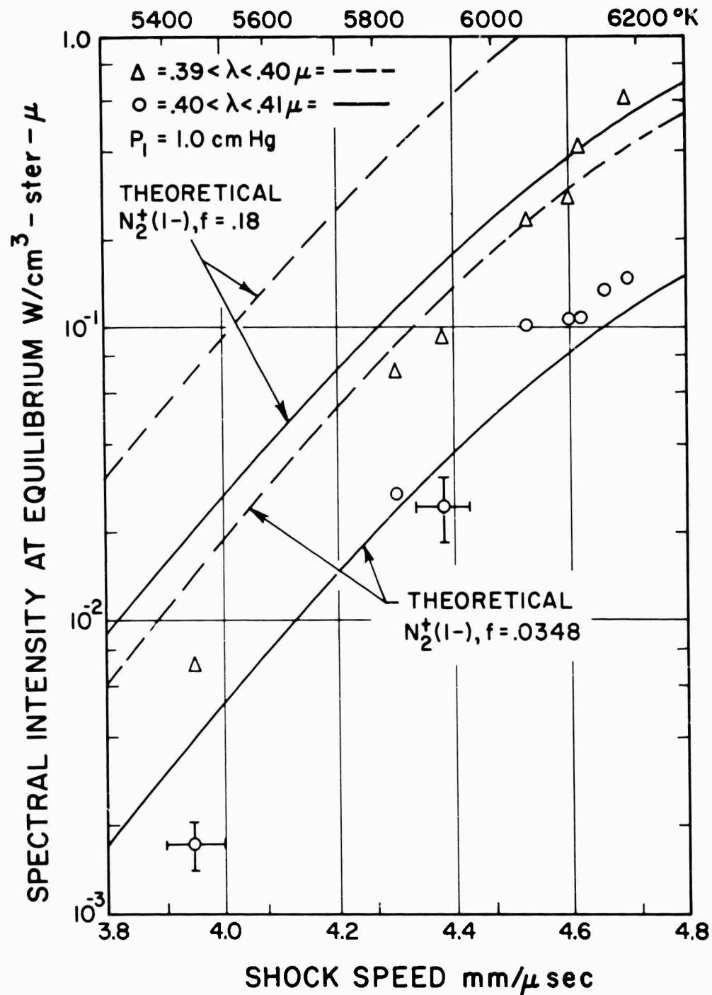
Fig. 5 Intensity of two adjacent monochromator channels versus shock speed in the N_2^+(1-) region comparing experimental observations with theoretical predictions based on the f-number of the N_2^+(1-) system reported by Keck et al 1 (.18) and Bennet and Dalby 5 (.0348).
