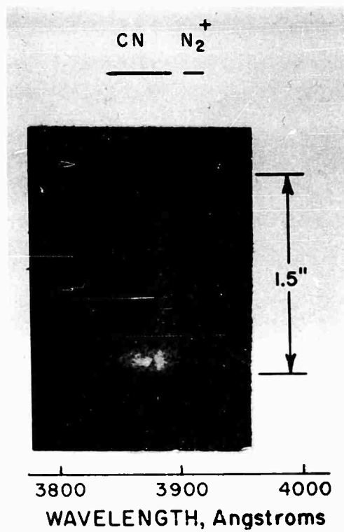
Fig. 3 Spectrogram obtained with slit of spectrograph perpendicular to axis of shock tube driver passage of a 5.1 mm/ \mu sec shock through nitrogen at a pressure of 1 cm Hg. The CN radiation is confined mainly to the shock tube walls.
