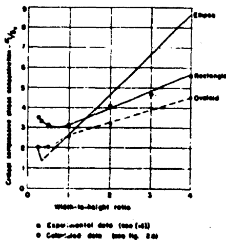
Figure 2.8. Critical compressive stress concentration for tunnels of various cross sections, two-directional stress field. S_h = 1/3 S_0
