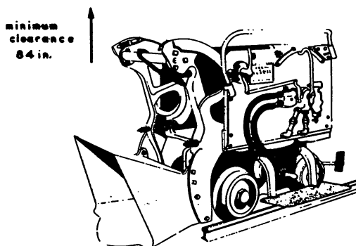
Figure 3.6. Common sizes, up-and-over loaders
