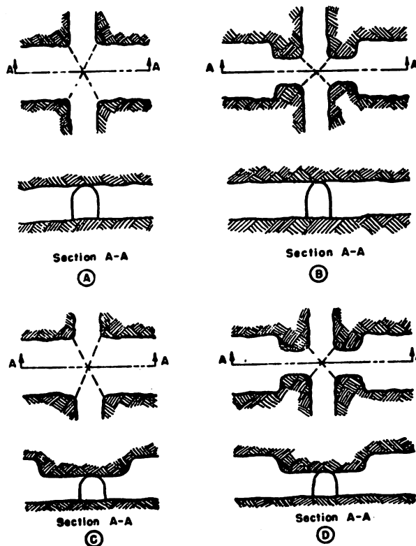
Figure 3.1. Tunnel intersections
