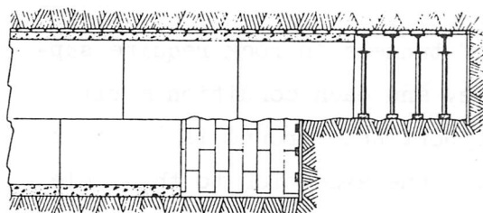
Figure 3.19. Flying arch method
