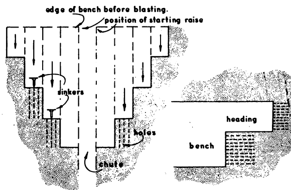
Figure 3.20. Benching
