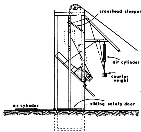
Figure 3.26. Shaft head frame and dumping arrangement
