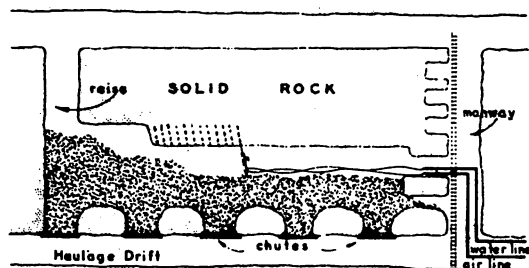
Figure 3.21. Shrinkage method
