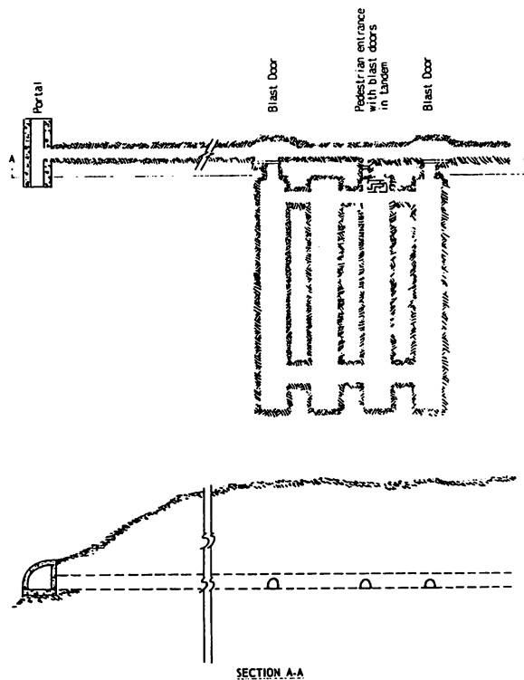
Figure 3.3. Example of entrance layout
