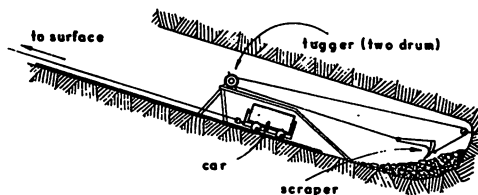
Figure 3.27. Incline showing slusher, ramp, car, and hoist
