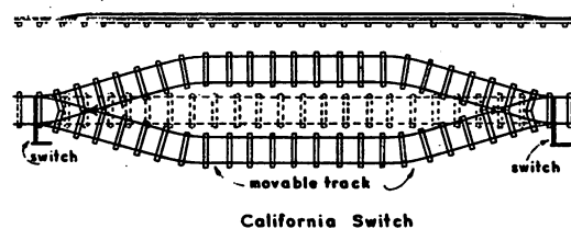
Figure 3.8. Car transfers
