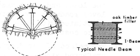
Figure 3.18. Needle beam method
