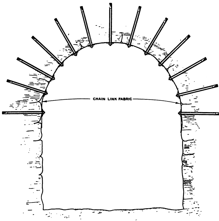
Figure 3.10. Rock bolt pattern
