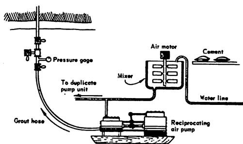
Figure 3.12. Grout machine
