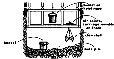
Figure 3.24. Shaft mucker
