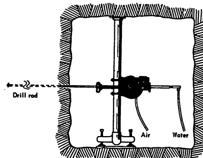
Figure 3.13. Diamond drill
