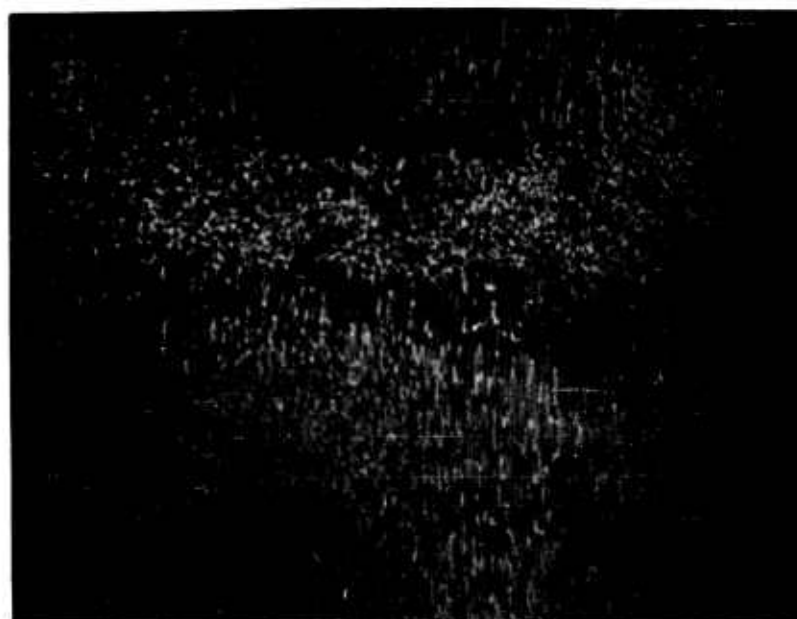
Stress Cracks at 163,000 psi Hoop Stress at Girth Weld. X 2
