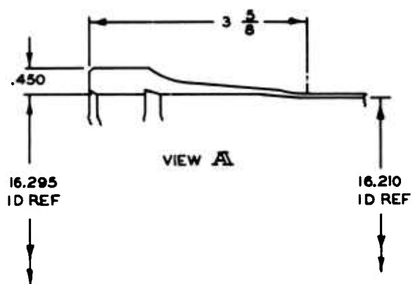
Figure 1. Hydrosun Case Design
